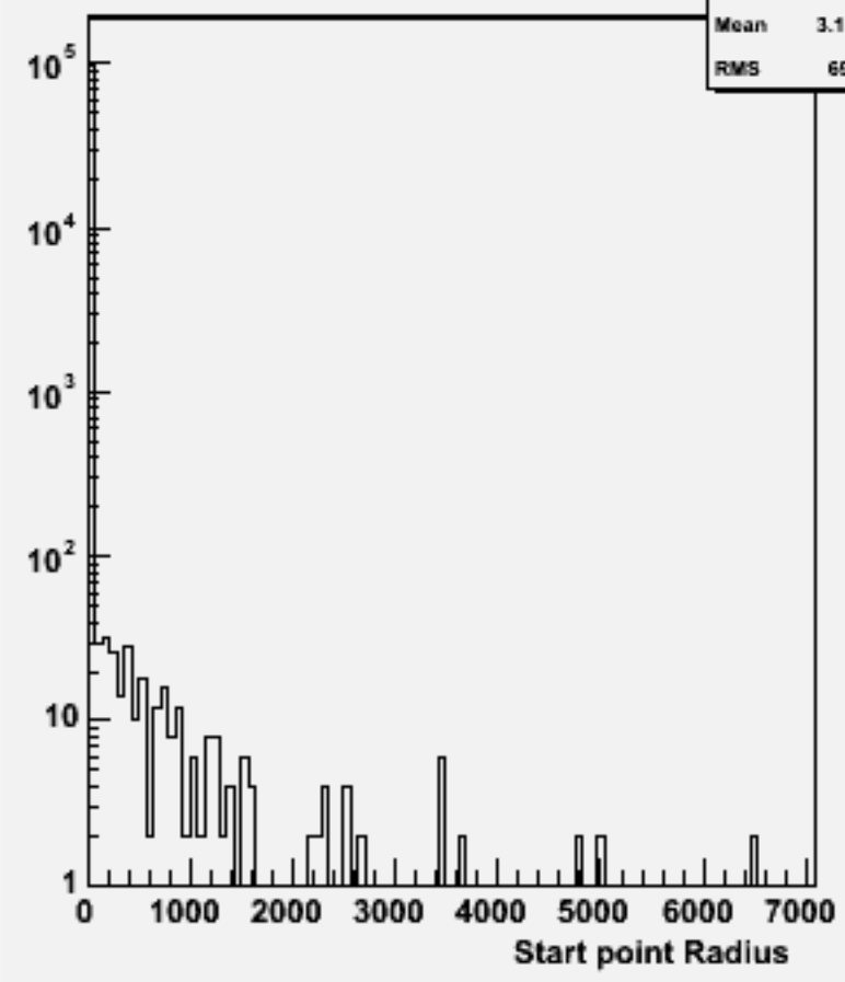
Start point R : w103674 ae1_e1n2e2e3n3_o
