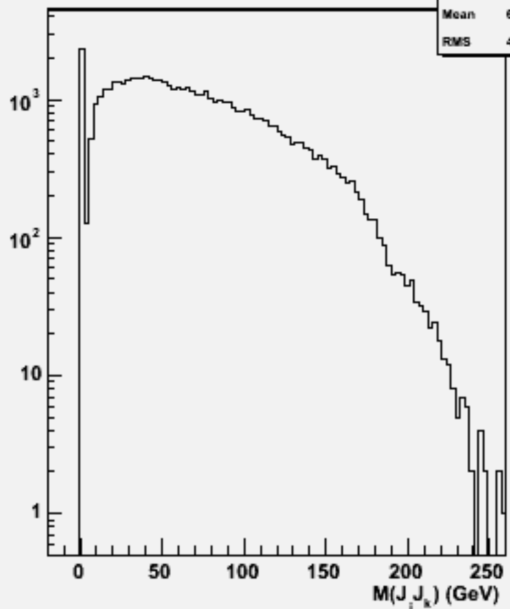
2jets mass(All comb)w103674 ae1_e1n2e2e3n3_o
