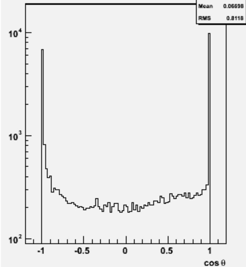
Jet cos theta (All jets)w103674 ae1_e1n2e2e3n3_o
