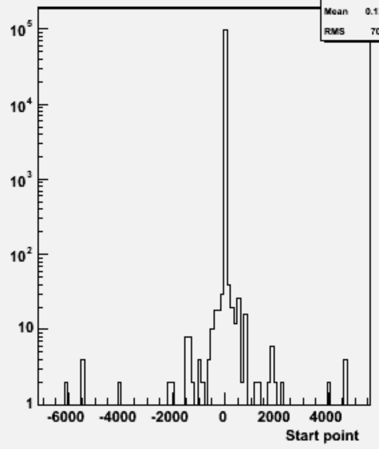
Start point Z : w103674 ae1_e1n2e2e3n3_o
