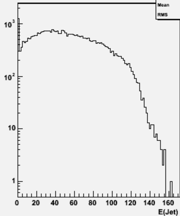
Jet energies(All jets)w103674 ae1_e1n2e2e3n3_o
