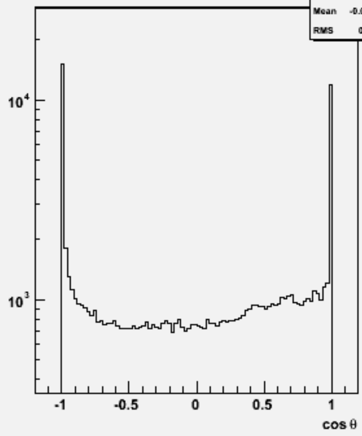
Particle cos \theta : w103674 ae1_e1n2e2e3n3_o
