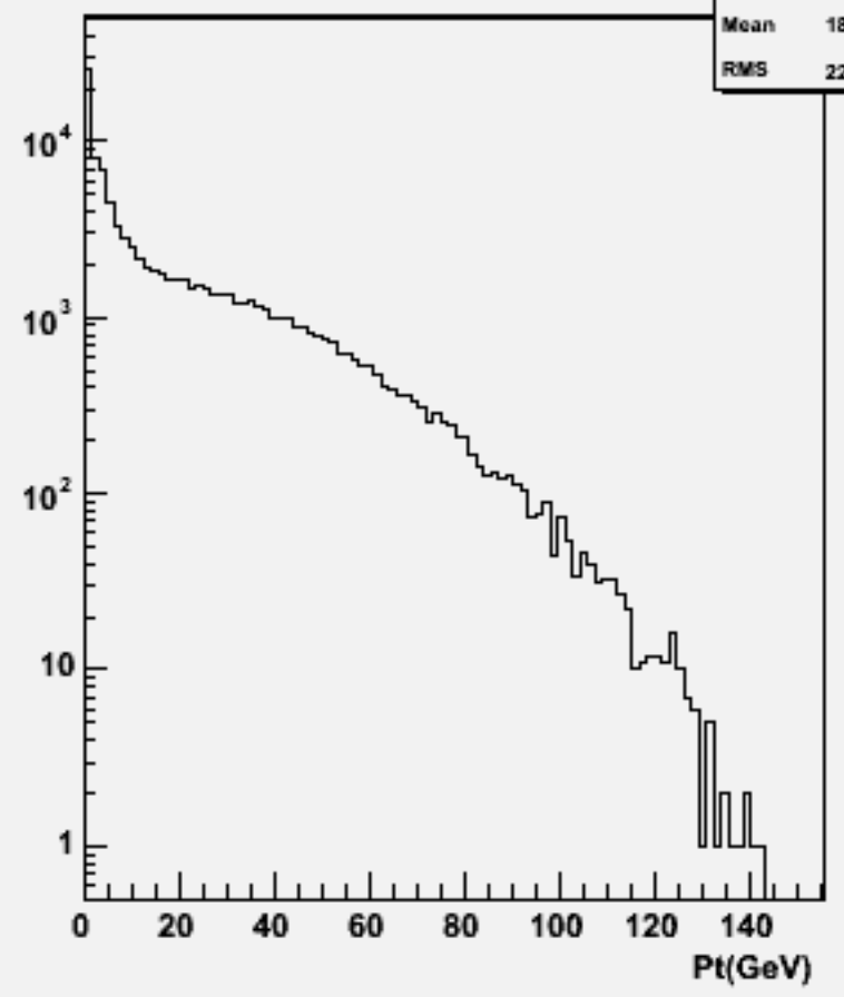
Start point Z : w103672 ae1_e1n2e2e3n3_o
