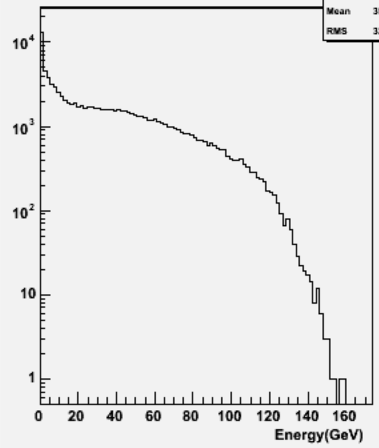
Start point R : w103672 ae1_e1n2e2e3n3_o
