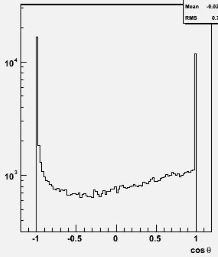
Particle cos θ : w103672 ae1_e1n2e2e3n3_o
