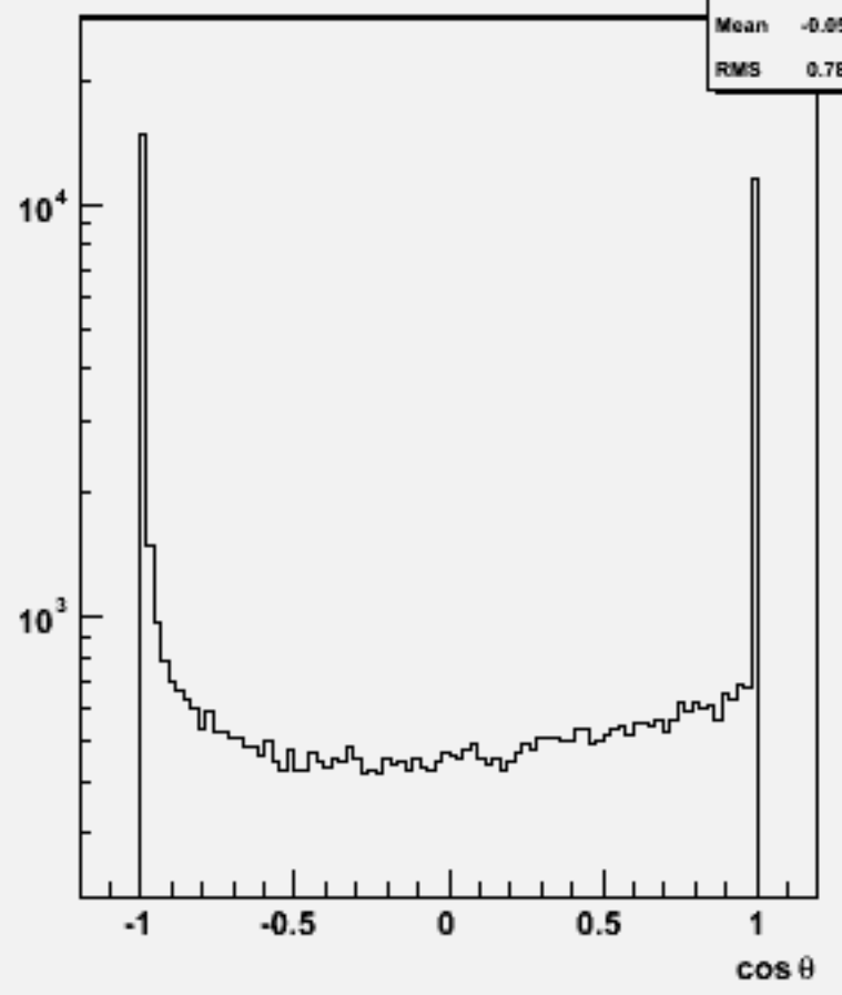
Particle cos θ : w103670 ae1_e1n2e2e2n2_o
