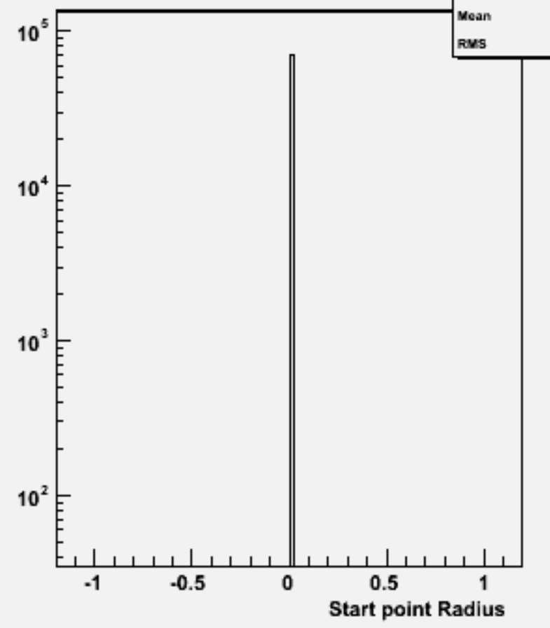
Start point R : w103670 ae1_e1n2e2e2n2_o
