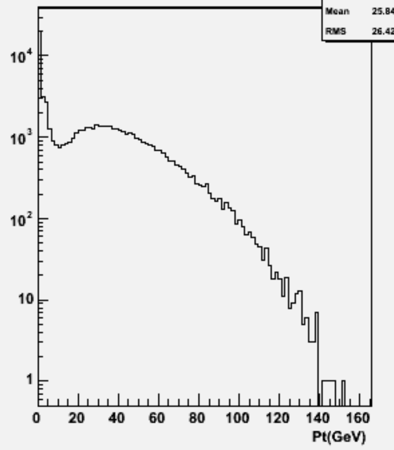
Start point Z : w103670 ae1_e1n2e2e2n2_o
