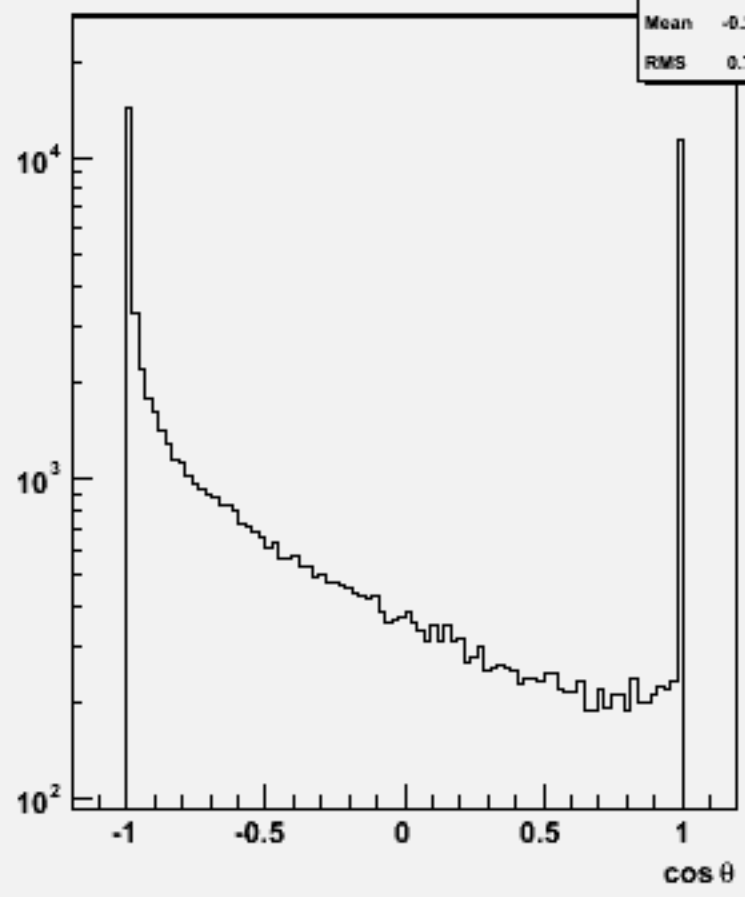
Particle cos θ : w103669 ae1_e1n2e2e2n2_o
