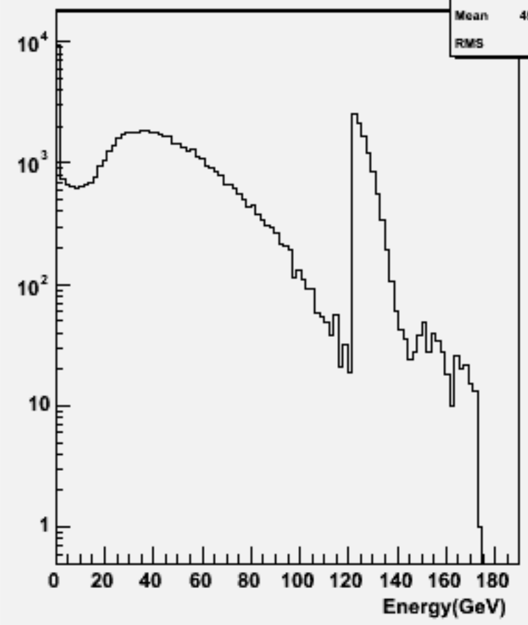
Start point R : w103665 ae1_e1n2e2e1n1_o
