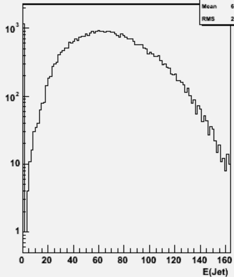
Jet energies(All jets)w103658 ae1_n1udbb_o
