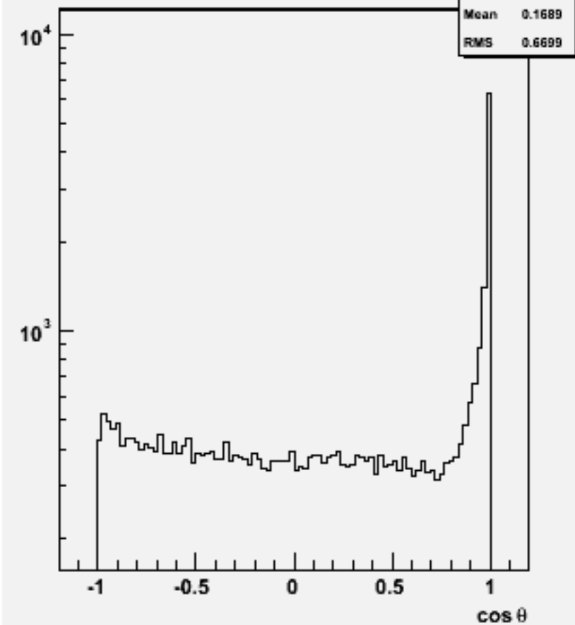
Jet cos \theta (All jets)w103658 ae1_n1udbb_o
