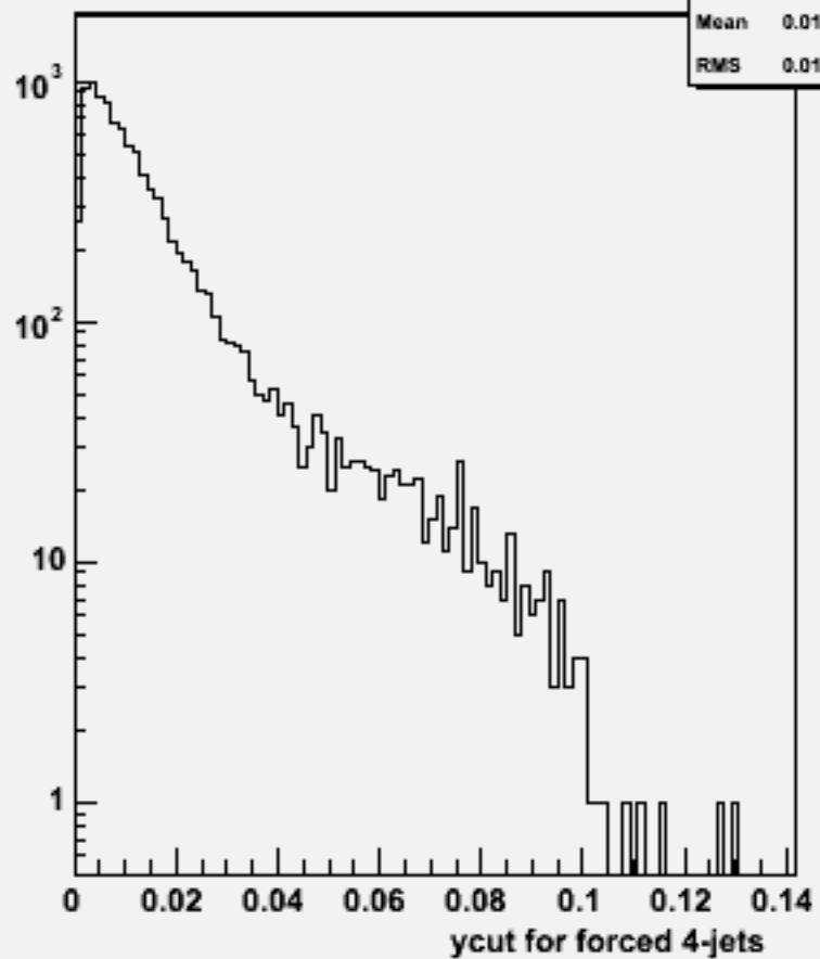
Ycut for 4-jets :w103658 ae1_n1udbb_o
