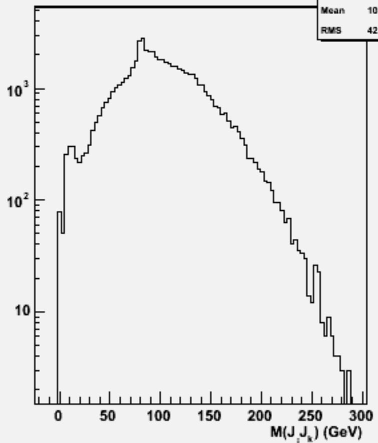
2jets mass(All comb)w103658 ae1_n1udbb_o
