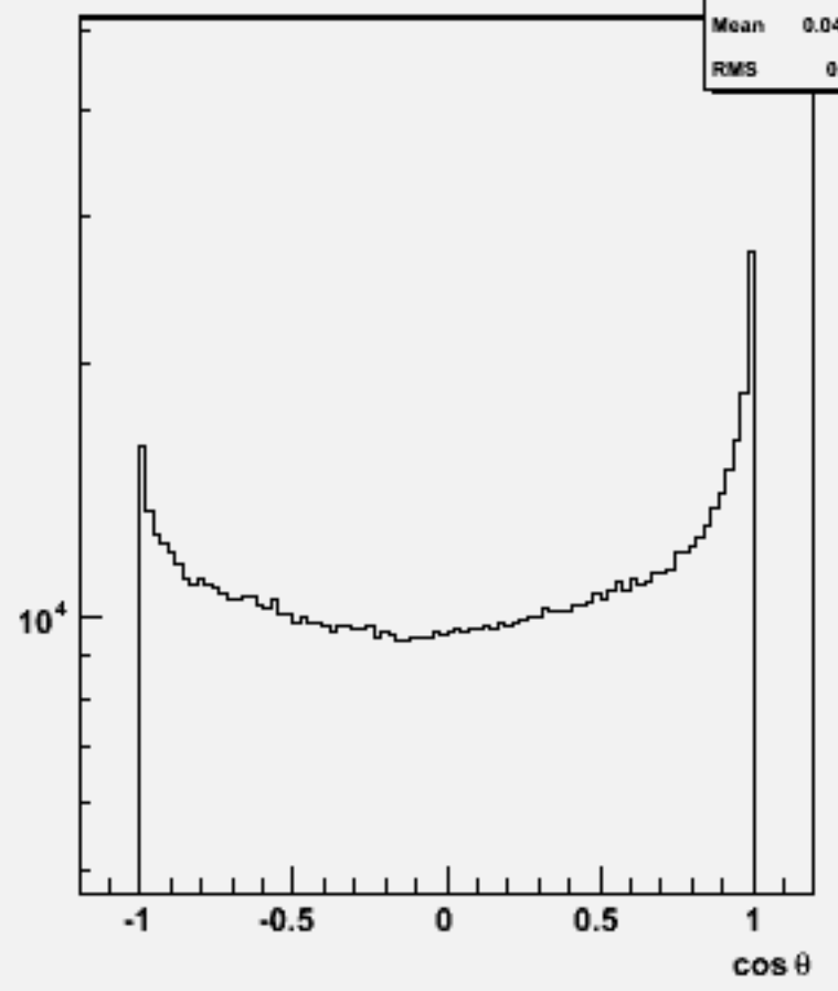
Particle cosθ : w103658 ae1_n1udbb_o
