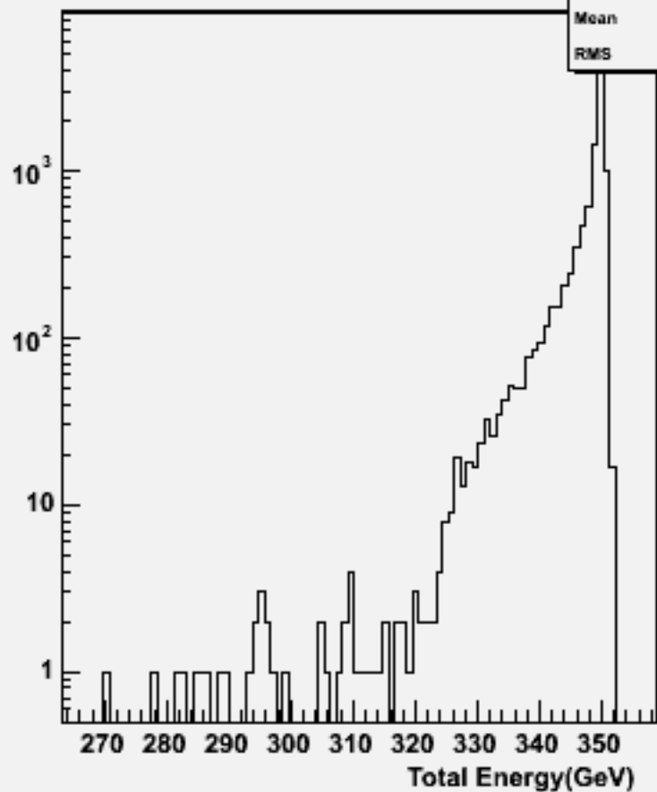
Pt Sum: w103658 ae1_n1udbb_o
