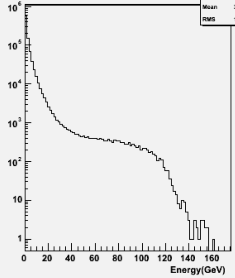
Start point R : w103658 ae1_n1udbb_o
