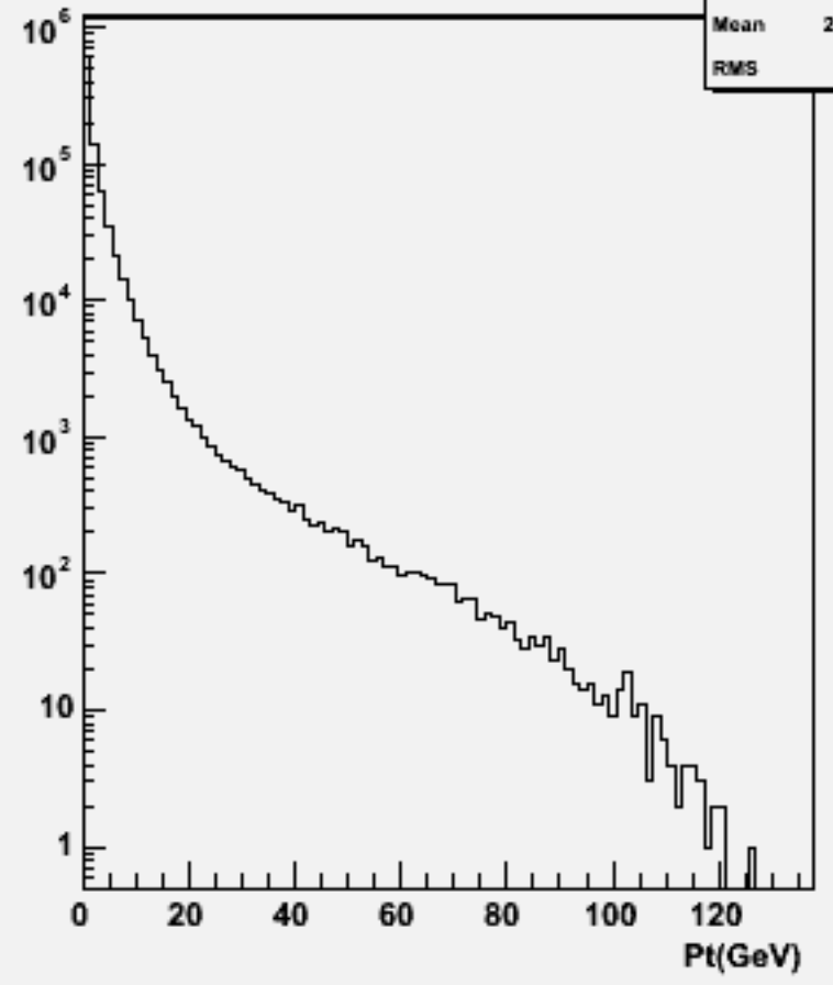
Start point Z : w103658 ae1_n1udbb_o
