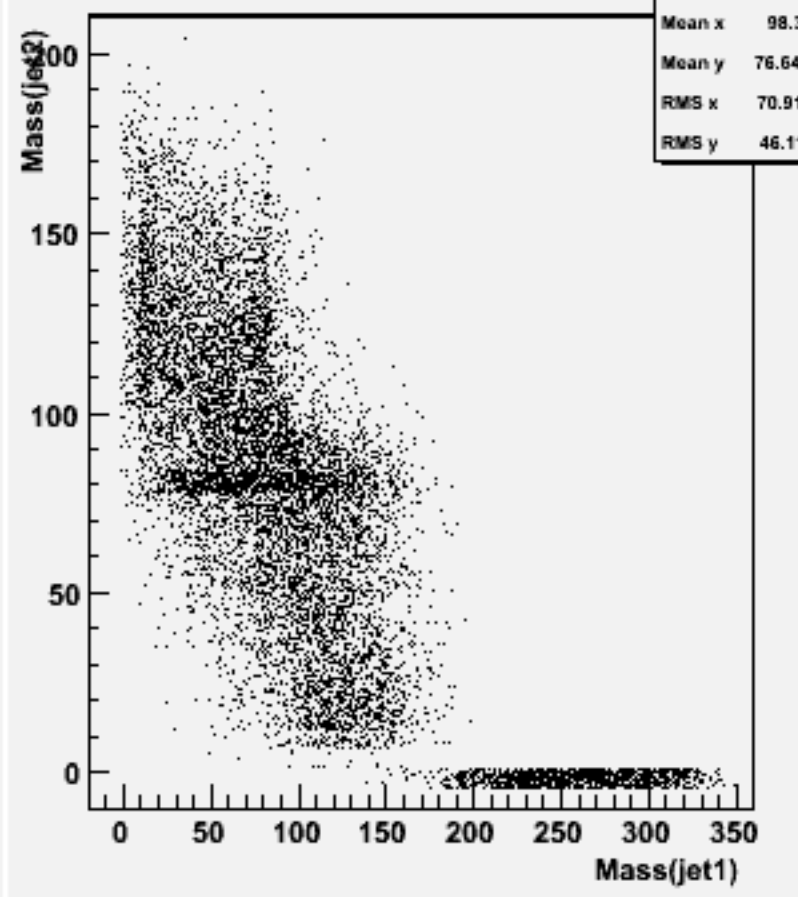
Jet mass for forced 2-jets : w103658 ae1_n1udbb_o
