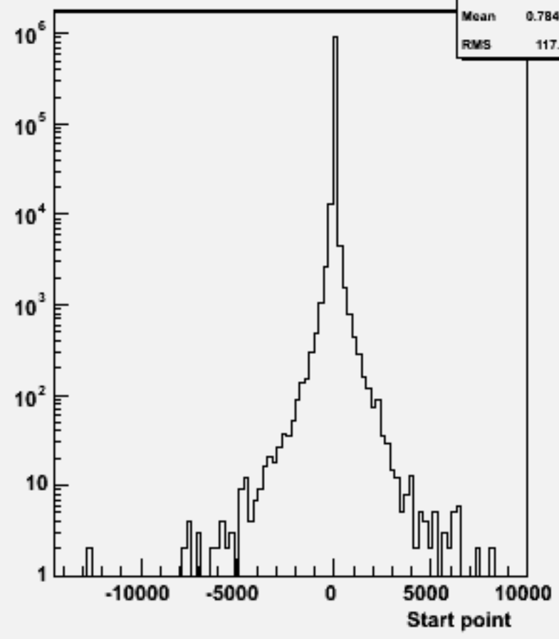
Start point Z : w103658 ae1_n1udbb_o
