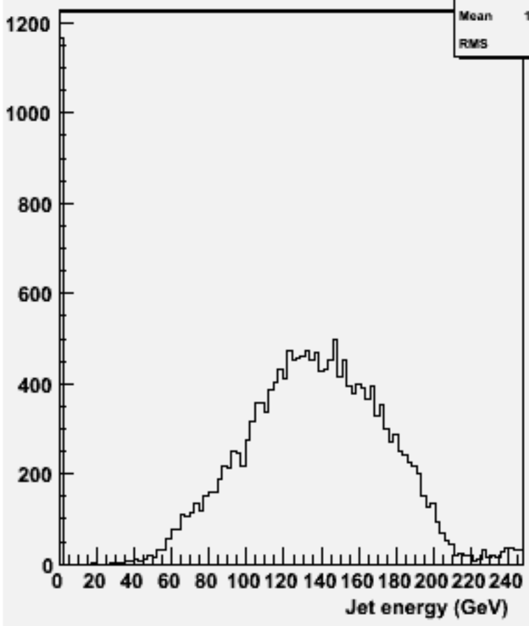
energy for 2-jets :w103658 ae1_n1udbb_o
