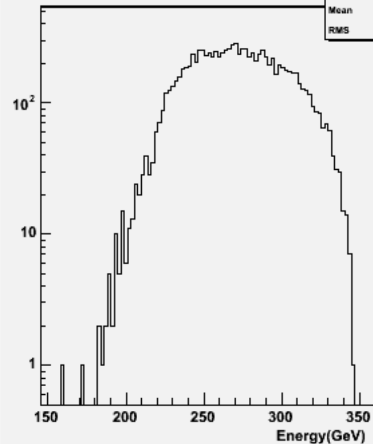
Thrust w103658 ae1_n1udbb_o
