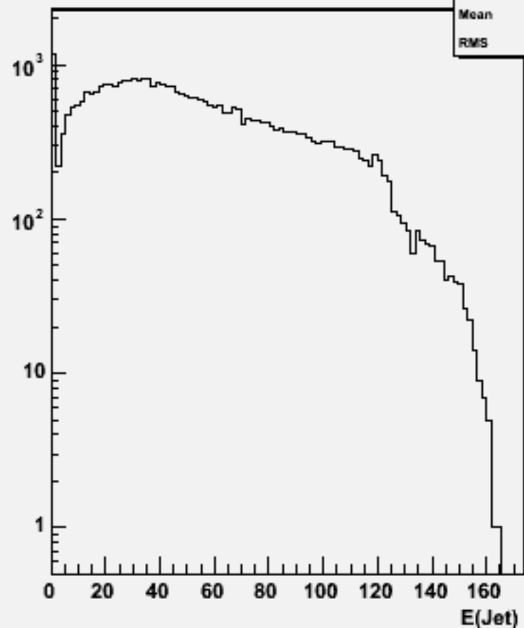
Jet energies(All jets)w103644 ae1_n1n1e1bb_o
