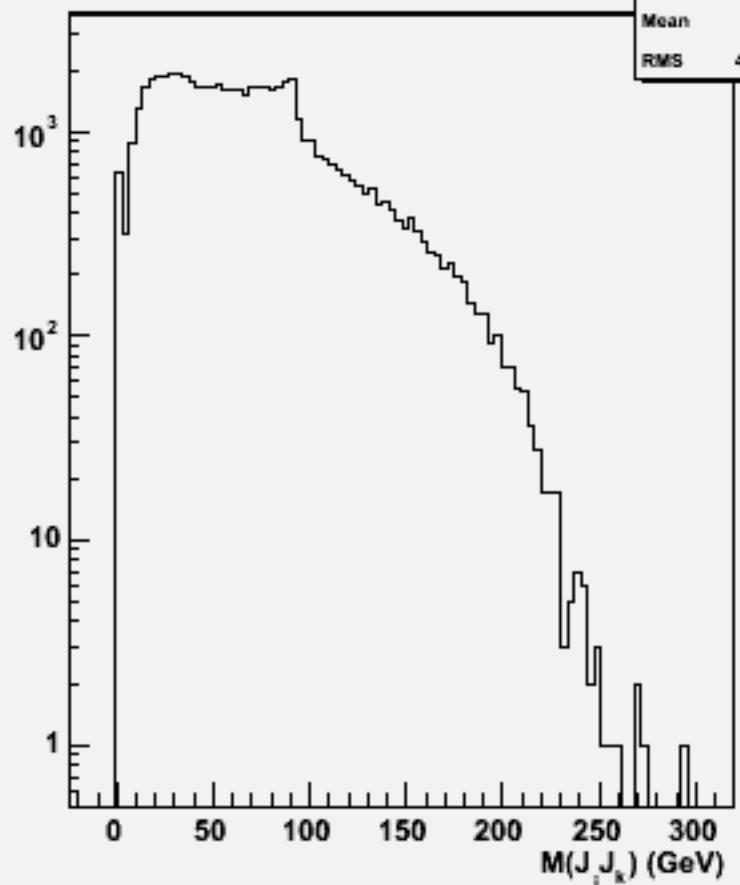
2jets mass(All comb)w103644 ae1_n1n1e1bb_o
