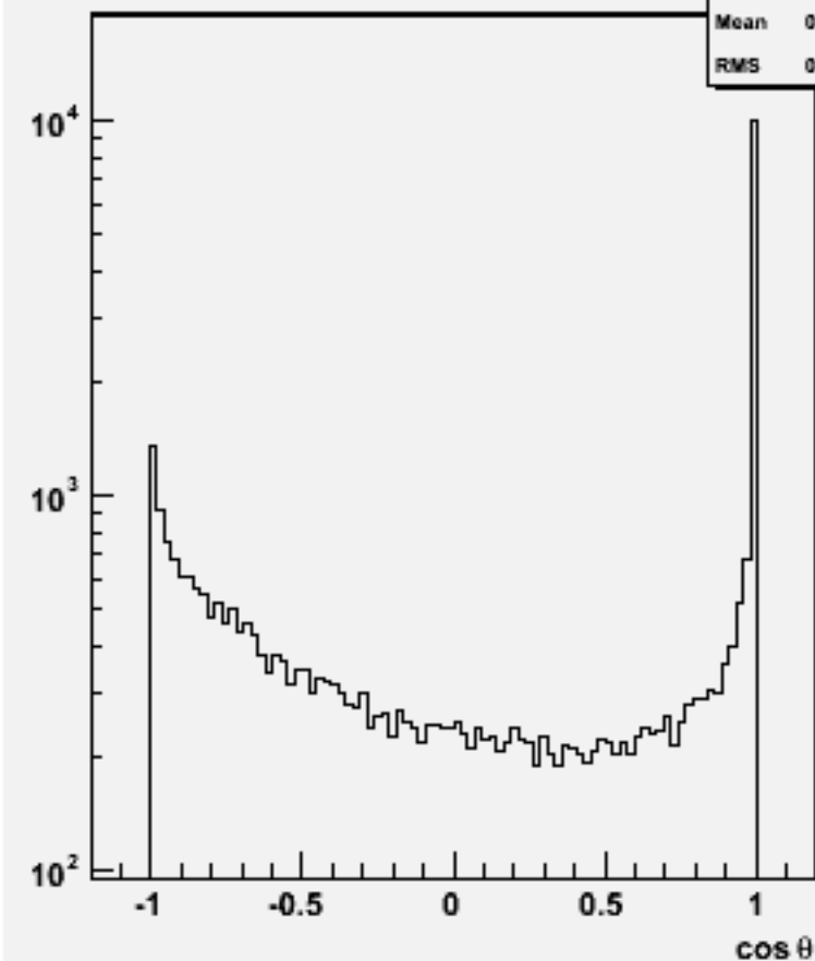
Jet cos \theta (All jets)w103644 ae1_n1n1e1bb_o
