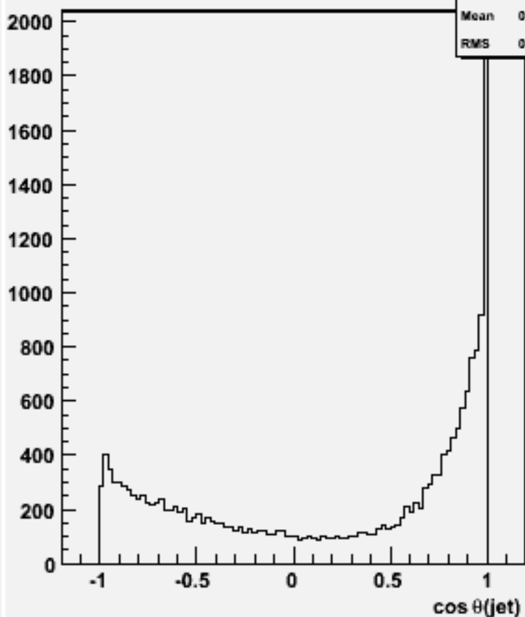
cos \theta for 2-jets :w103642 ae1_n1csss_o
