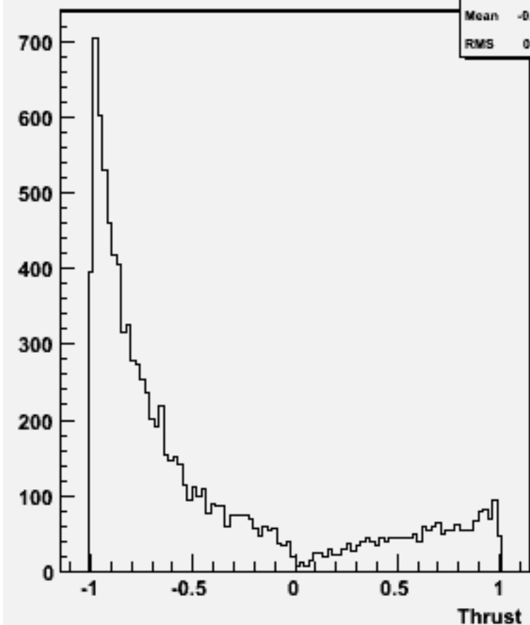
cos \Theta (thrust) w103642 ae1_n1csss_o
