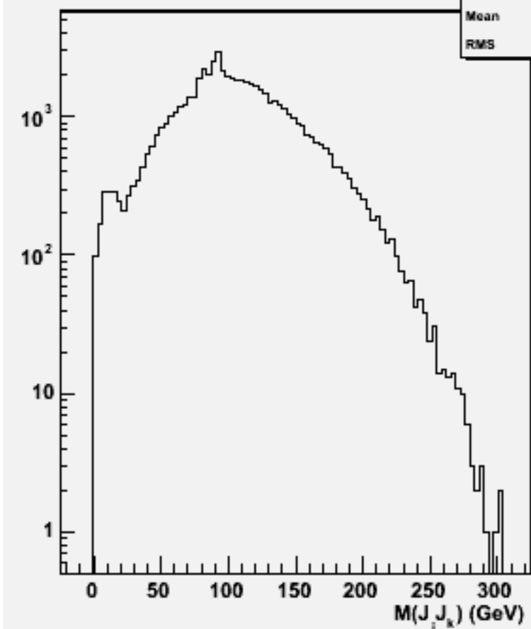
2jets mass(All comb)w103642 ae1_n1csss_o
