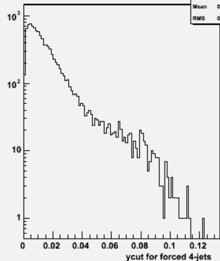
Ycut for 4-jets :w103642 ae1_n1csss_o
