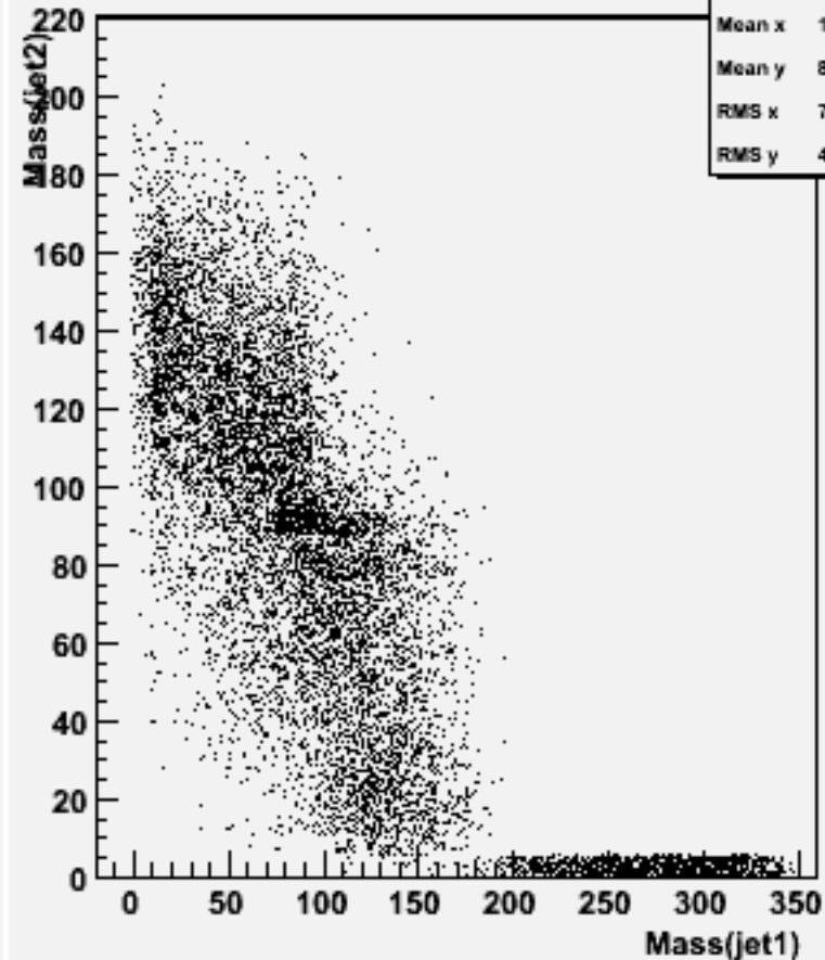
Jet mass for forced 2-jets : w103642 ae1_n1csss_o
