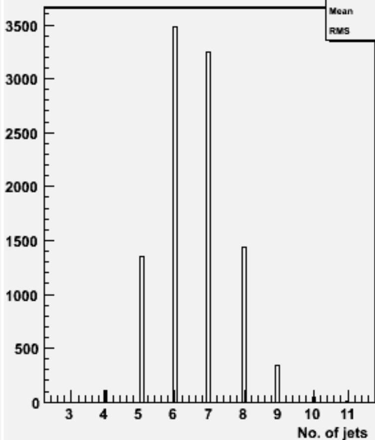
No. jets (ycut=0.001) : w103642 ae1_n1csss_o
