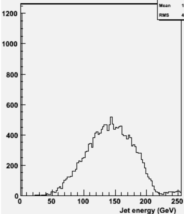
energy for 2-jets :w103642 ae1_n1csss_o
