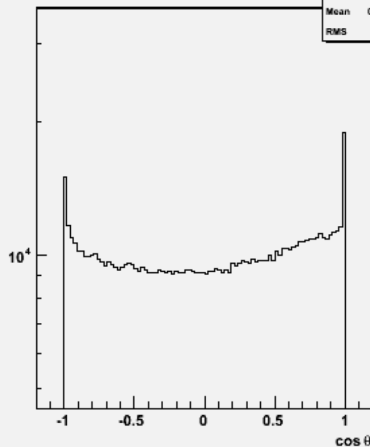
Particle \cos\theta : w103642 ae1_n1csss_o
