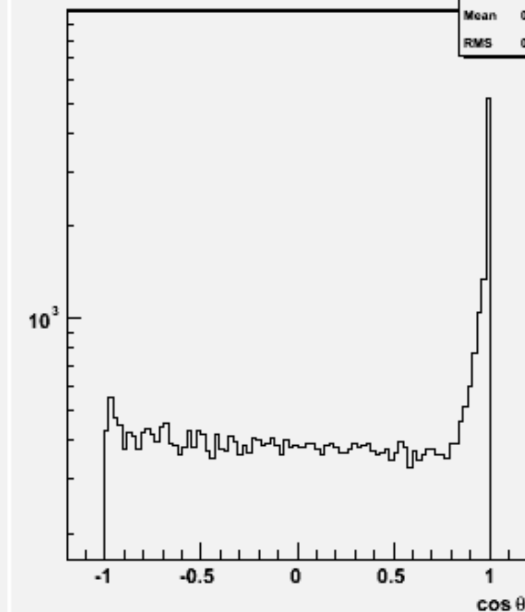
Jet cos \theta (All jets)w103642 ae1_n1csss_o
