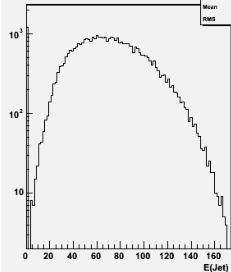
Jet energies(All jets)w103642 ae1_n1csss_o
