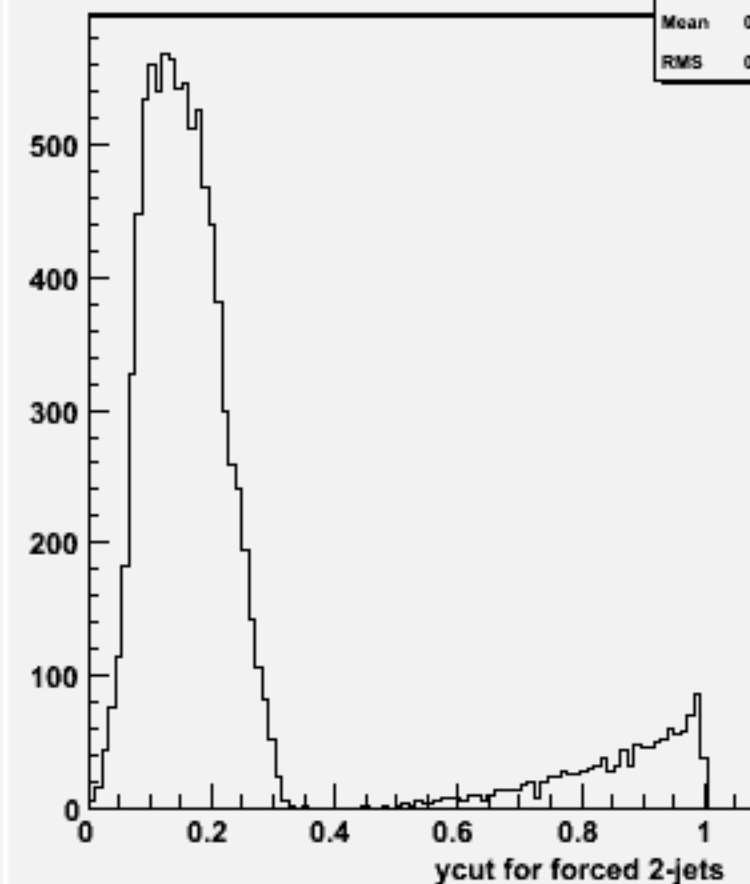
Ycut for 2-jets :w103642 ae1_n1csss_o
