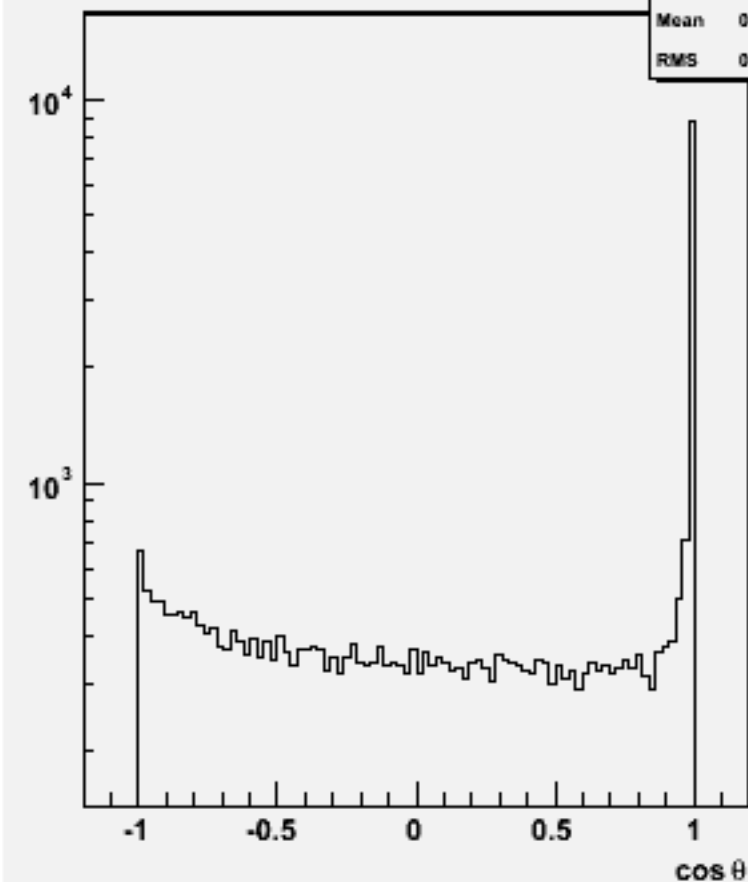
Jet cos \theta (All jets)w103634 ae1_n1n3e3ss_o
