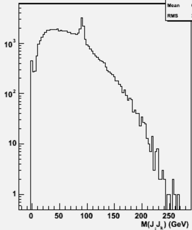
2jets mass(All comb)w103634 ae1_n1n3e3ss_o
