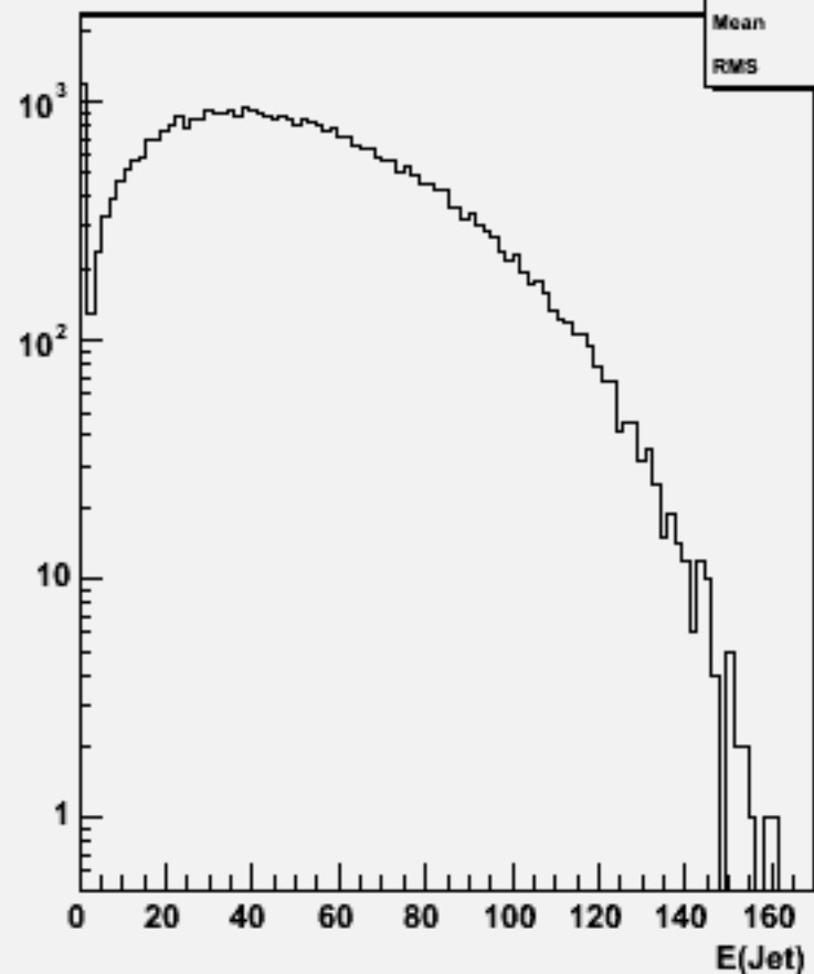
Jet energies(All jets)w103634 ae1_n1n3e3ss_o
