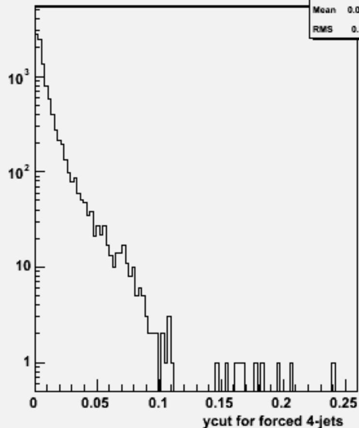
Ycut for 4-jets :w103634 ae1_n1n3e3ss_o
