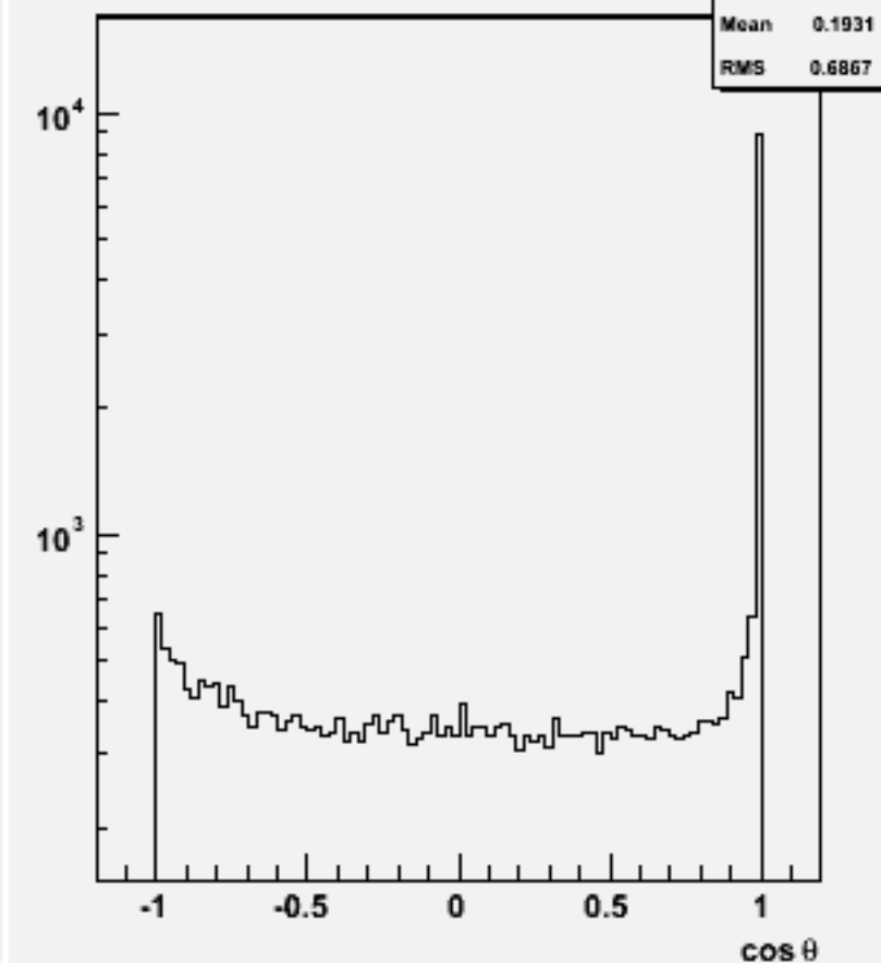
Jet cos theta (All jets)w103626 ae1_n1n1e1ss_o
