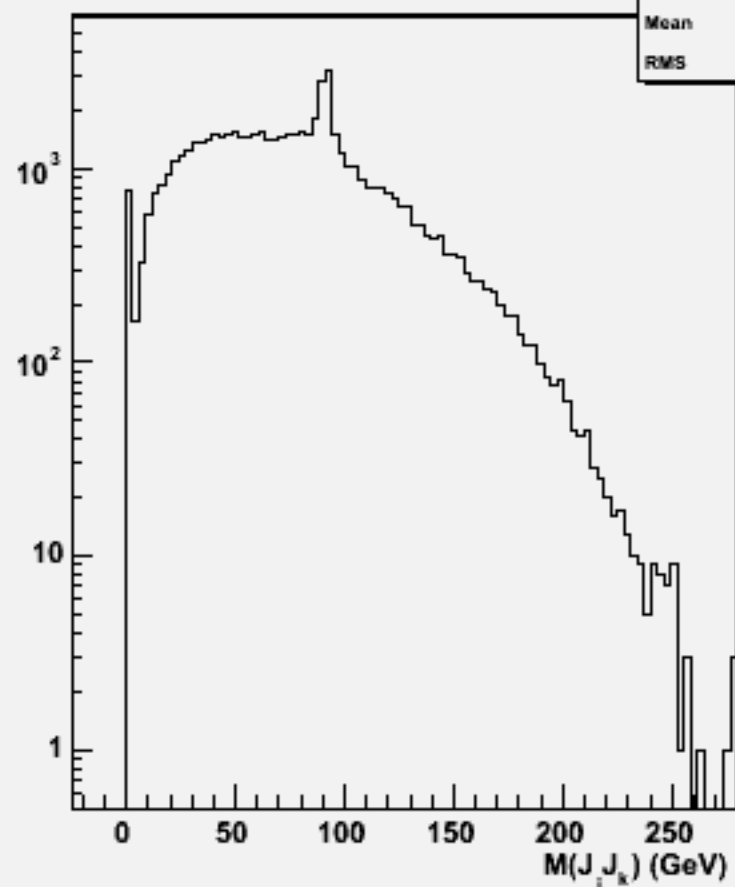
2jets mass(All comb)w103626 ae1_n1n1e1ss_o
