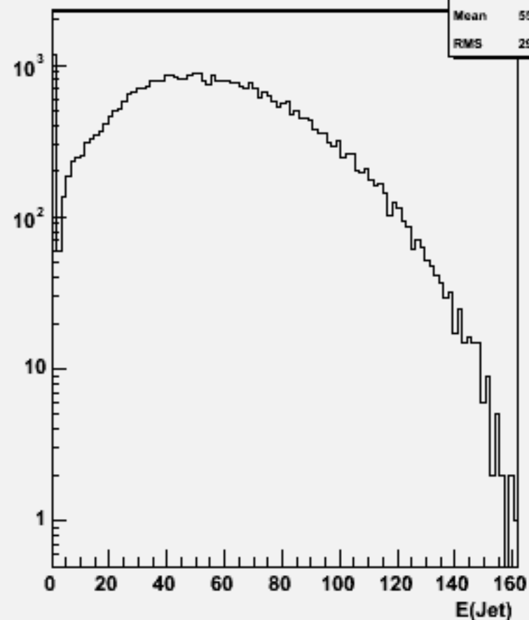
Jet energies(All jets)w103626 ae1_n1n1e1ss_o
