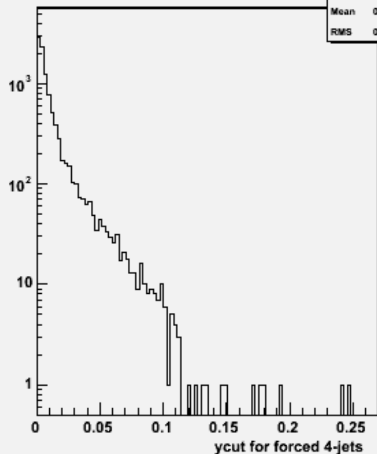
Ycut for 4-jets :w103626 ae1_n1n1e1ss_o
