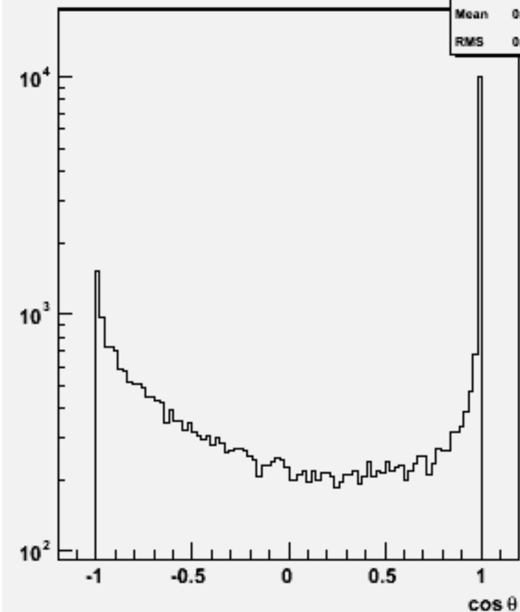
Jet cos \theta (All jets)w103624 ae1_n1n1e1ss_o
