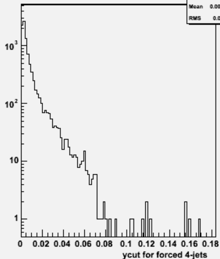
Ycut for 4-jets :w103603 ae1_n1cse3e3_o
