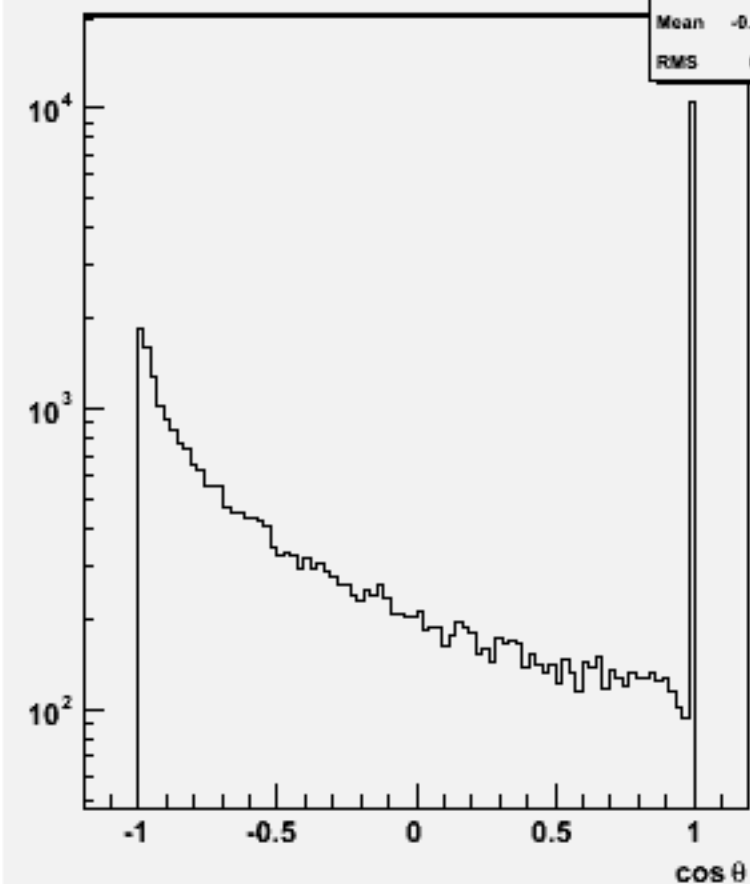
Jet cos \theta (All jets)w103603 ae1_n1cse3e3_o
