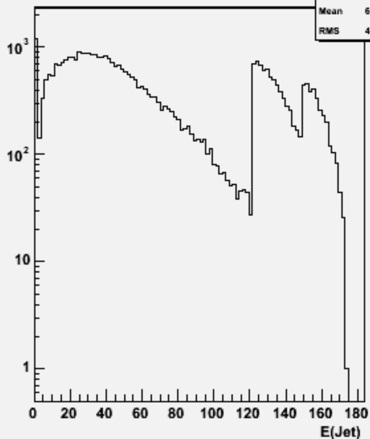
Jet energies(All jets)w103603 ae1_n1cse3e3_o
