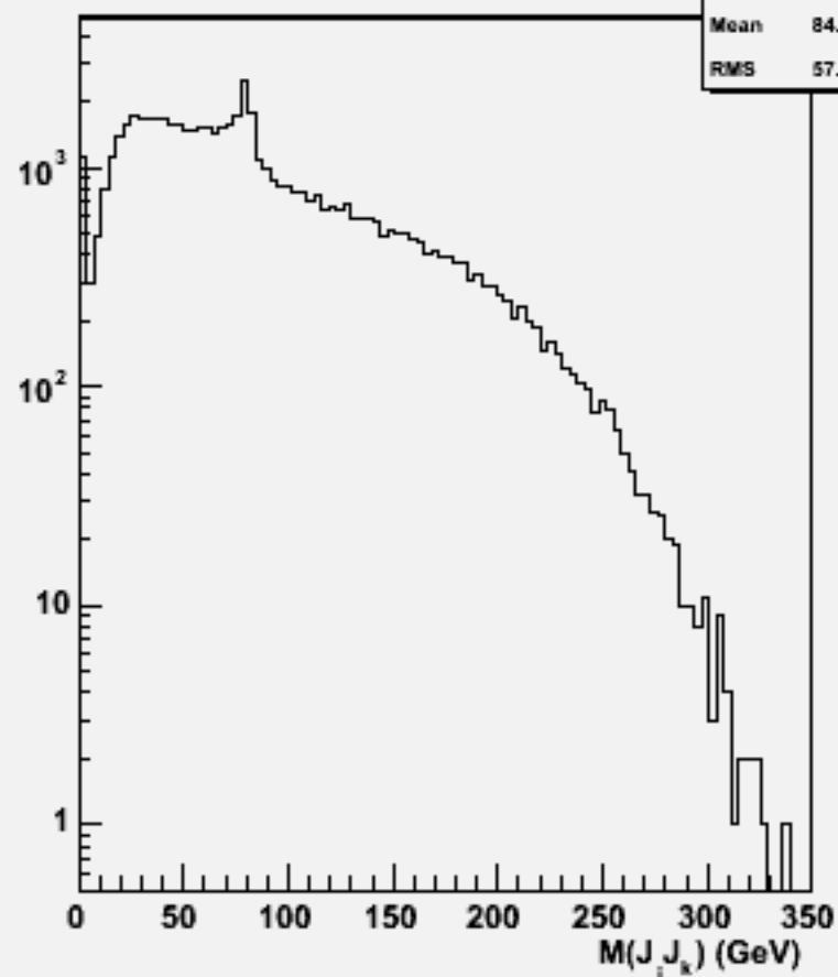
2jets mass(All comb)w103603 ae1_n1cse3e3_o
