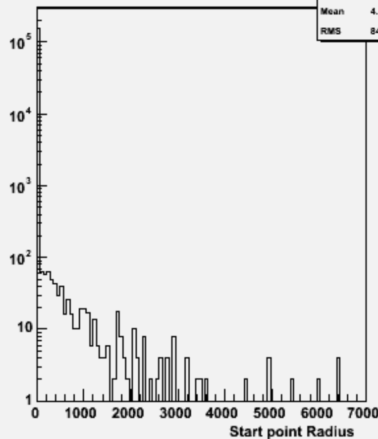
Start point R : w103594 ae1_n1n3e3e3e3_o
