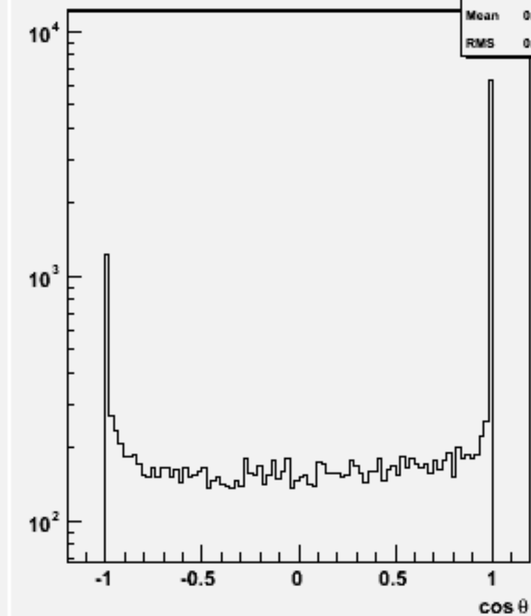
Jet cos \theta (All jets)w103594 ae1_n1n3e3e3e3_o
