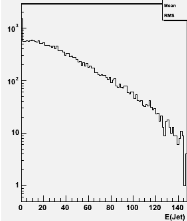
Jet energies(All jets)w103594 ae1_n1n3e3e3e3_o
