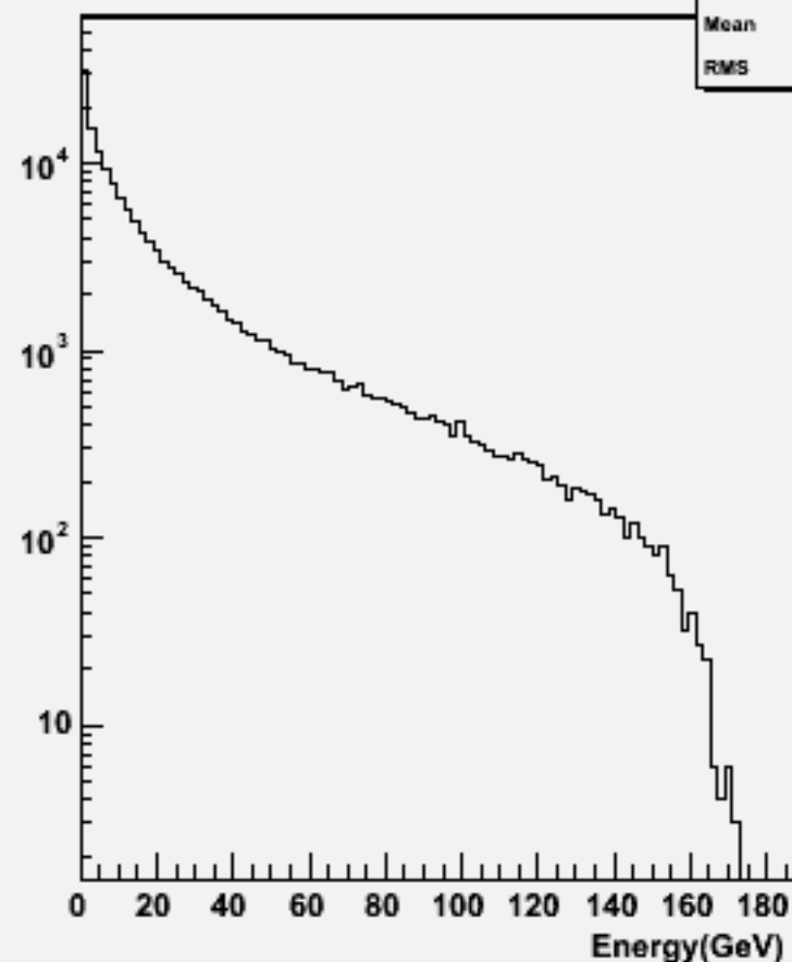
Start point R : w103594 ae1_n1n3e3e3e3_o
