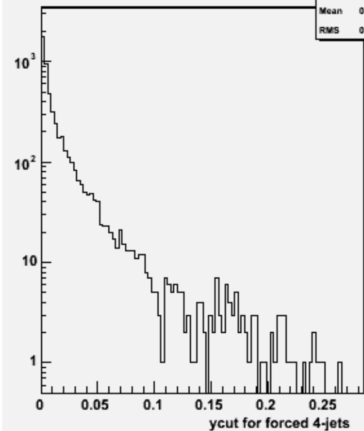
Ycut for 4-jets :w103594 ae1_n1n3e3e3e3_o
