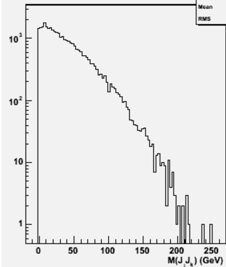
2jets mass(All comb)w103594 ae1_n1n3e3e3e3_o
