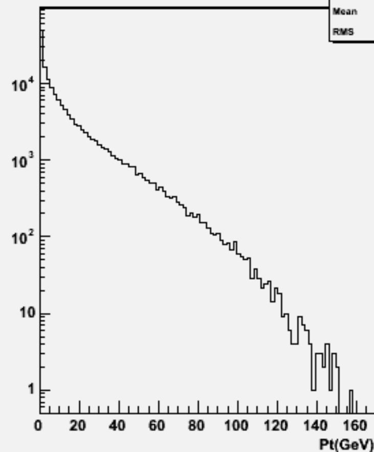
Start point Z : w103594 ae1_n1n3e3e3e3_o
