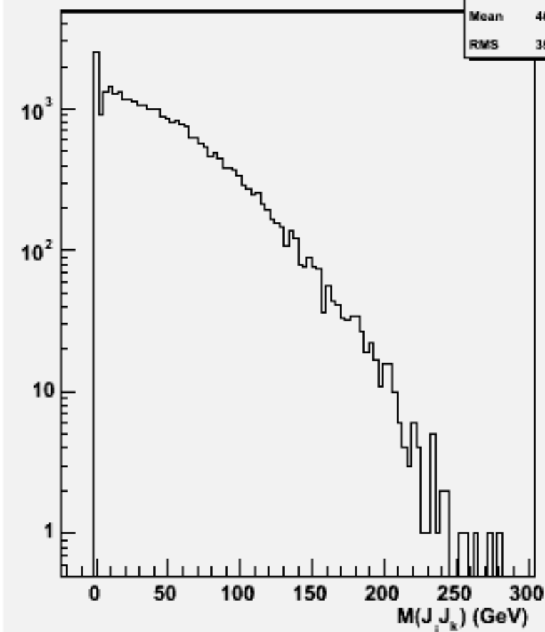
2jets mass(All comb)w103590 ae1_n1n2e2e3e3_o
