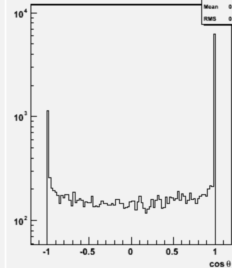
Jet cos \theta (All jets)w103590 ae1_n1n2e2e3e3_o
