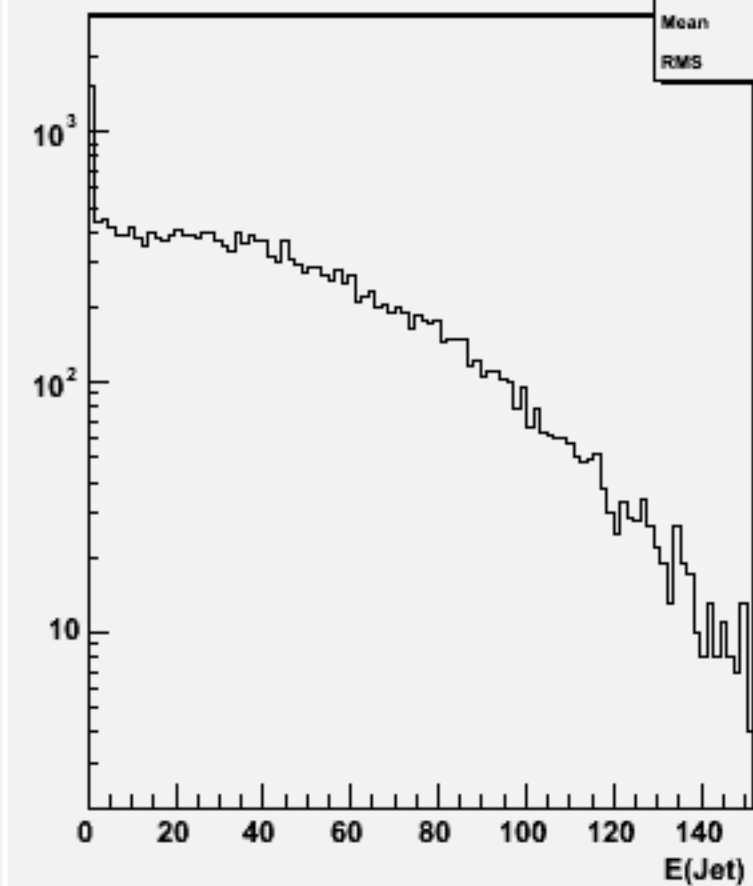
Jet energies(All jets)w103590 ae1_n1n2e2e3e3_o
