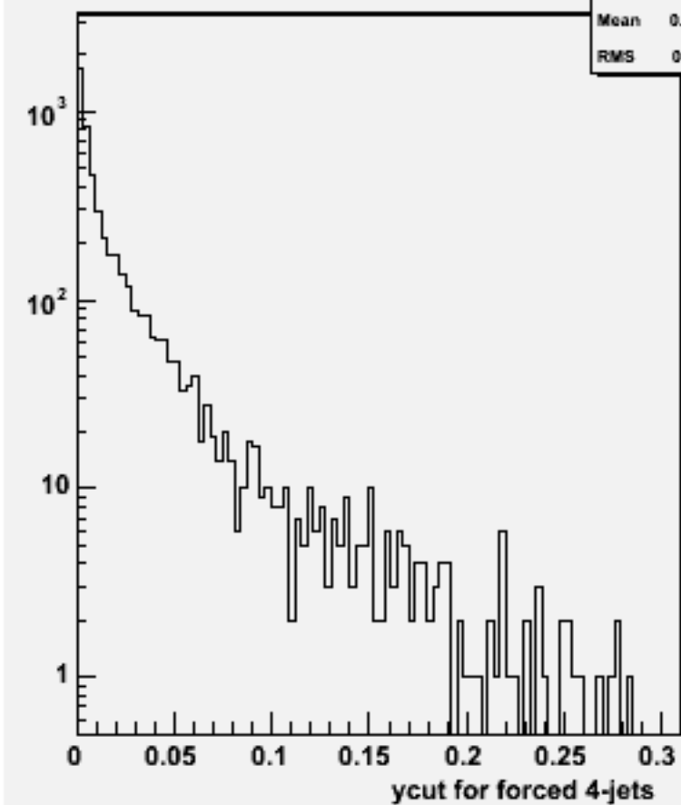
Ycut for 4-jets :w103590 ae1_n1n2e2e3e3_o
