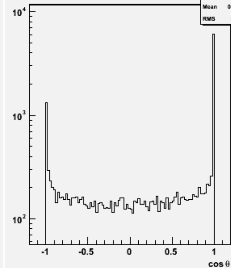
Jet cos \theta (All jets)w103586 ae1_n1n1e1e3e3_o
