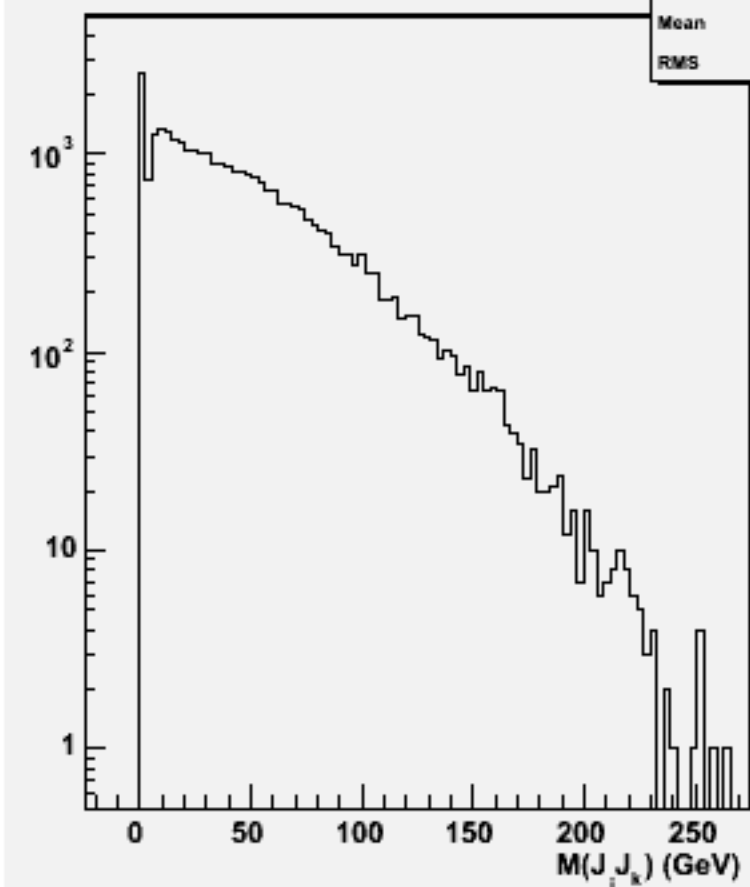
2jets mass(All comb)w103586 ae1_n1n1e1e3e3_o
