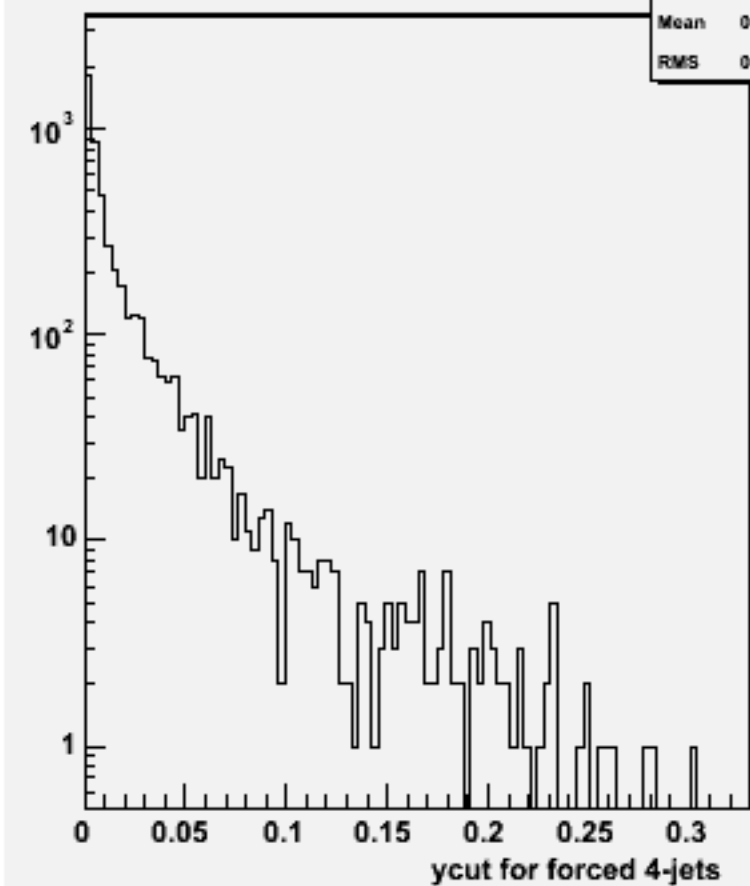
Ycut for 4-jets :w103586 ae1_n1n1e1e3e3_o
