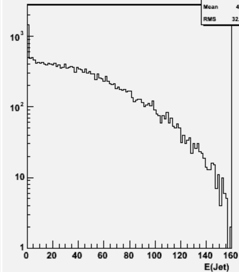
Jet energies(All jets)w103586 ae1_n1n1e1e3e3_o
