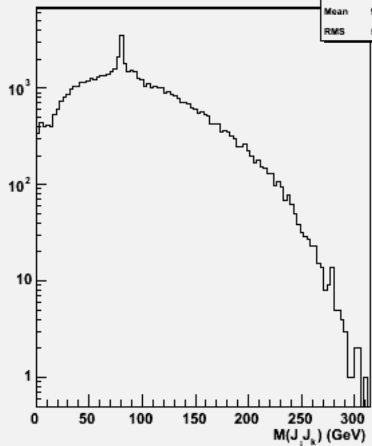
2jets mass(All comb)w103582 ae1_n1cse2e2_o
