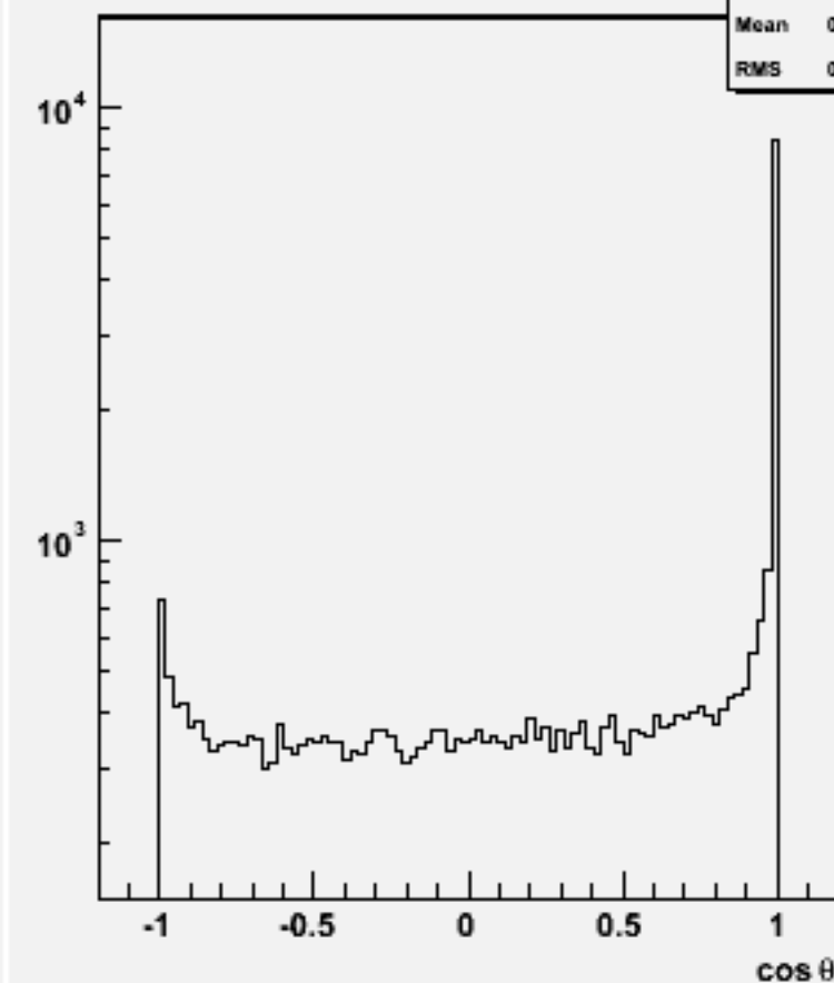
Jet cos \theta (All jets)w103582 ae1_n1cse2e2_o
