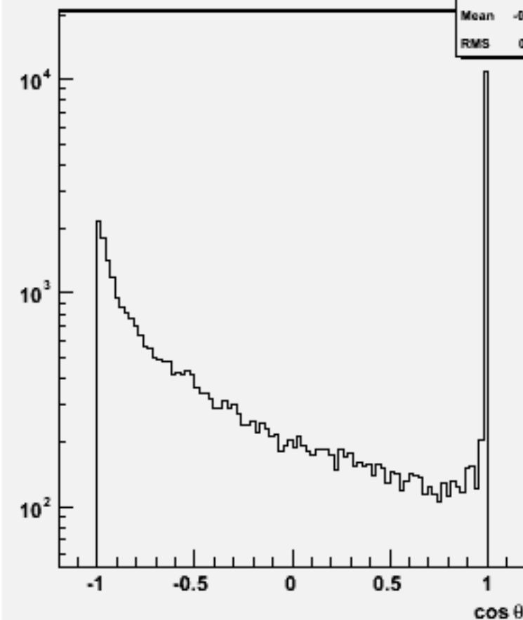
Jet cos \theta (All jets)w103579 ae1_n1ude2e2_o
