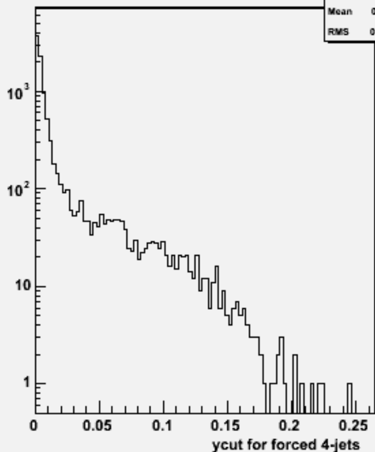
Ycut for 4-jets :w103579 ae1_n1ude2e2_o
