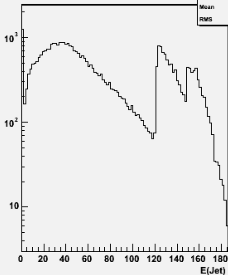
Jet energies(All jets)w103579 ae1_n1ude2e2_o
