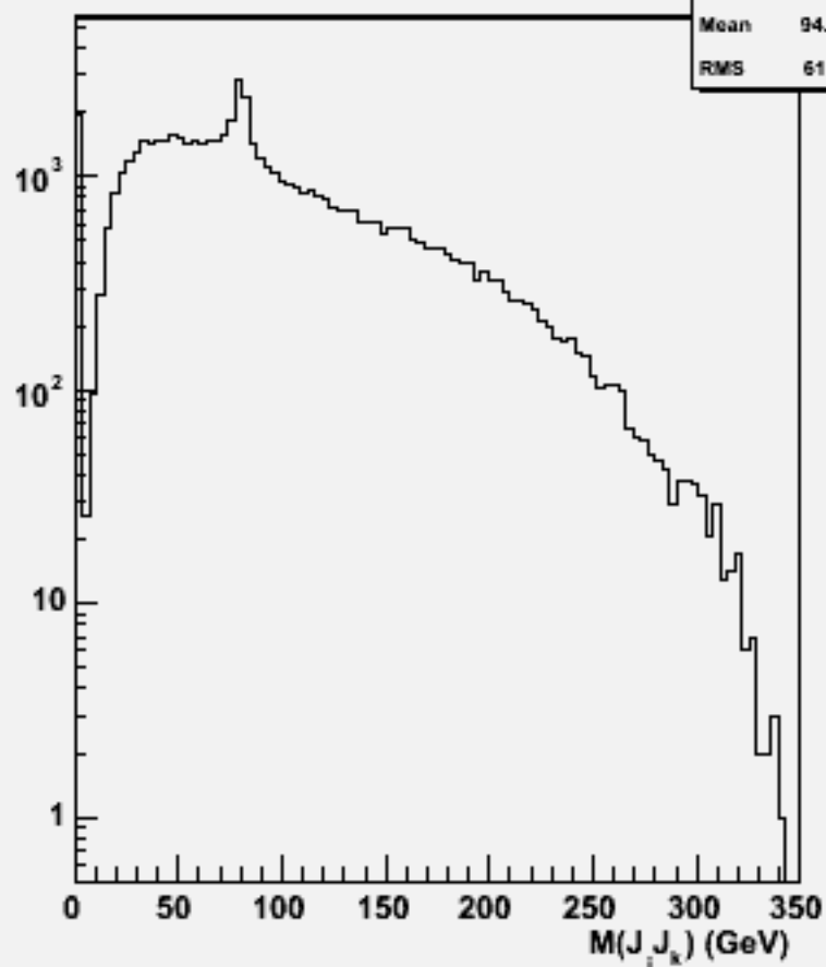
2jets mass(All comb)w103579 ae1_n1ude2e2_o
