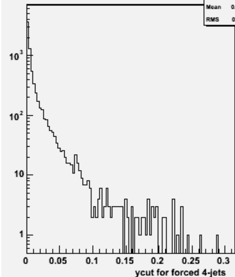
Ycut for 4-jets :w103574 ae1_n1n3e3e2e2_o
