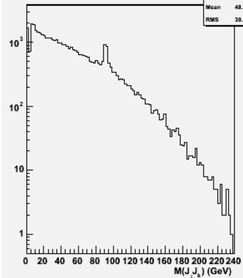
2jets mass(All comb)w103574 ae1_n1n3e3e2e2_o
