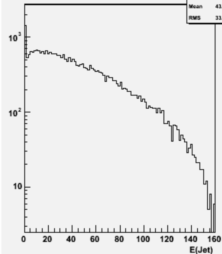
Jet energies(All jets)w103574 ae1_n1n3e3e2e2_o
