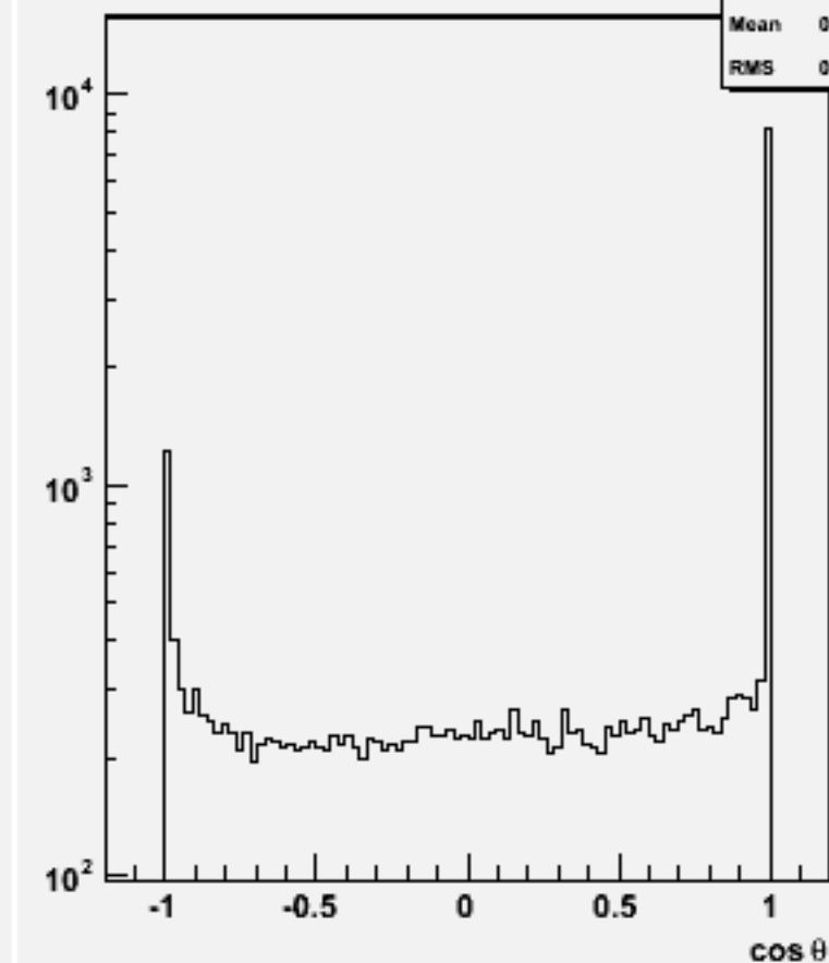
Jet cos \theta (All jets)w103574 ae1_n1n3e3e2e2_o
