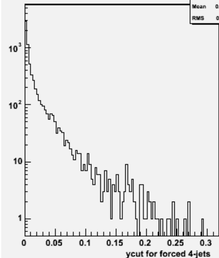
Ycut for 4-jets :w103570 ae1_n1n2e2e2e2_o
