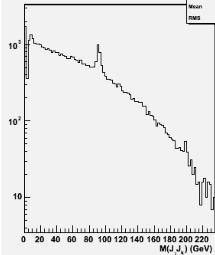
2jets mass(All comb)w103570 ae1_n1n2e2e2e2_o
