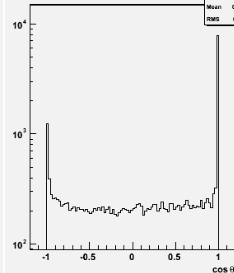
Jet cos \theta (All jets)w103570 ae1_n1n2e2e2e2_o
