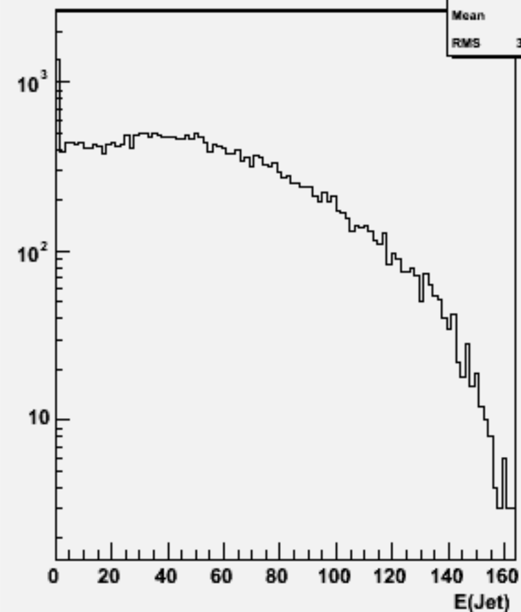
Jet energies(All jets)w103570 ae1_n1n2e2e2e2_o
