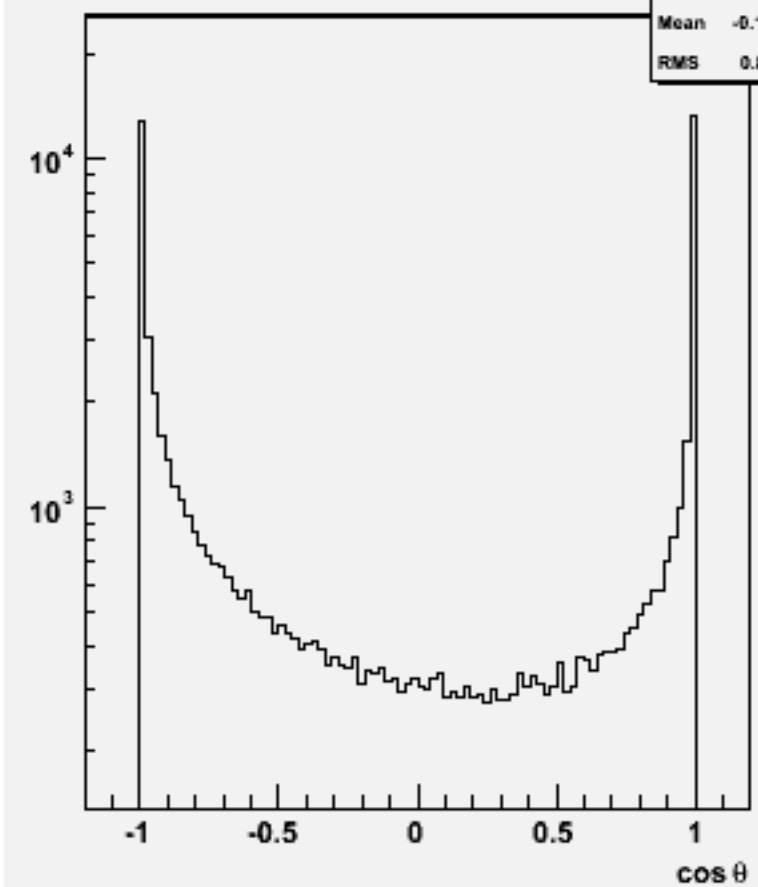
Particle cos \theta : w103564 ae1_n1n1e1e2e2_o
