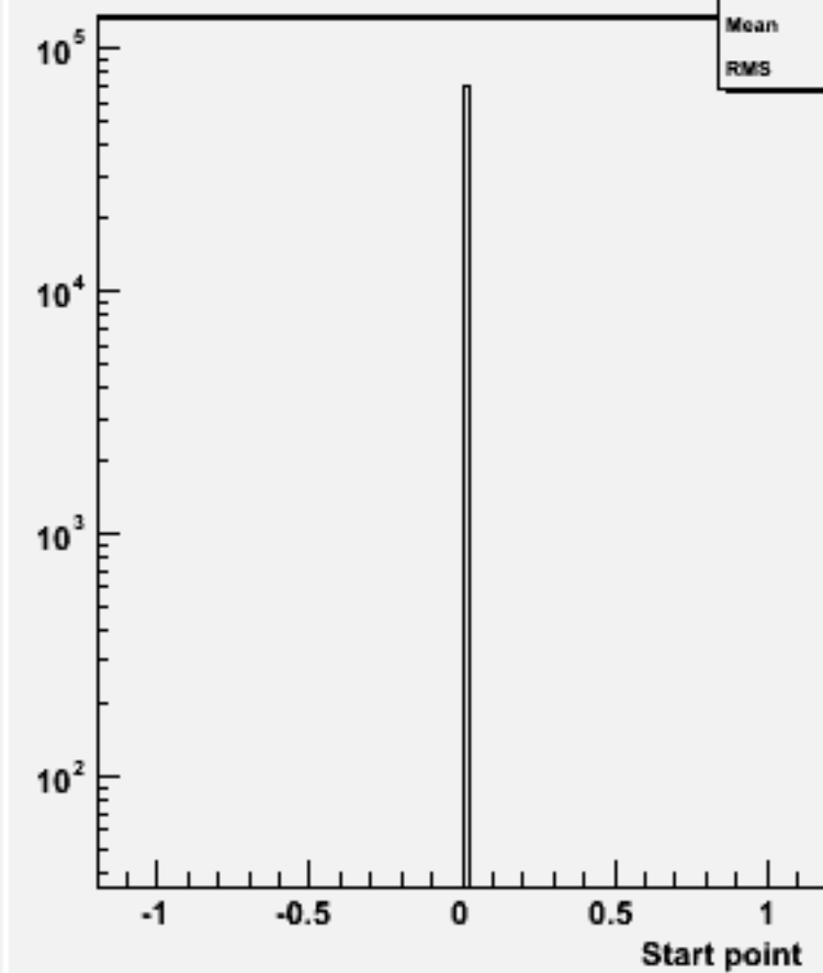
Start point Z : w103564 ae1_n1n1e1e2e2_o
