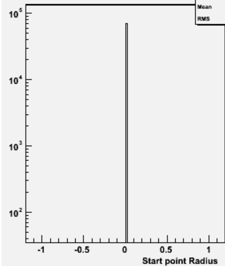
Start point R : w103564 ae1_n1n1e1e2e2_o
