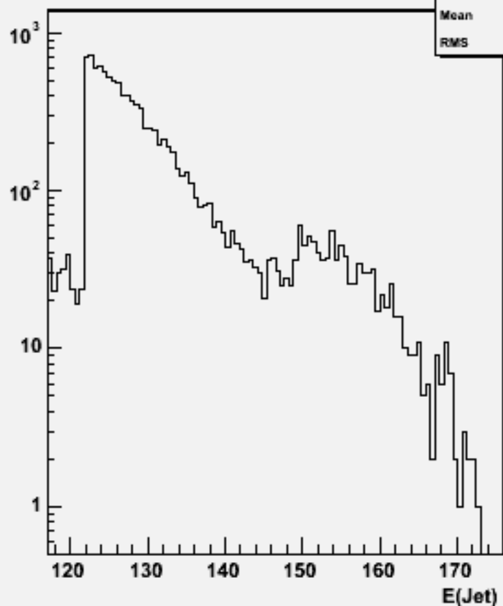
Jet energies(All jets)w103563 ae1_n1cse1e1_o
