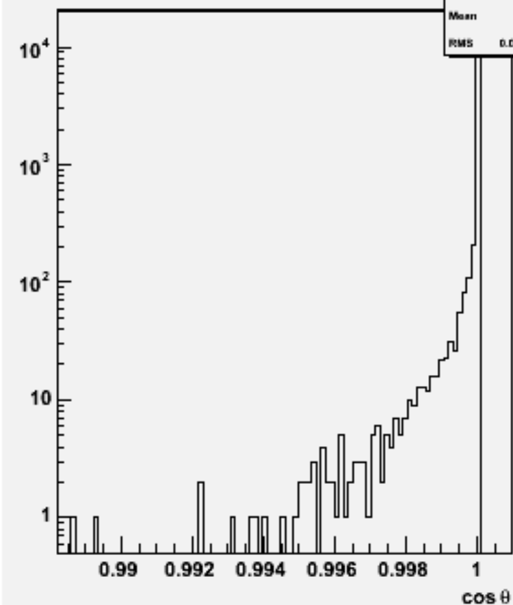
Jet cos \theta (All jets)w103563 ae1_n1cse1e1_o
