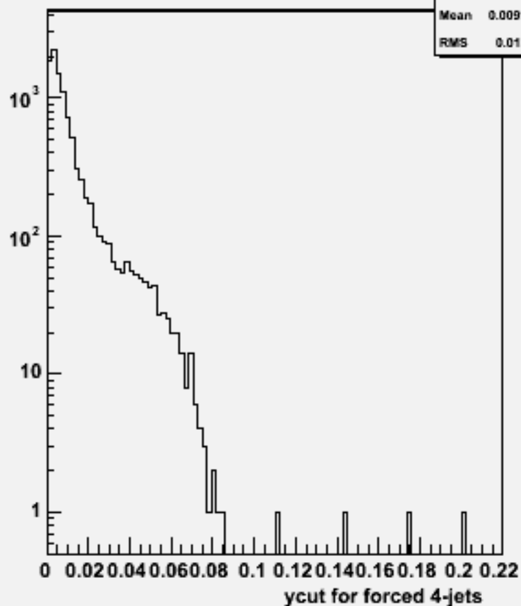
Ycut for 4-jets :w103563 ae1_n1cse1e1_o
