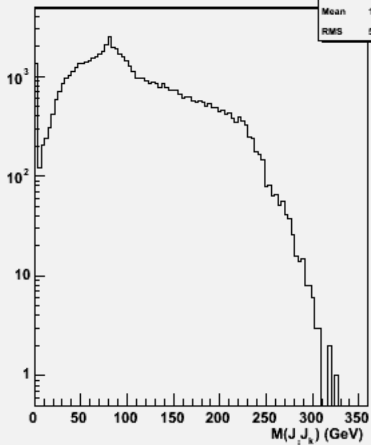
2jets mass(All comb)w103563 ae1_n1cse1e1_o
