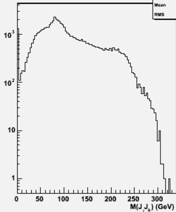
2jets mass(All comb)w103561 ae1_n1cse1e1_o
