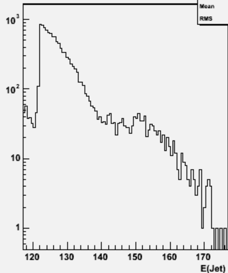
Jet energies(All jets)w103561 ae1_n1cse1e1_o
