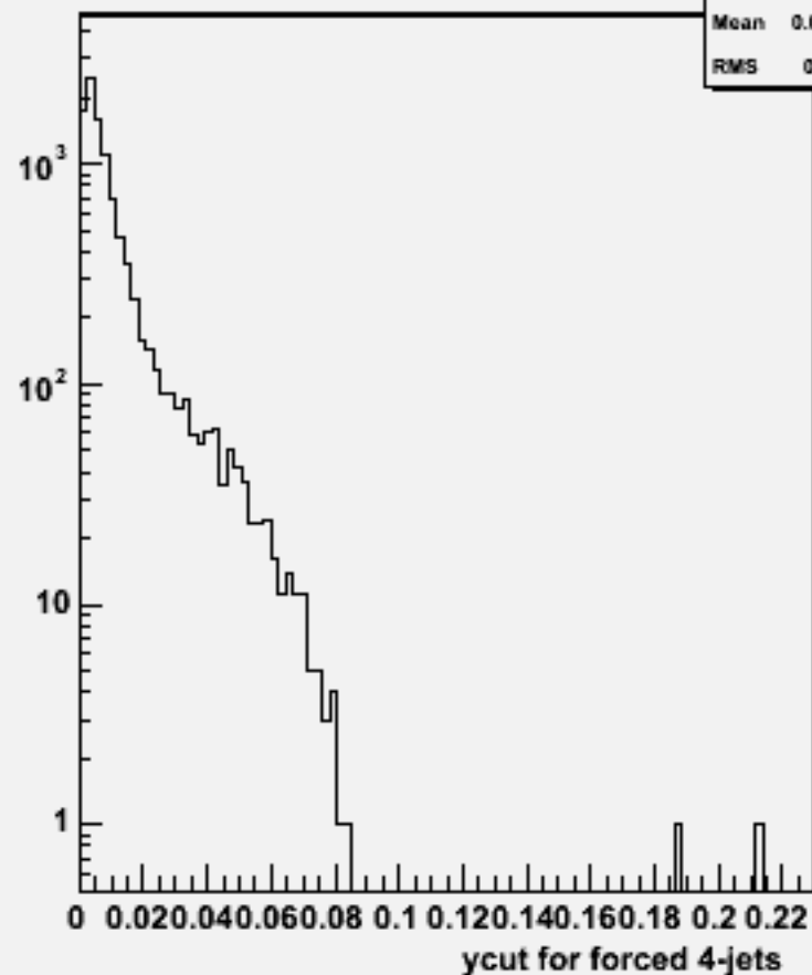
Ycut for 4-jets :w103561 ae1_n1cse1e1_o
