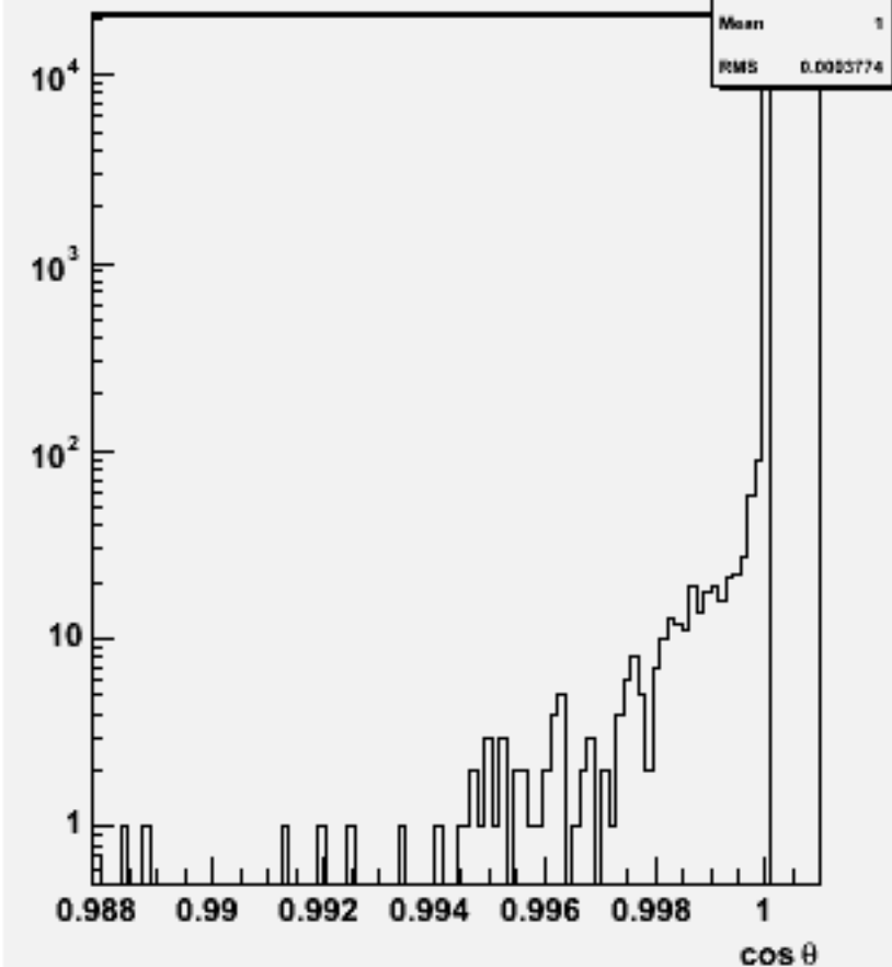
Jet cos theta (All jets)w103561 ae1_n1cse1e1_o
