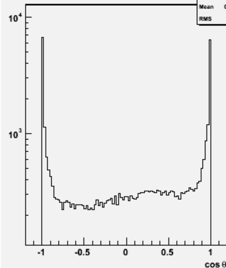
Jet cos \theta (All jets)w103560 ae1_n1cse1e1_o
