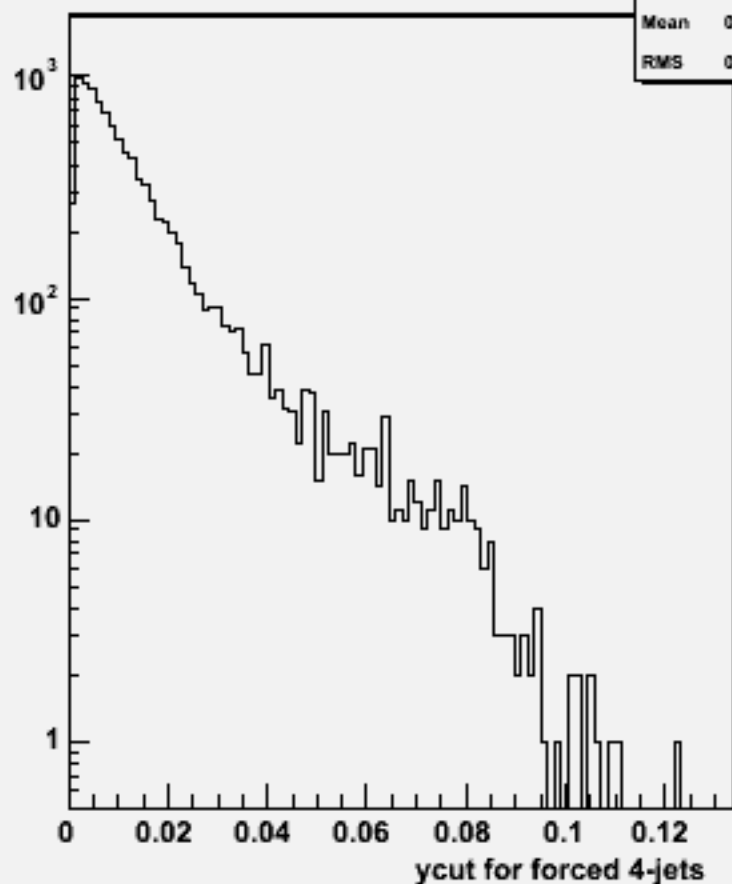
Ycut for 4-jets :w103560 ae1_n1cse1e1_o
