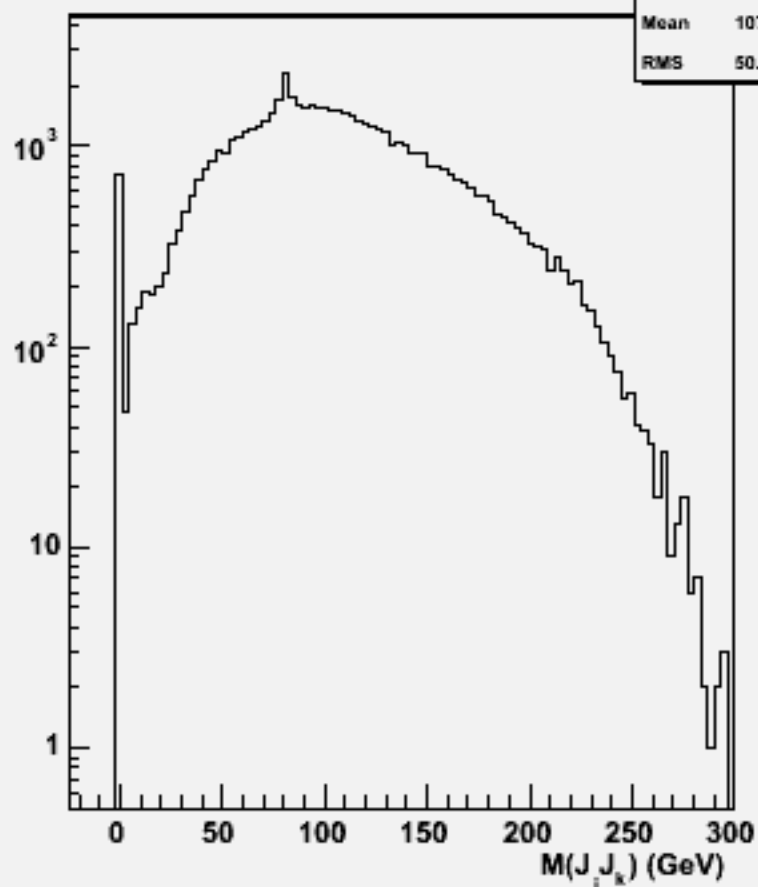
2jets mass(All comb)w103560 ae1_n1cse1e1_o
