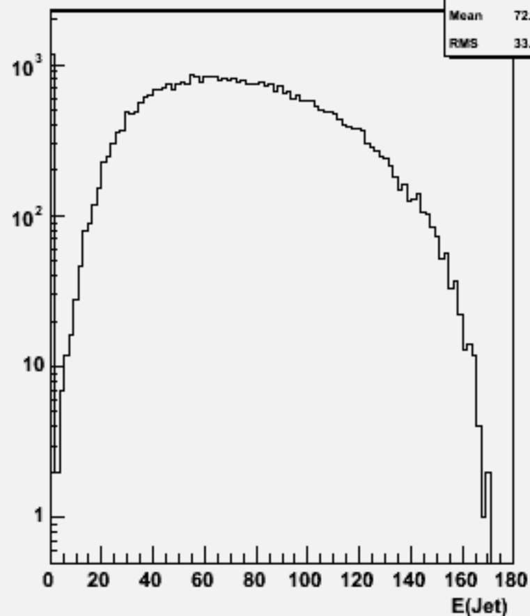
Jet energies(All jets)w103560 ae1_n1cse1e1_o
