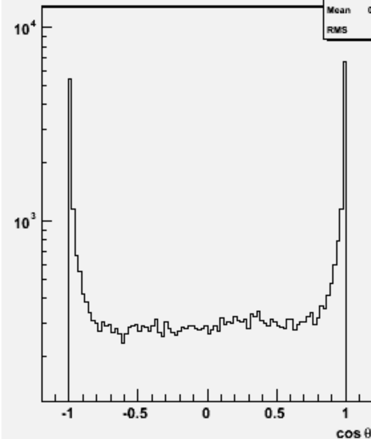
Jet cos \theta (All jets)w103558 ae1_n1ude1e1_o
