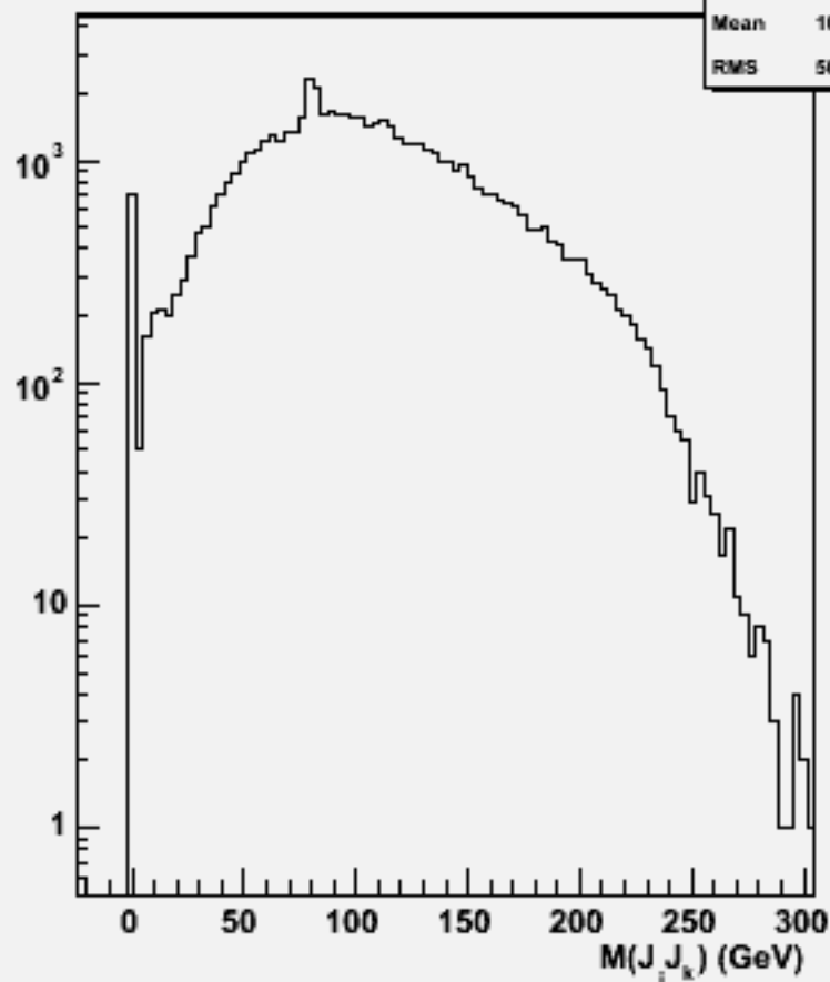
2jets mass(All comb)w103558 ae1_n1ude1e1_o
