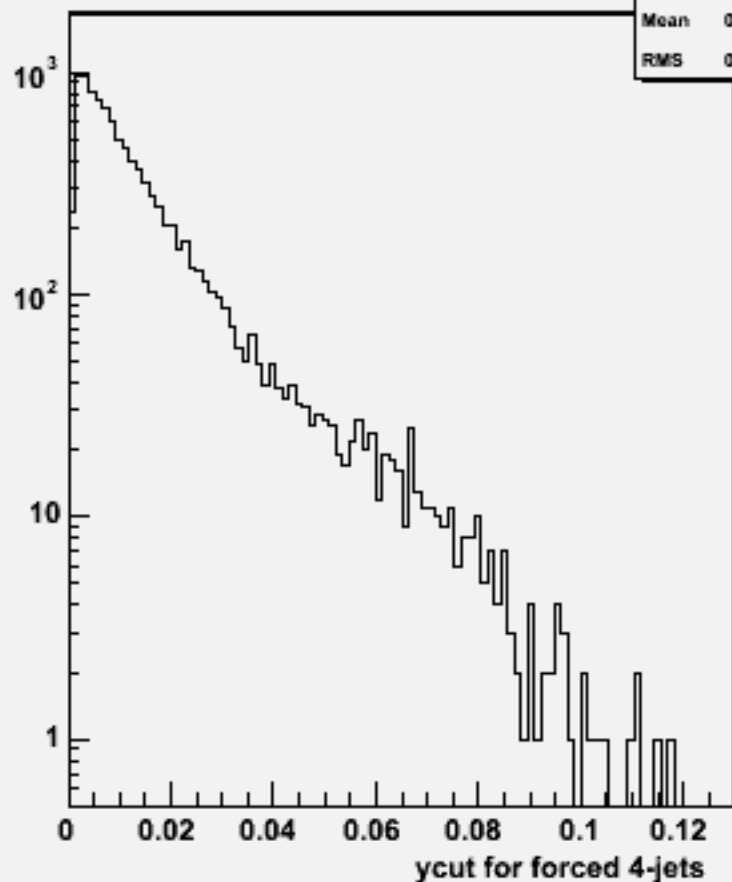
Ycut for 4-jets :w103558 ae1_n1ude1e1_o
