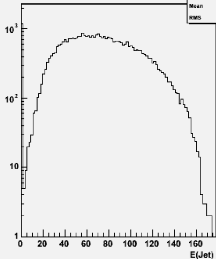
Jet energies(All jets)w103558 ae1_n1ude1e1_o
