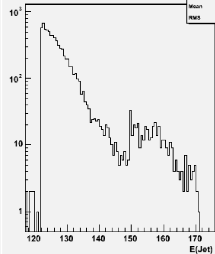
Jet energies(All jets)w103555 ae1_n1n3e3e1e1_o
