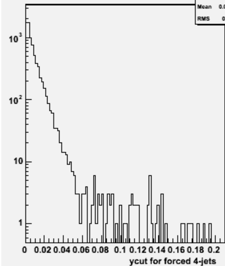
Ycut for 4-jets :w103555 ae1_n1n3e3e1e1_o
