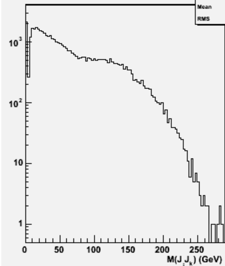
2jets mass(All comb)w103555 ae1_n1n3e3e1e1_o
