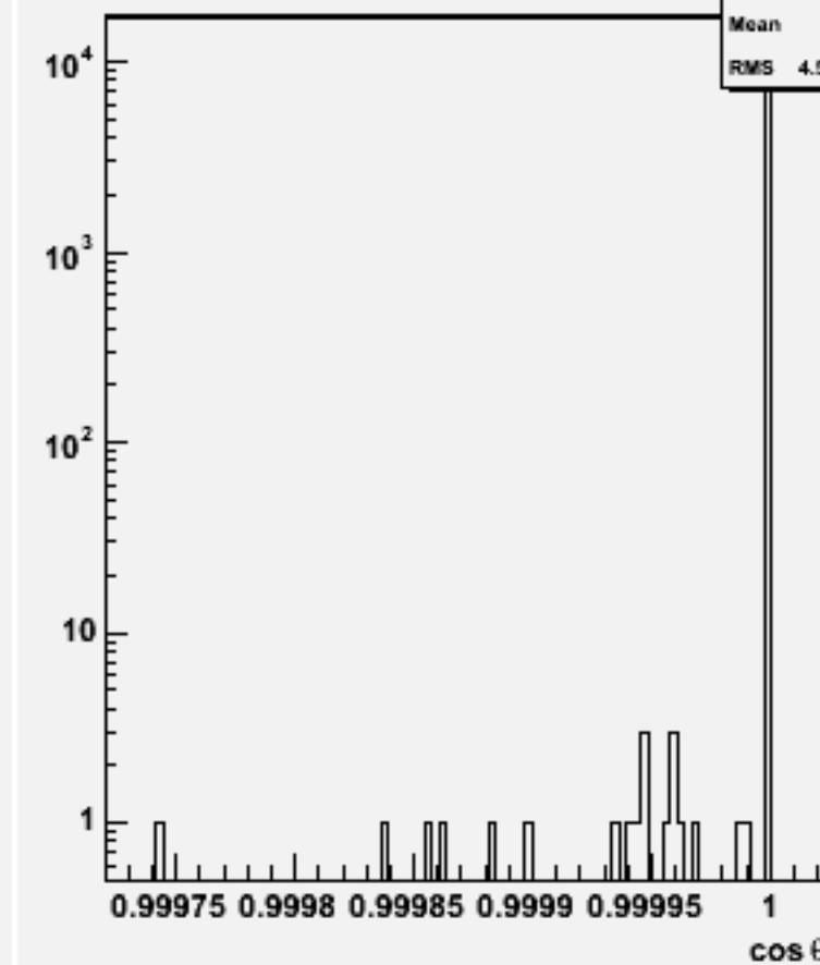
Jet cos \theta (All jets)w103555 ae1_n1n3e3e1e1_o
