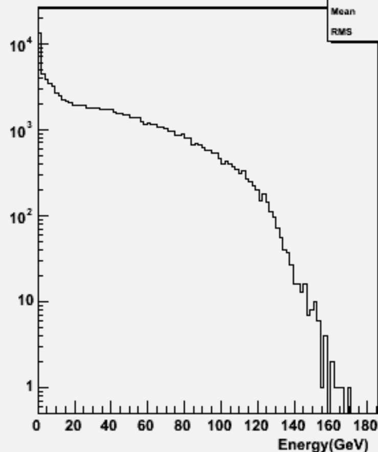
Start point R : w103554 ae1_n1n3e3e1e1_o
