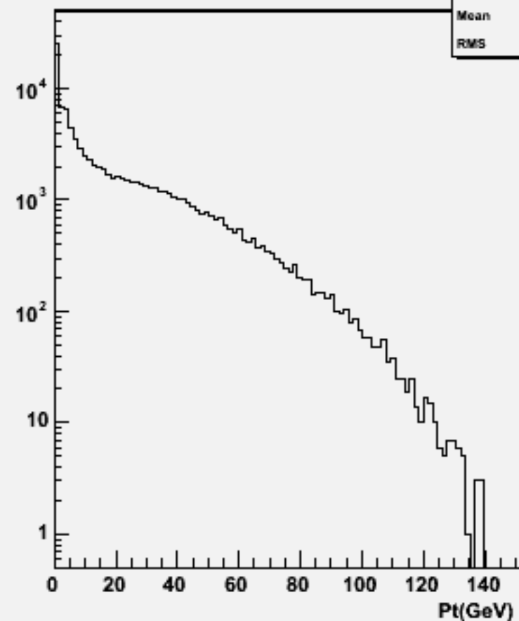
Start point Z : w103554 ae1_n1n3e3e1e1_o
