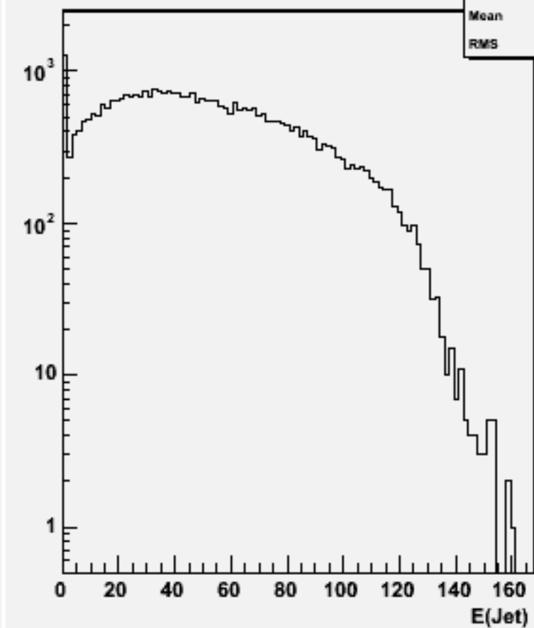
Jet energies(All jets)w103554 ae1_n1n3e3e1e1_o
