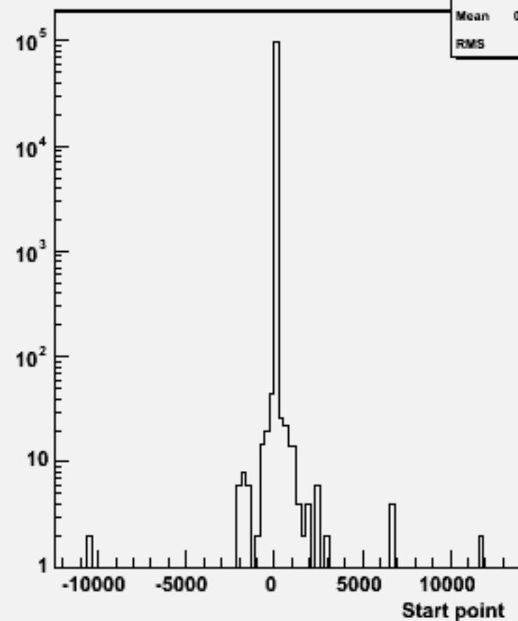
Start point Z : w103554 ae1_n1n3e3e1e1_o
