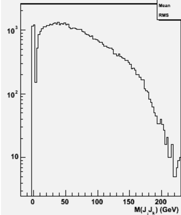
2jets mass(All comb)w103554 ae1_n1n3e3e1e1_o
