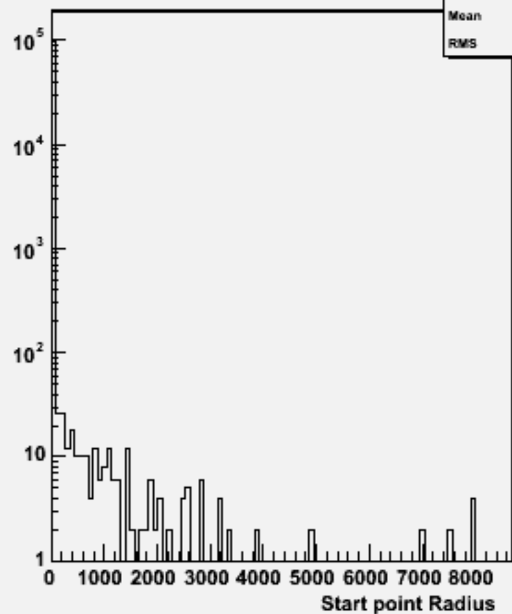
Start point R : w103554 ae1_n1n3e3e1e1_o
