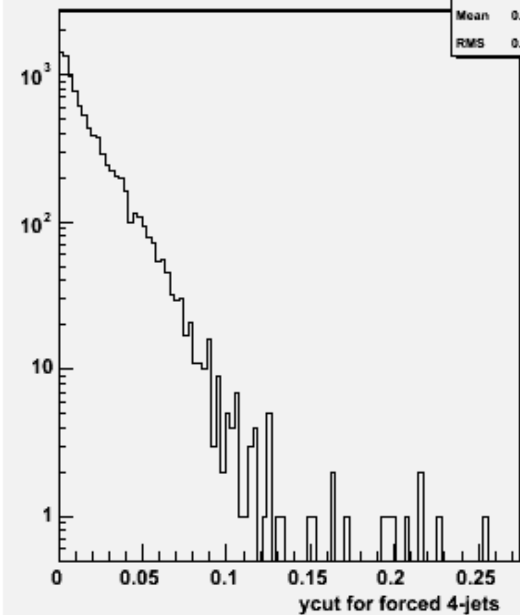
Ycut for 4-jets :w103554 ae1_n1n3e3e1e1_o
