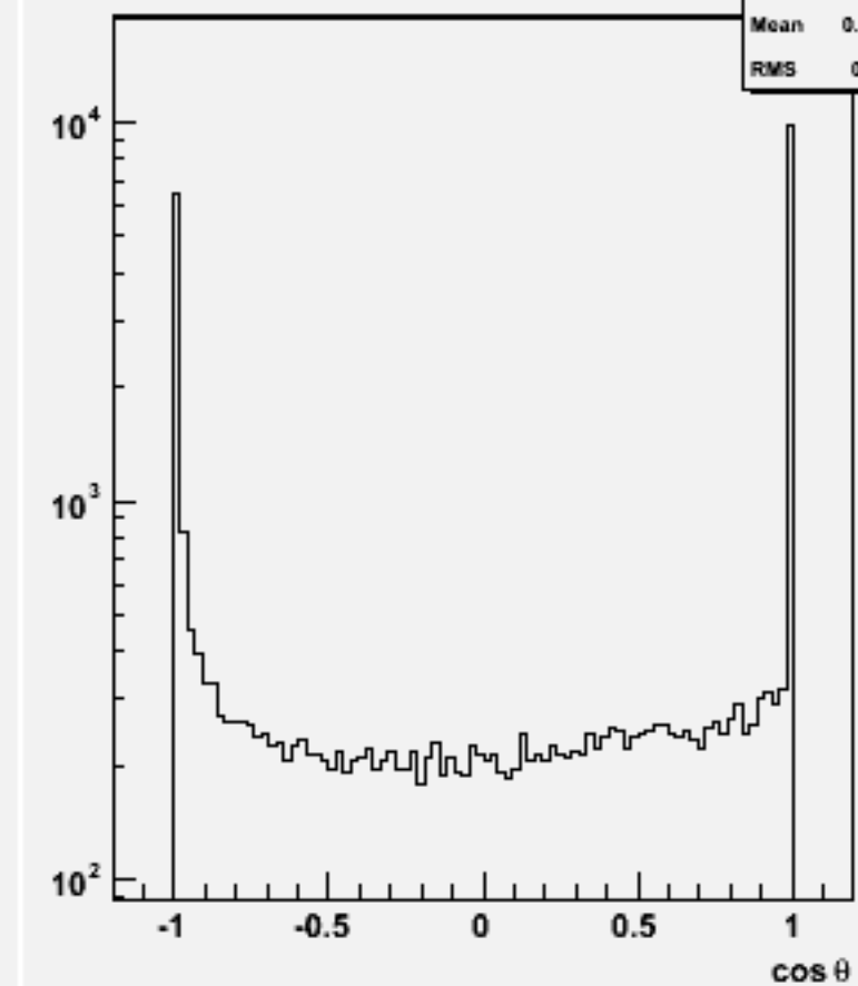
Jet cos \theta (All jets)w103554 ae1_n1n3e3e1e1_o
