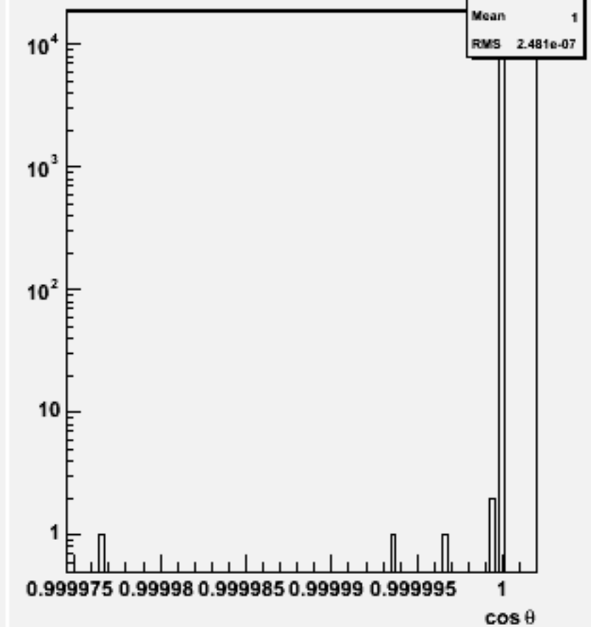
Jet cos θ (All jets)w103553 ae1_n1n3e3e1e1_o
