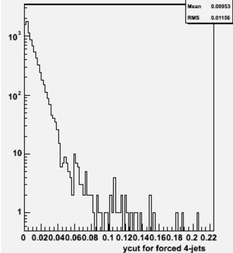
Ycut for 4-jets :w103553 ae1_n1n3e3e1e1_o
