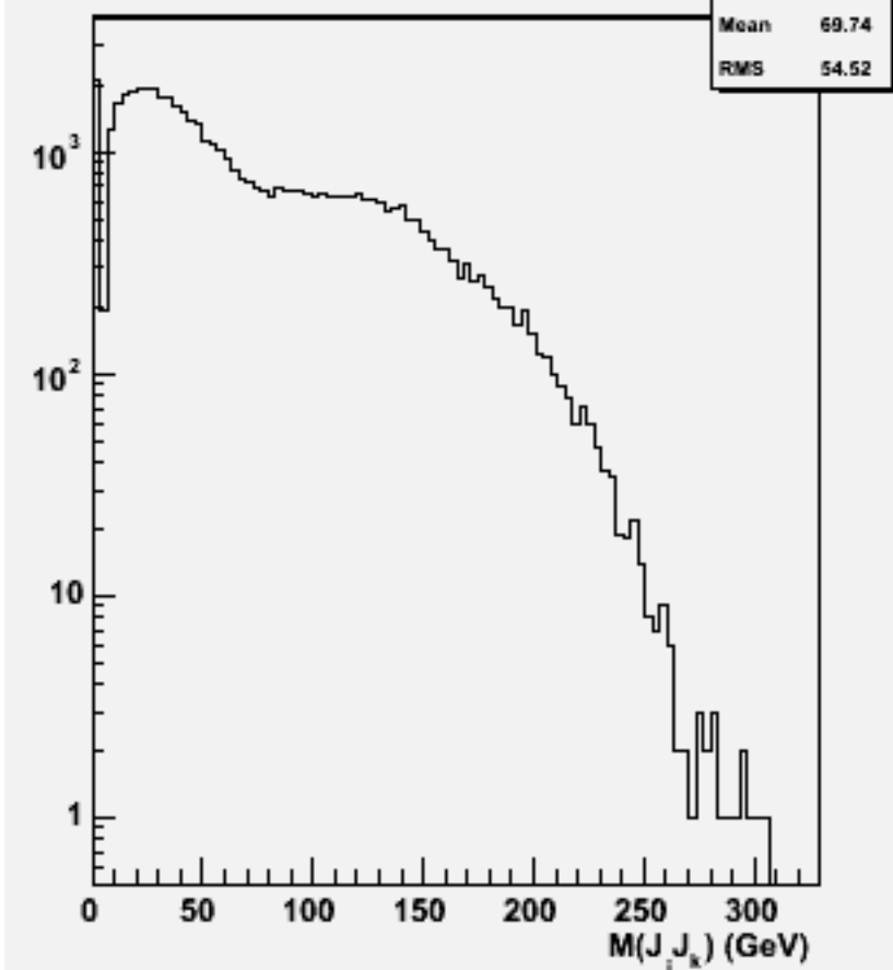
2jets mass(All comb)w103553 ae1_n1n3e3e1e1_o
