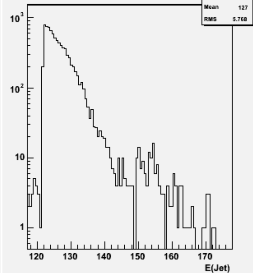
Jet energies(All jets)w103553 ae1_n1n3e3e1e1_o
