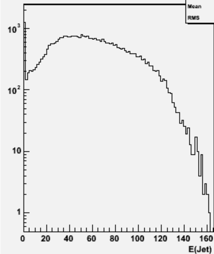
Jet energies(All jets)w103546 ae1_n1n1e1e1e1_o
