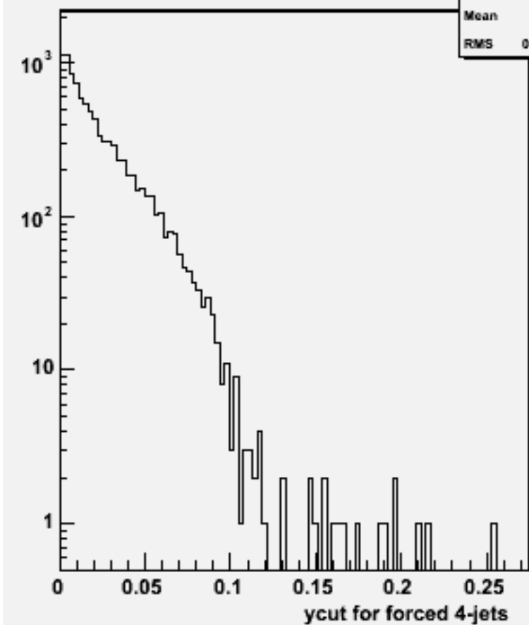
Ycut for 4-jets :w103546 ae1_n1n1e1e1e1_o
