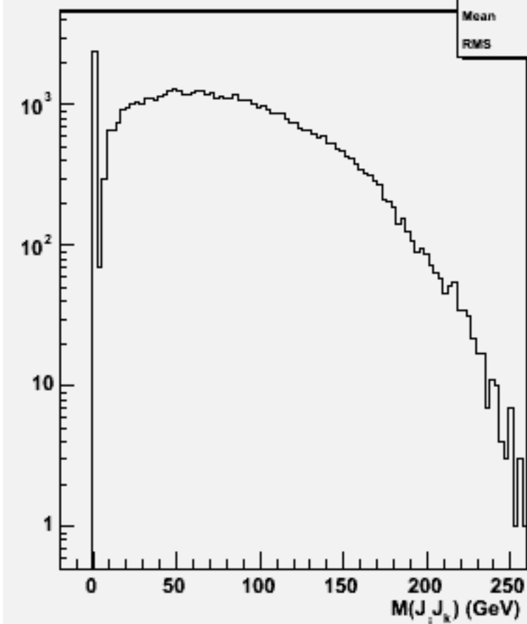
2jets mass(All comb)w103546 ae1_n1n1e1e1e1_o
