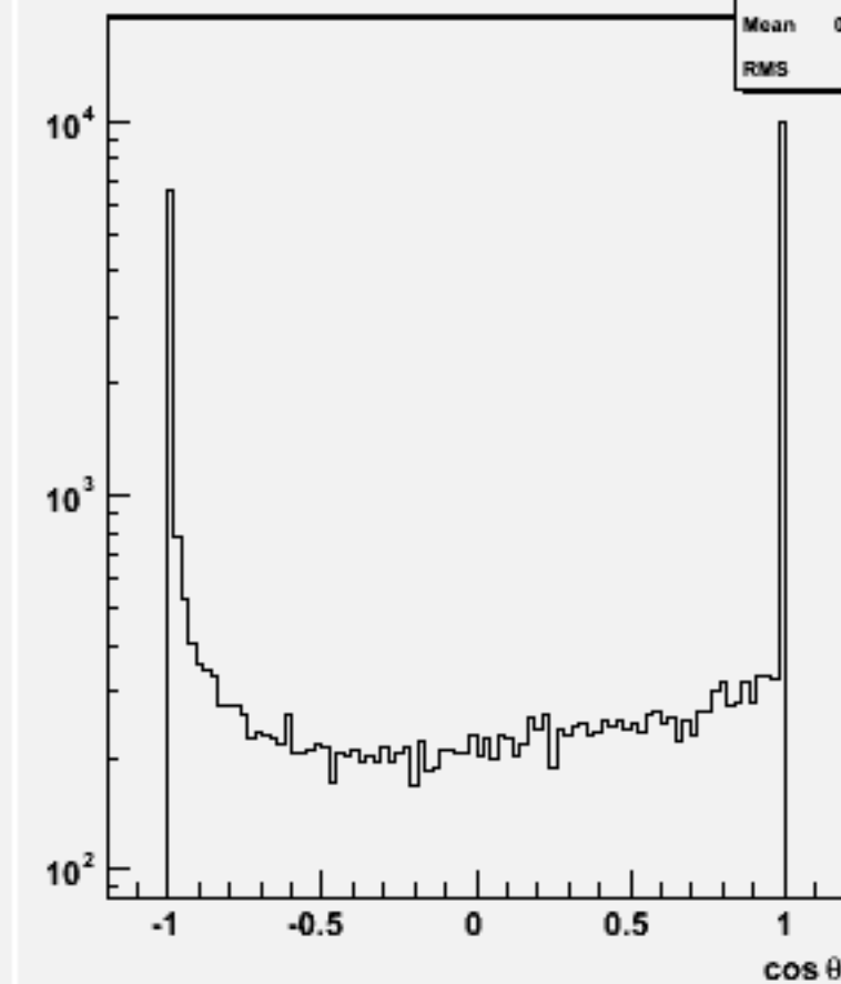
Jet cos \theta (All jets)w103546 ae1_n1n1e1e1e1_o
