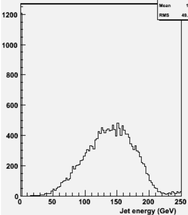
energy for 2-jets :w103542 ae1_n1csc_o
