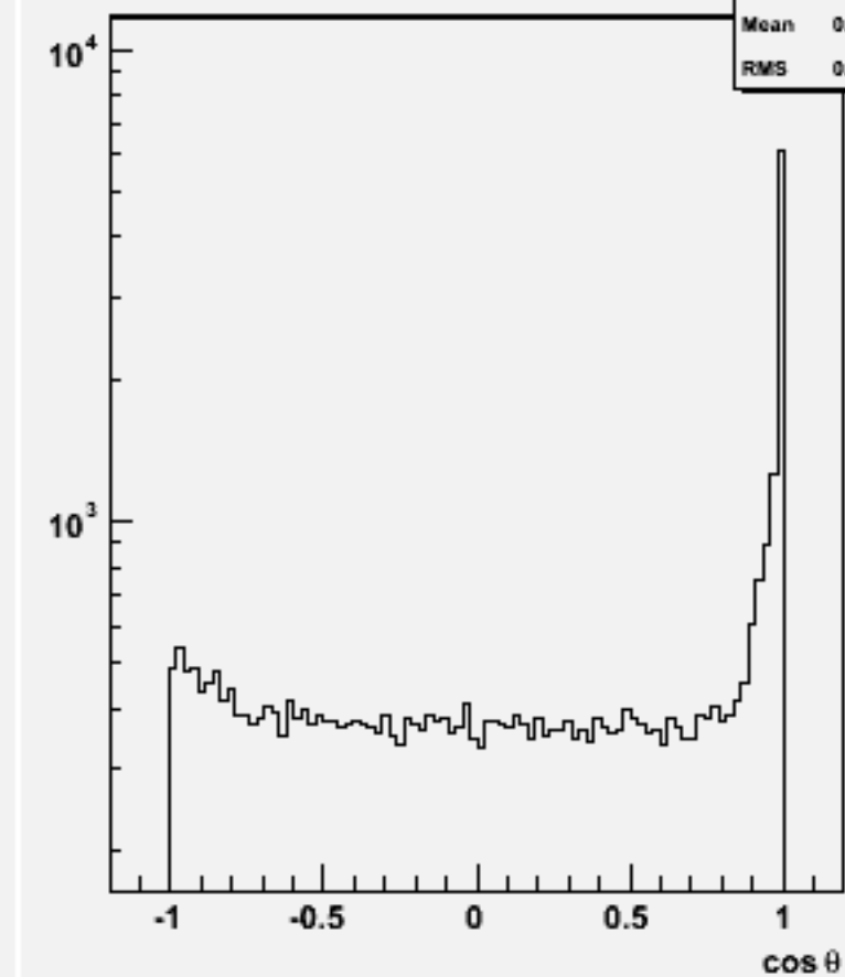
Jet cos \theta (All jets)w103542 ae1_n1csc_o
