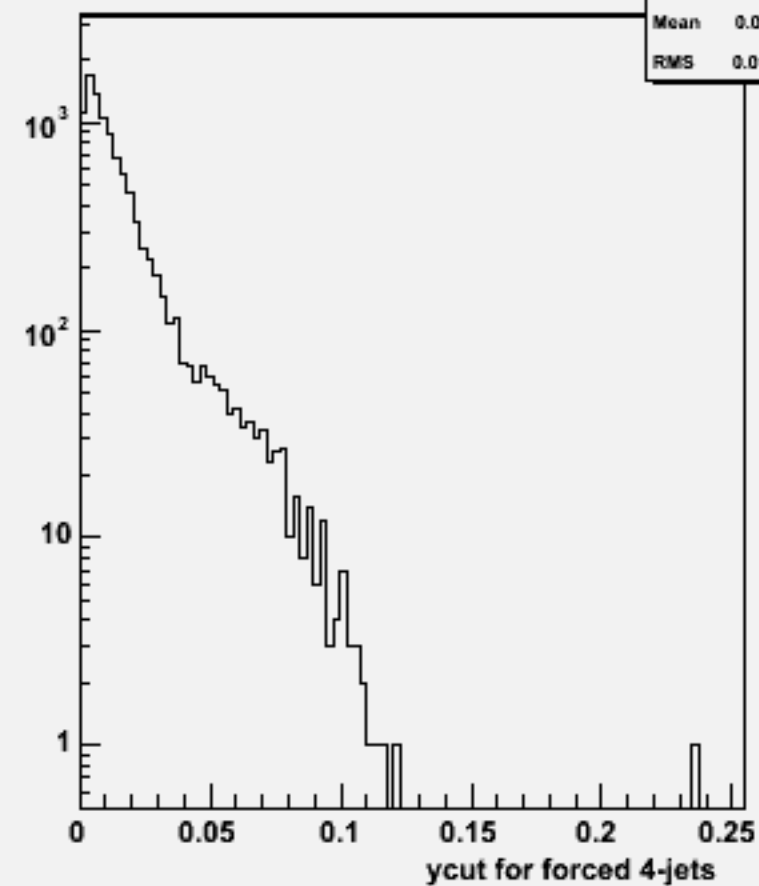
Ycut for 4-jets :w103542 ae1_n1csc_o
