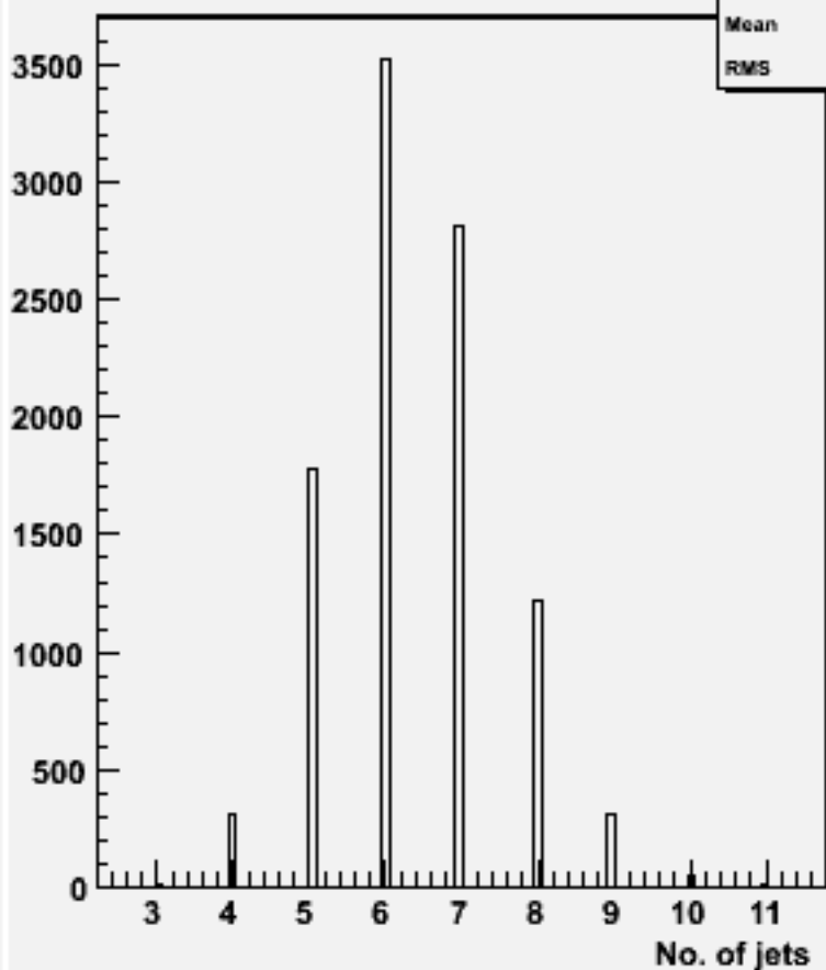
No. jets (ycut=0.001) : w103542 ae1_n1csc_o
