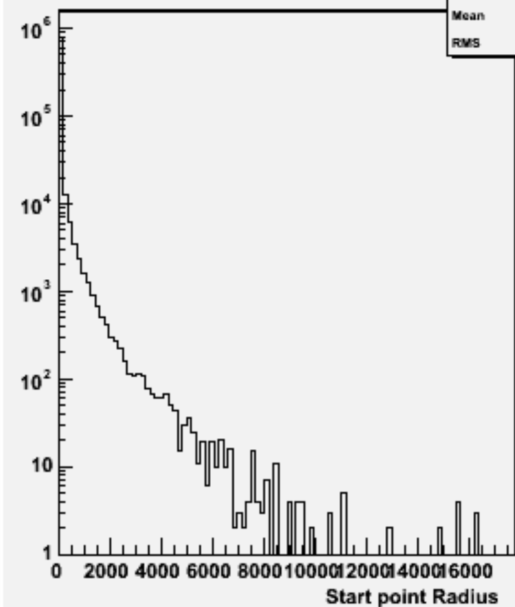
Start point R : w103542 ae1_n1csc_o
