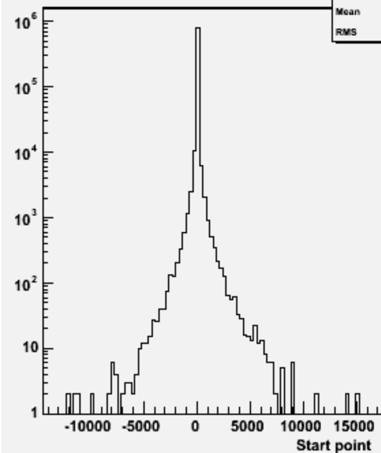
Start point Z : w103542 ae1_n1csc_o
