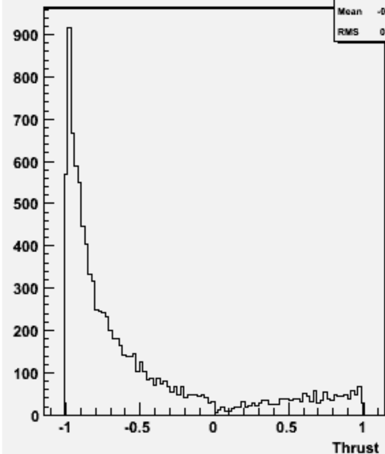
cos \Theta (thrust) w103542 ae1_n1csc_o
