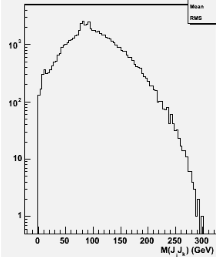
2jets mass(All comb)w103542 ae1_n1csc_o
