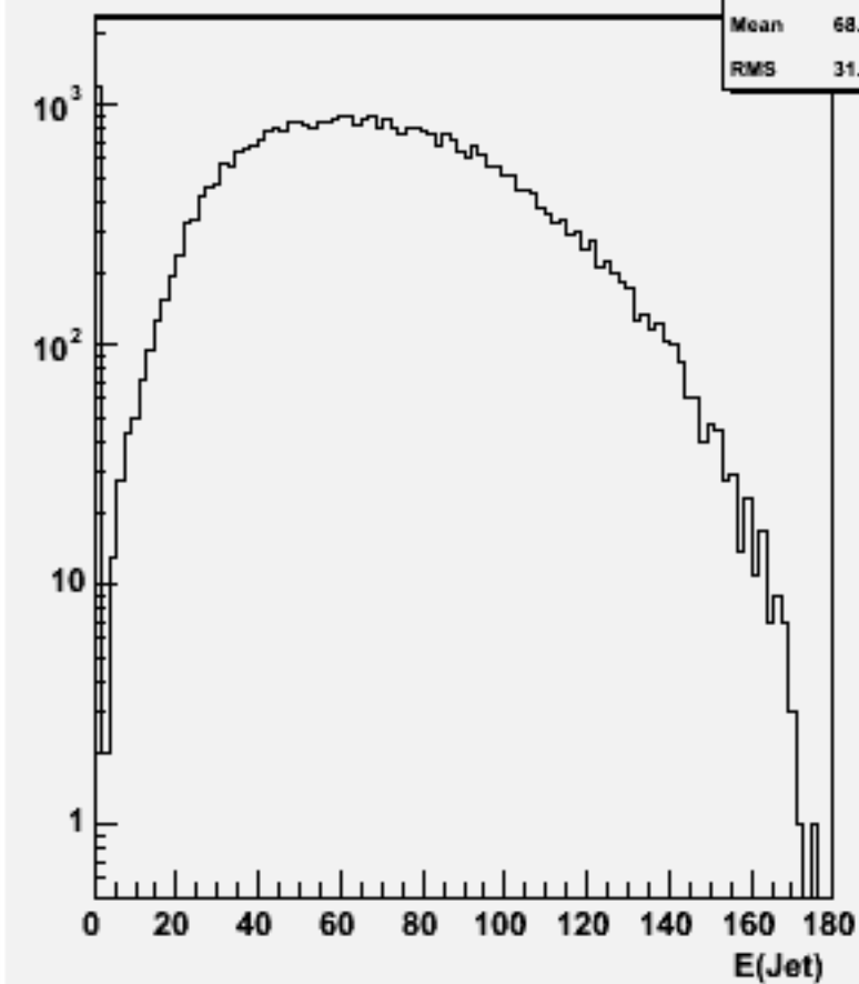
Jet energies(All jets)w103542 ae1_n1csc_o
