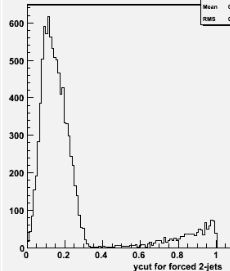
Ycut for 2-jets :w103542 ae1_n1csc_o
