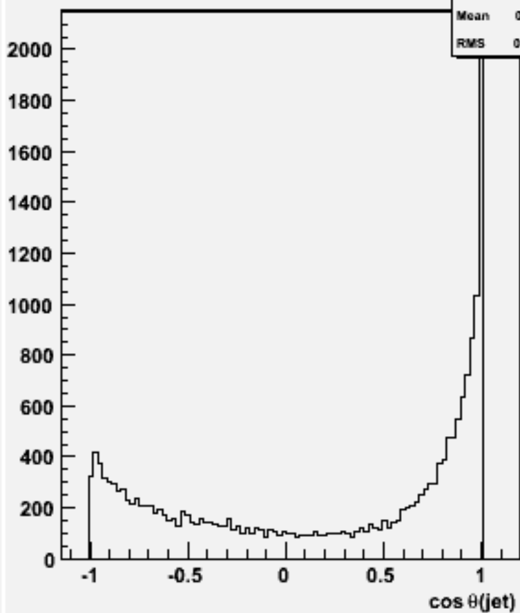
cos \theta for 2-jets :w103542 ae1_n1csc_o
