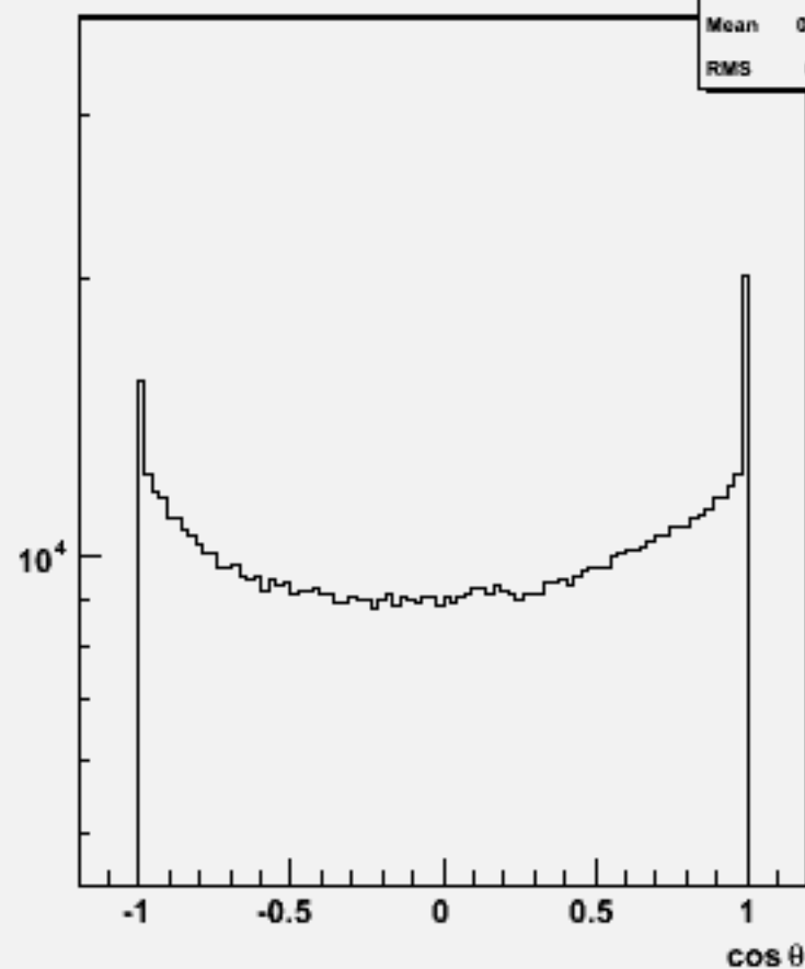
Particle cos \theta : w103542 ae1_n1csc_o
