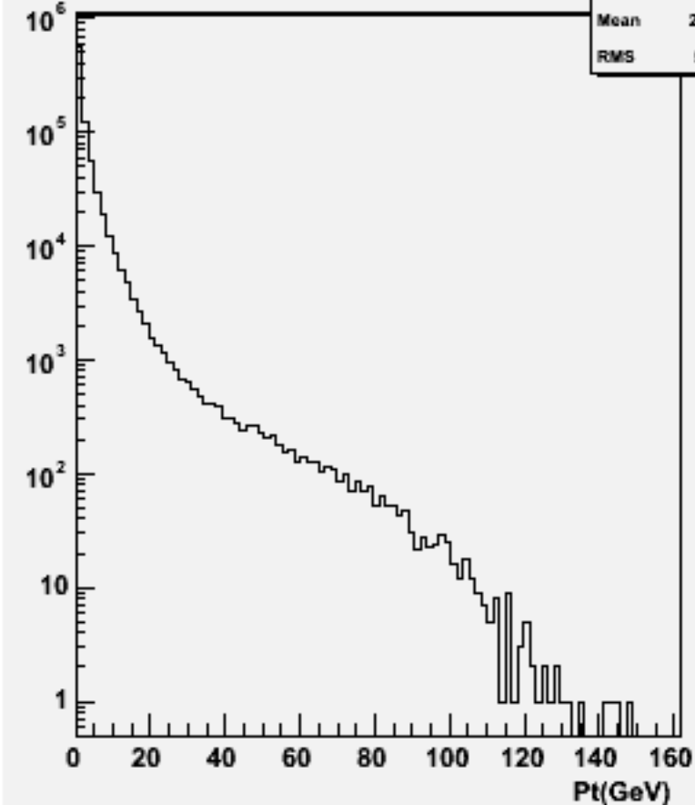
Particle Pt : w103542 ae1_n1csc_o
