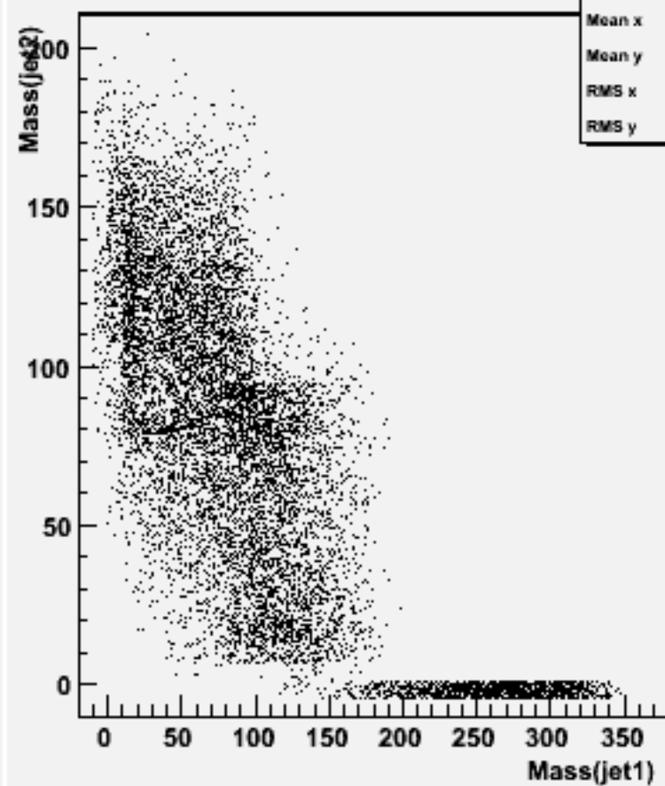
Jet mass for forced 2-jets : w103542 ae1_n1csc_o
