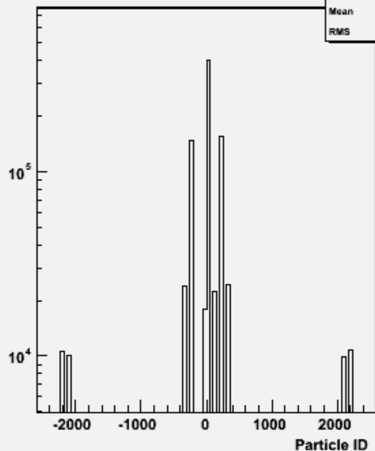
Particle ID : w103542 ae1_n1csc_o
