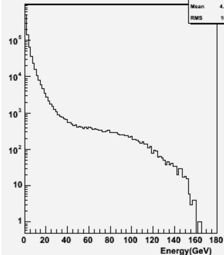
Particle Energy : w103542 ae1_n1csc_o
