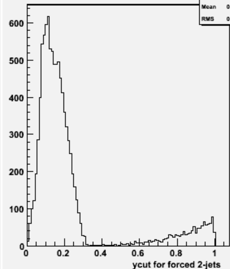
Ycut for 2-jets :w103538 ae1_n1udcc_o
