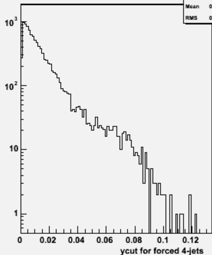
Ycut for 4-jets :w103538 ae1_n1udcc_o
