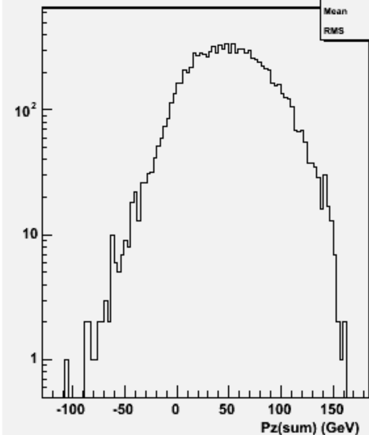
Pz Sum: w103538 ae1_n1udcc_o
