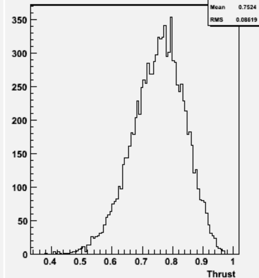
Thrust w103538 ae1_n1udcc_o
