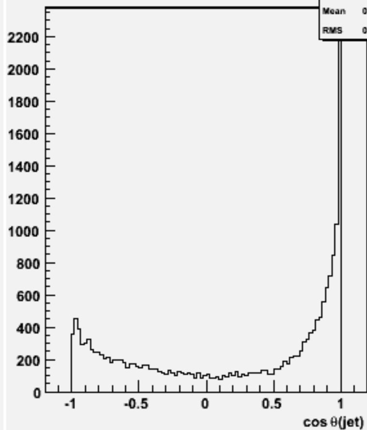
cos \Theta for 2-jets :w103538 ae1_n1udcc_o
