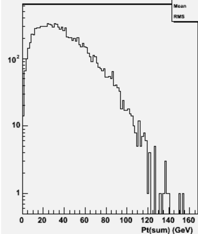
Pt Sum: w103538 ae1_n1udcc_o
