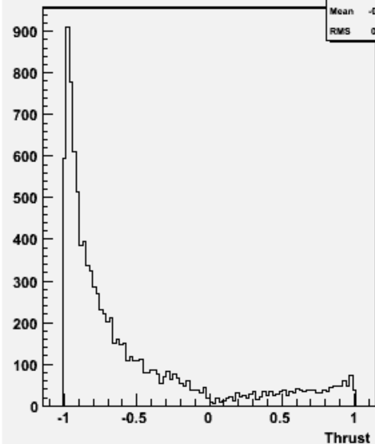
cos \Theta (thrust) w103538 ae1_n1udcc_o
