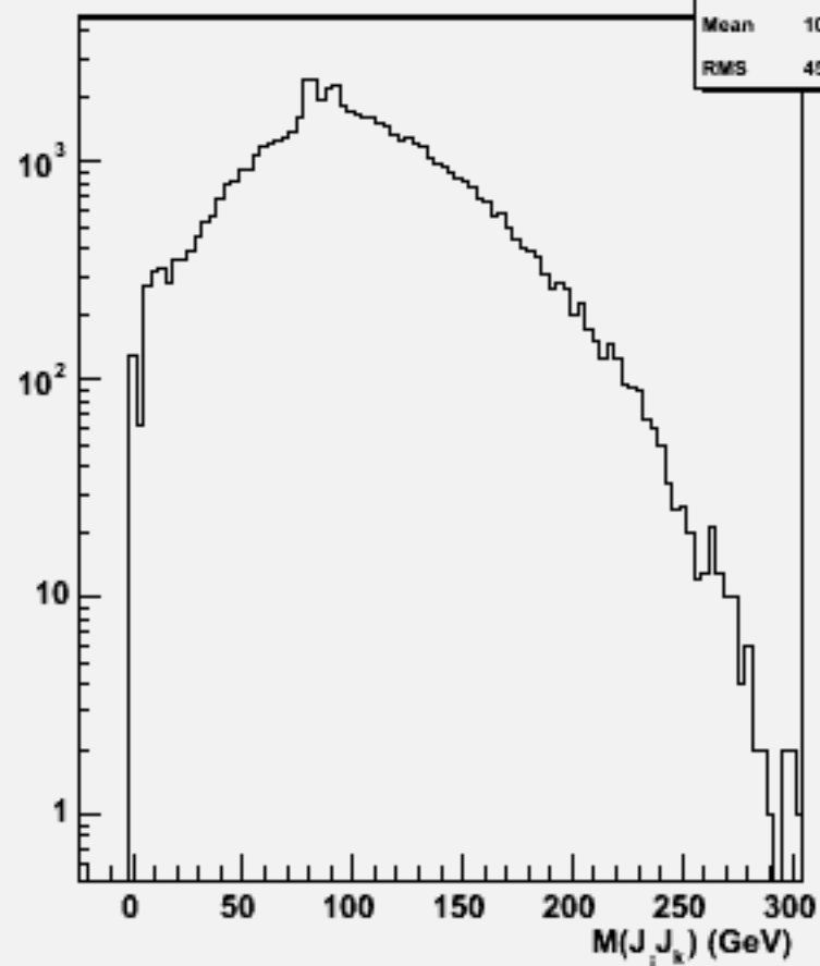
2jets mass(All comb)w103538 ae1_n1udcc_o
