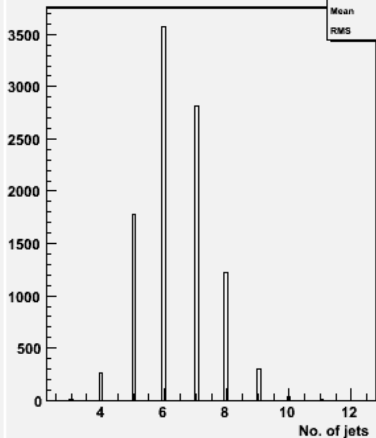
No. jets (ycut=0.001) : w103538 ae1_n1udcc_o
