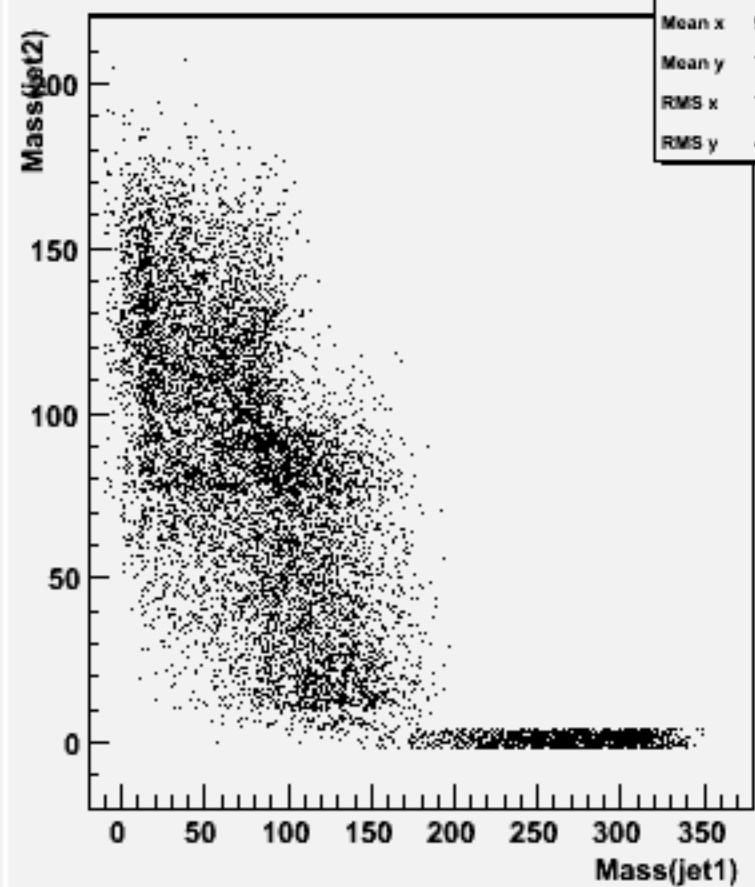
Jet mass for forced 2-jets : w103538 ae1_n1udcc_o
