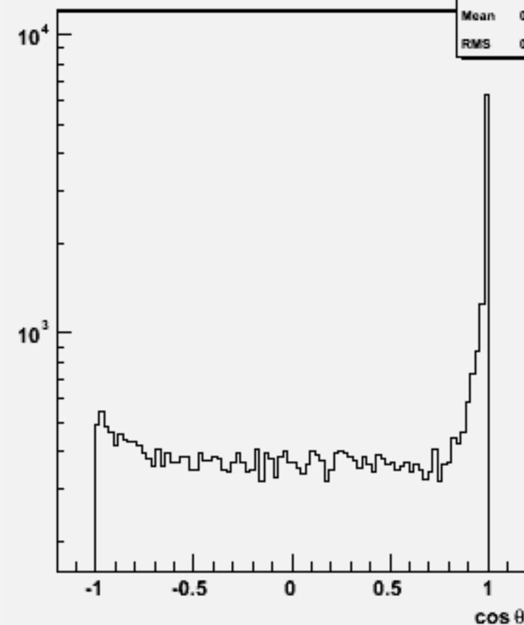
Jet cos \theta (All jets)w103538 ae1_n1udcc_o
