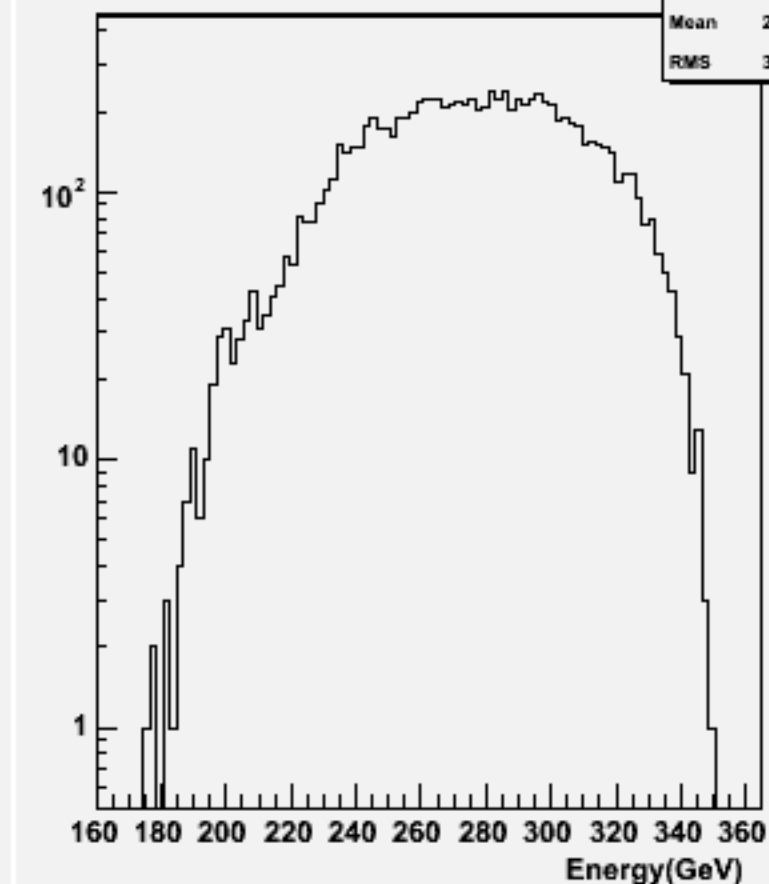
Thrust w103538 ae1_n1udcc_o
