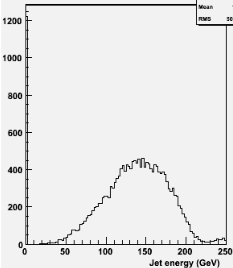
energy for 2-jets :w103538 ae1_n1udcc_o
