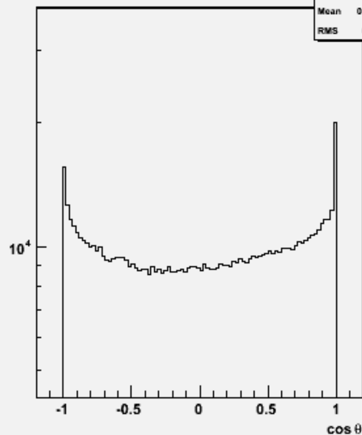
Particle cosθ : w103538 ae1_n1udcc_o
