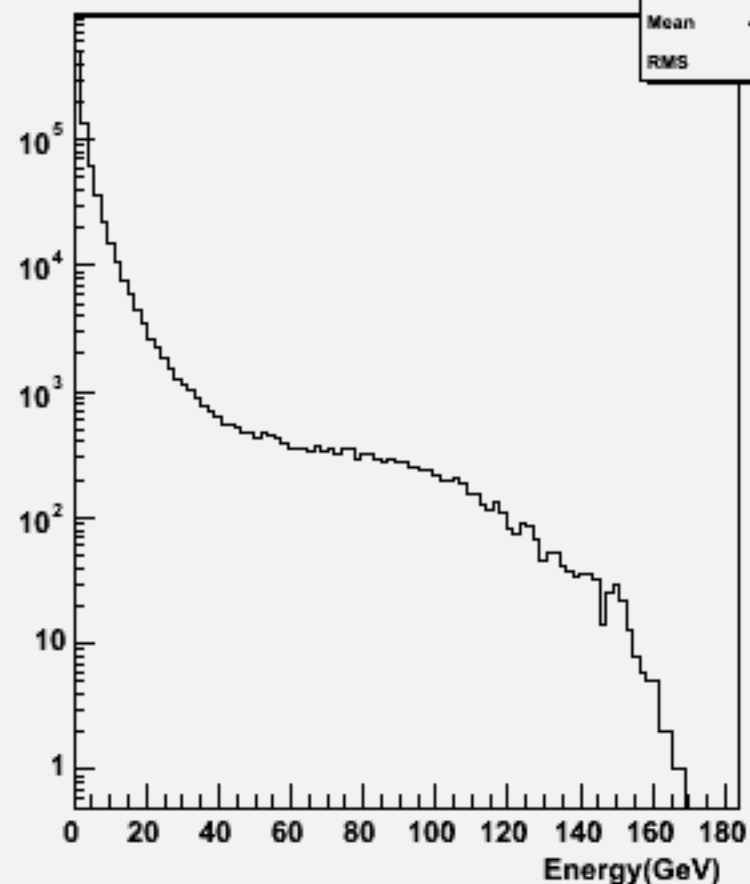
Particle Energy : w103538 ae1_n1udcc_o
