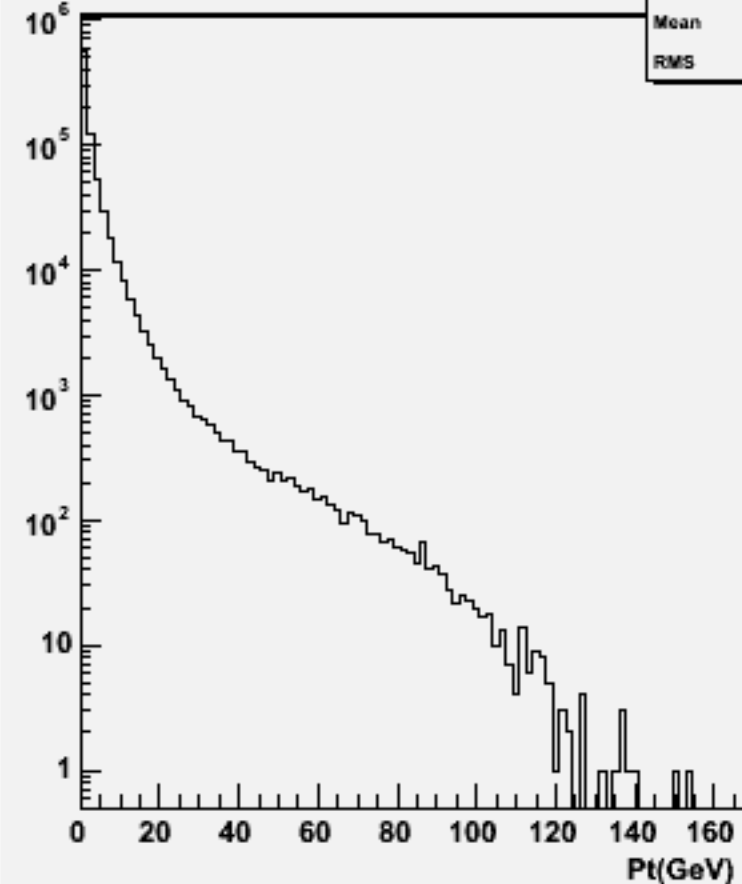
Particle Pt : w103538 ae1_n1udcc_o
