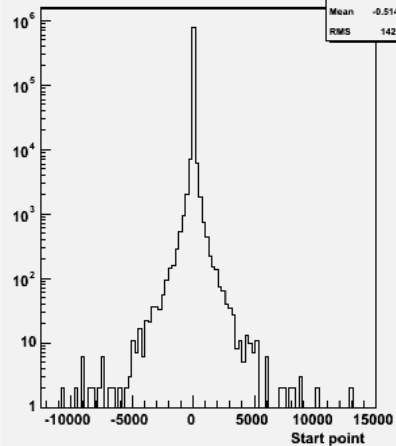
Start point Z : w103538 ae1_n1udcc_o
