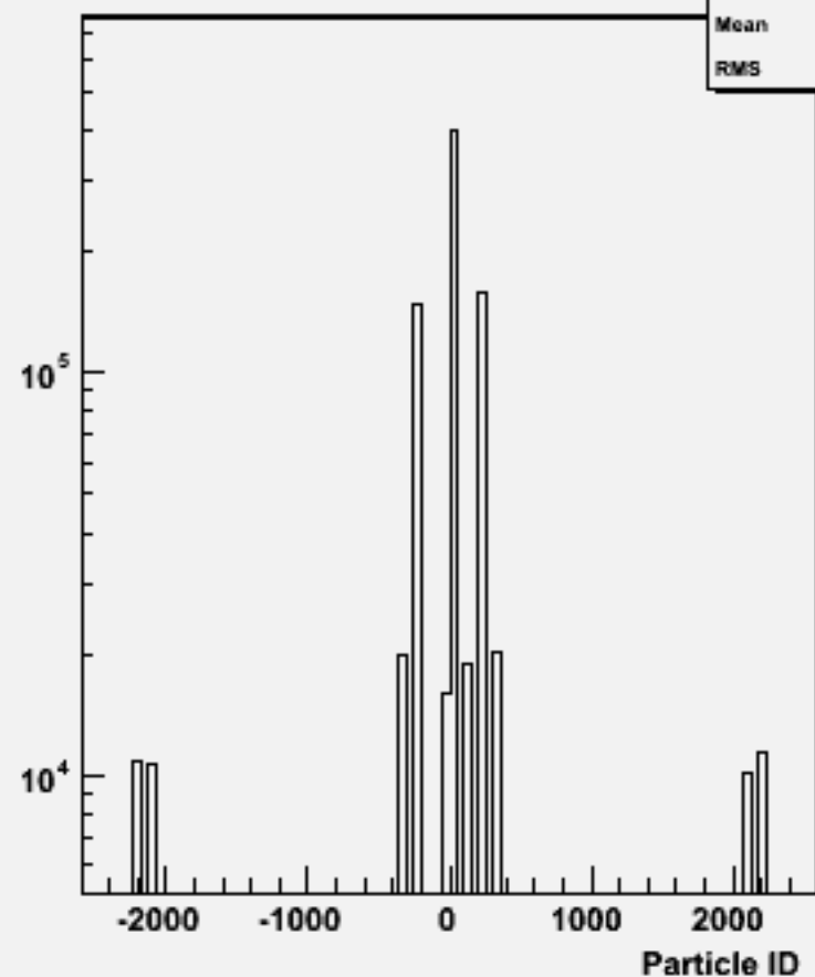
Particle ID : w103538 ae1_n1udcc_o
