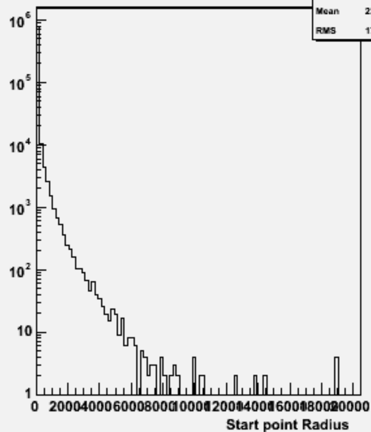
Start point R : w103538 ae1_n1udcc_o
