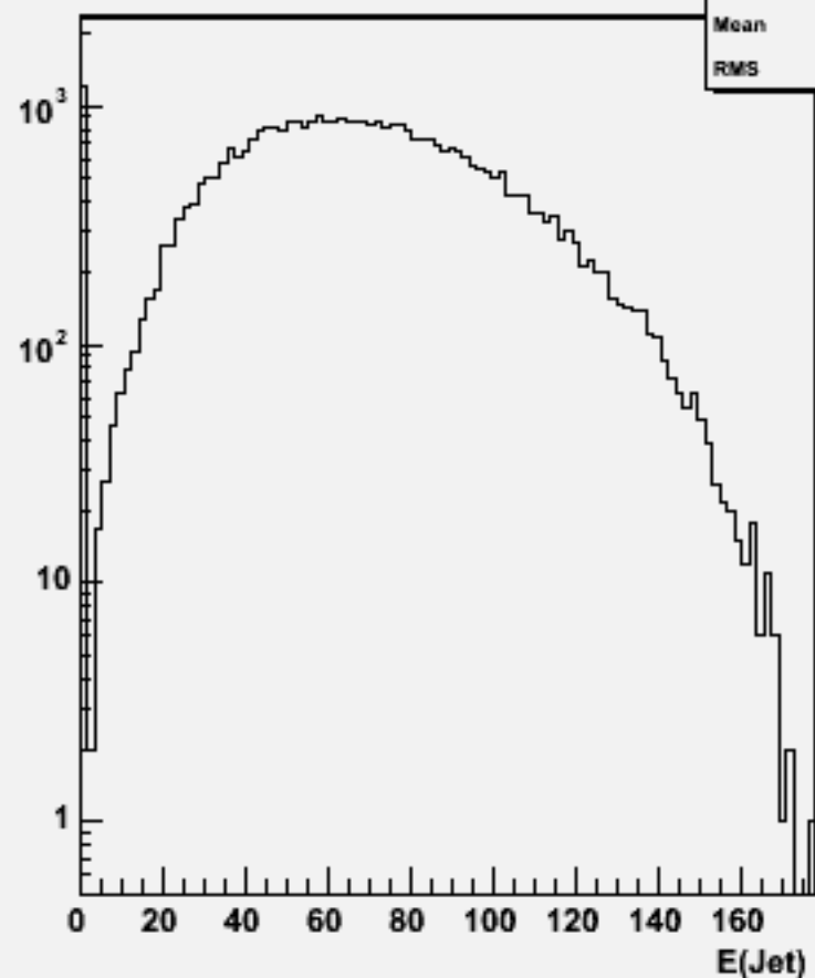
Jet energies(All jets)w103538 ae1_n1udcc_o
