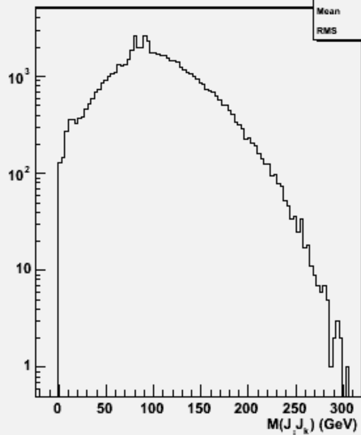
2jets mass(All comb)w103522 ae1_n1csuu_o
