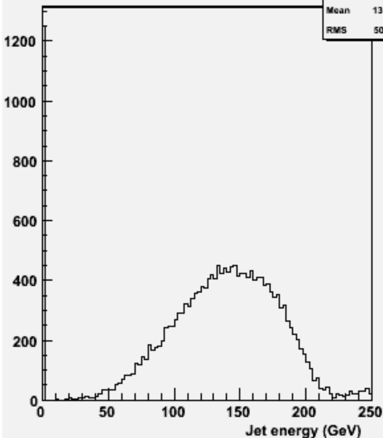
energy for 2-jets :w103522 ae1_n1csuu_o
