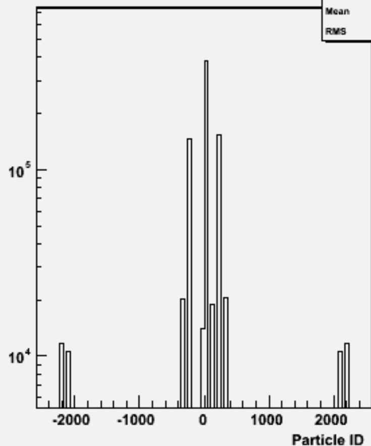
Particle ID : w103522 ae1_n1csuu_o
