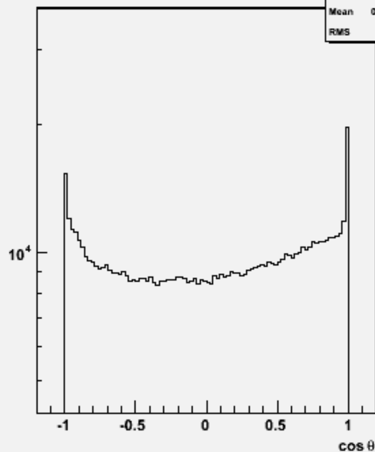
Particle \cos\theta : w103522 ae1_n1csuu_o
