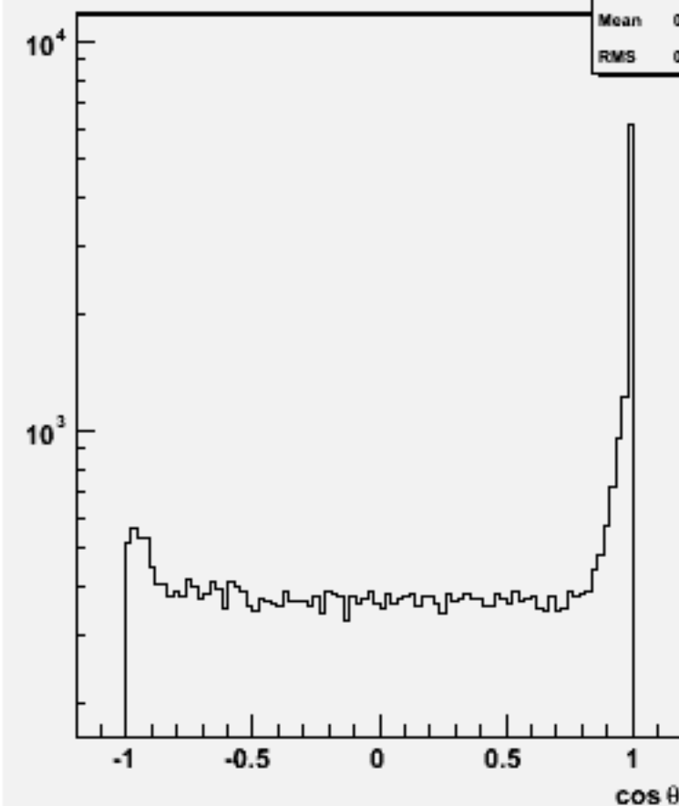
Jet cos \theta (All jets)w103522 ae1_n1csuu_o
