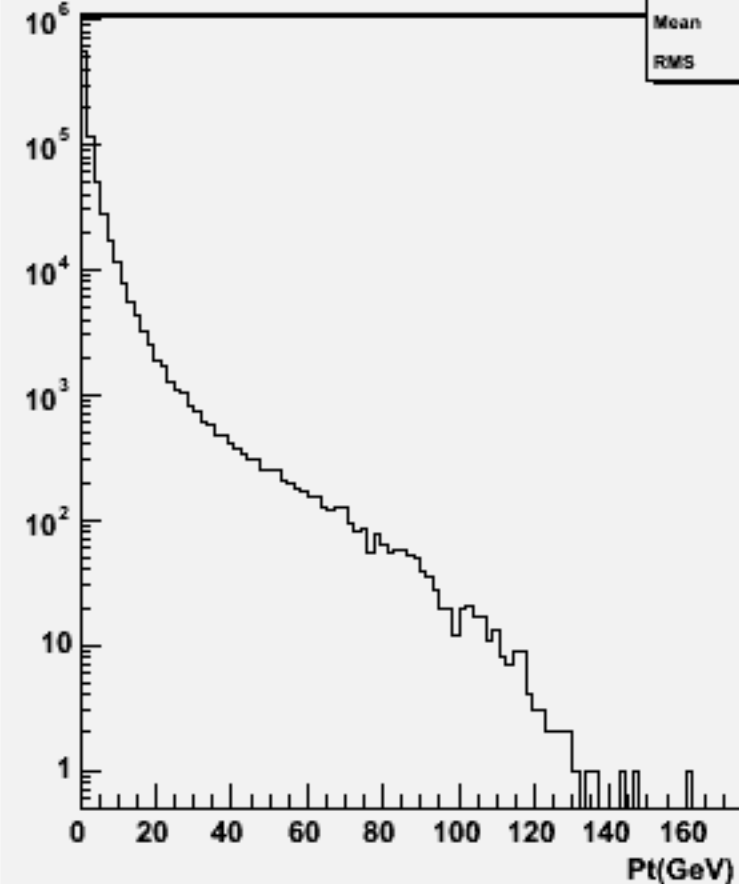
Particle Pt : w103522 ae1_n1csuu_o
