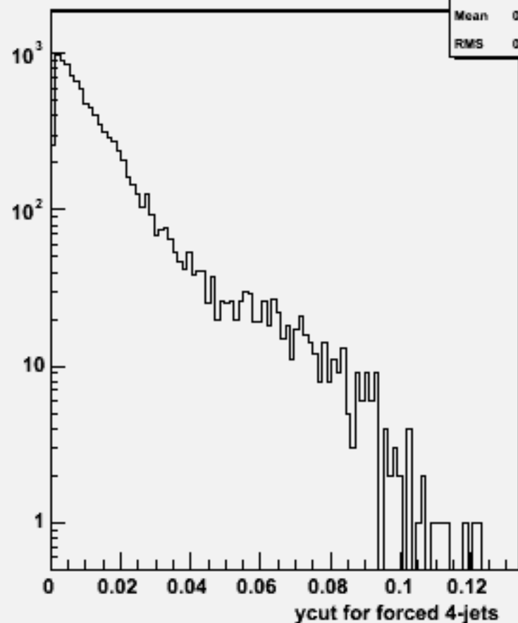
Ycut for 4-jets :w103522 ae1_n1csuu_o
