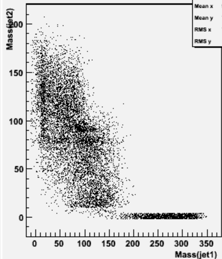
Jet mass for forced 2-jets : w103522 ae1_n1csuu_o
