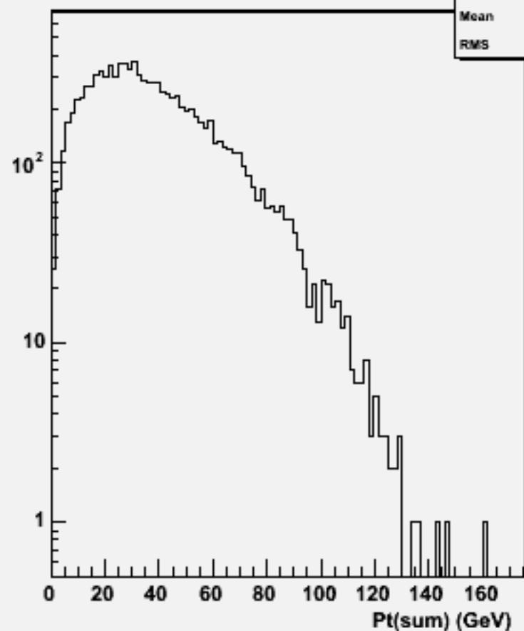
Pt Sum: w103522 ae1_n1csuu_o
