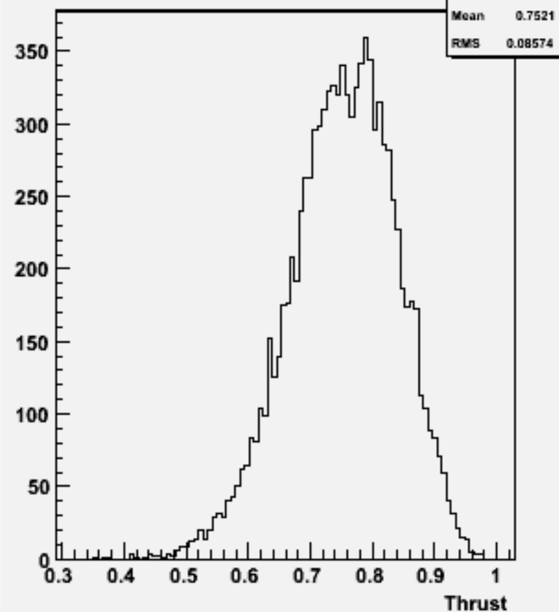
Thrust w103522 ae1_n1csuu_o
