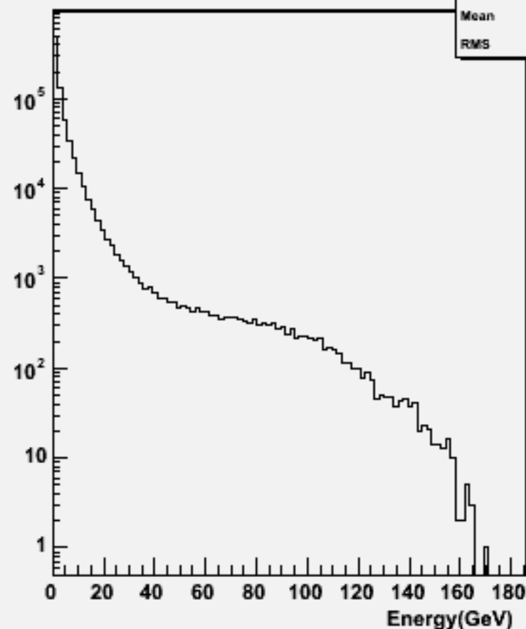
Particle Energy : w103522 ae1_n1csuu_o
