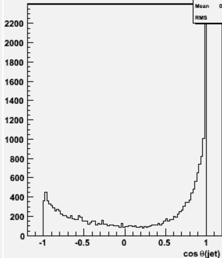
cos \Theta for 2-jets :w103522 ae1_n1csuu_o
