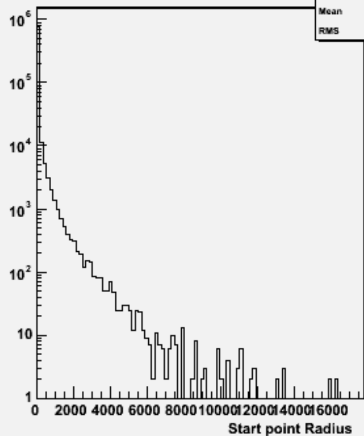
Start point R : w103522 ae1_n1csuu_o
