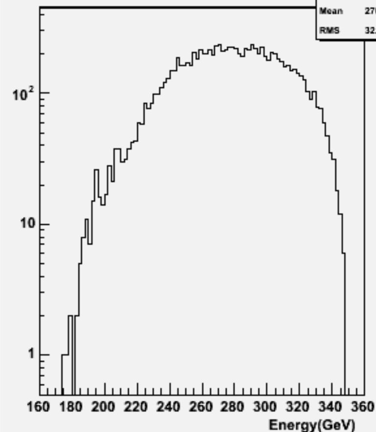
Thrust w103522 ae1_n1csuu_o
