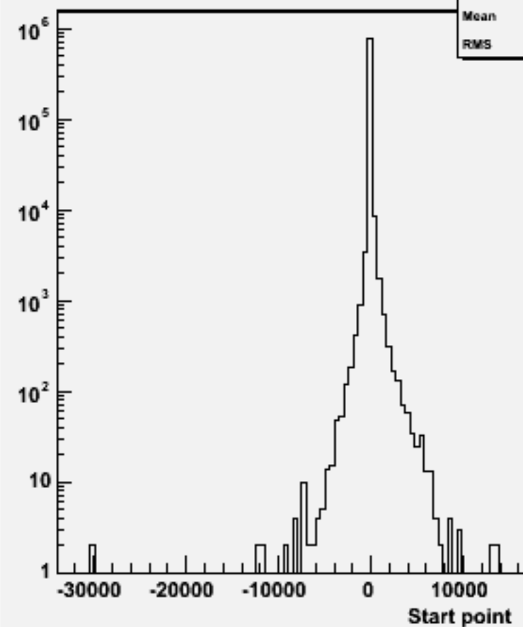
Start point Z : w103522 ae1_n1csuu_o
