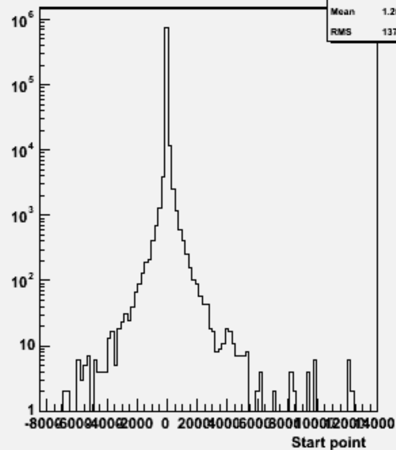
Start point Z : w103518 ae1_n1uduu_o
