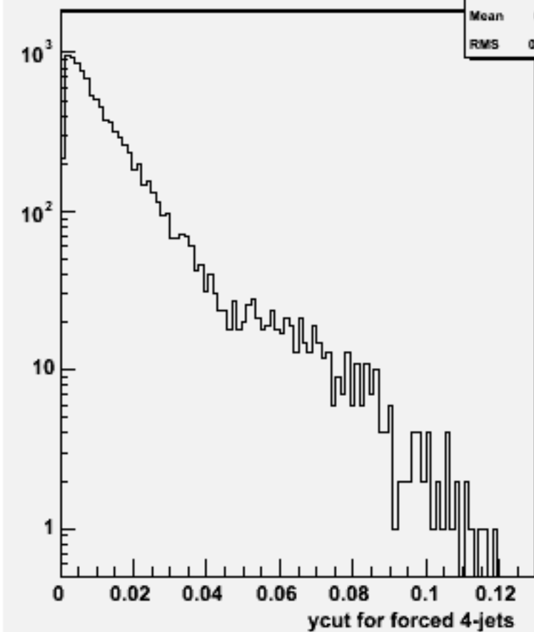
Ycut for 4-jets :w103518 ae1_n1uduu_o
