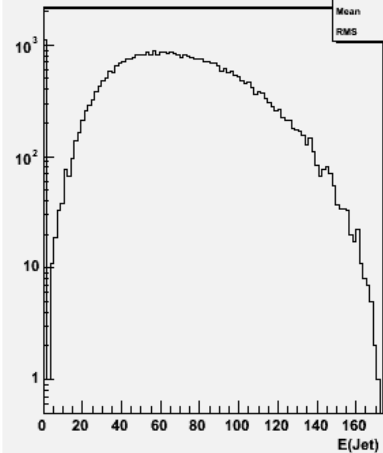
Jet energies(All jets)w103518 ae1_n1uduu_o
