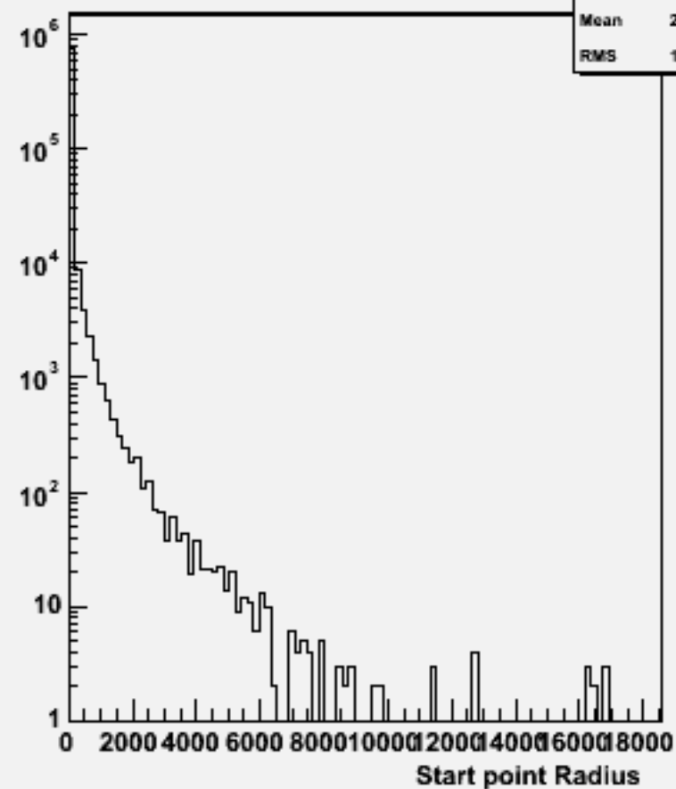
Start point R : w103518 ae1_n1uduu_o
