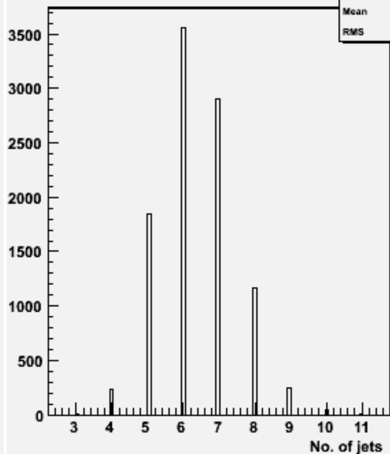
No. jets (ycut=0.001) : w103518 ae1_n1uduu_o
