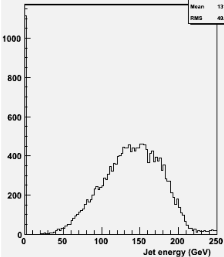
energy for 2-jets :w103518 ae1_n1uduu_o
