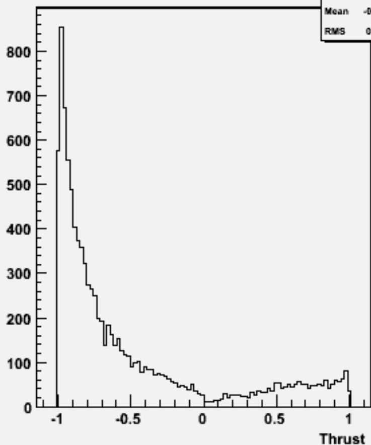
cos \Theta (thrust) w103518 ae1_n1uduu_o
