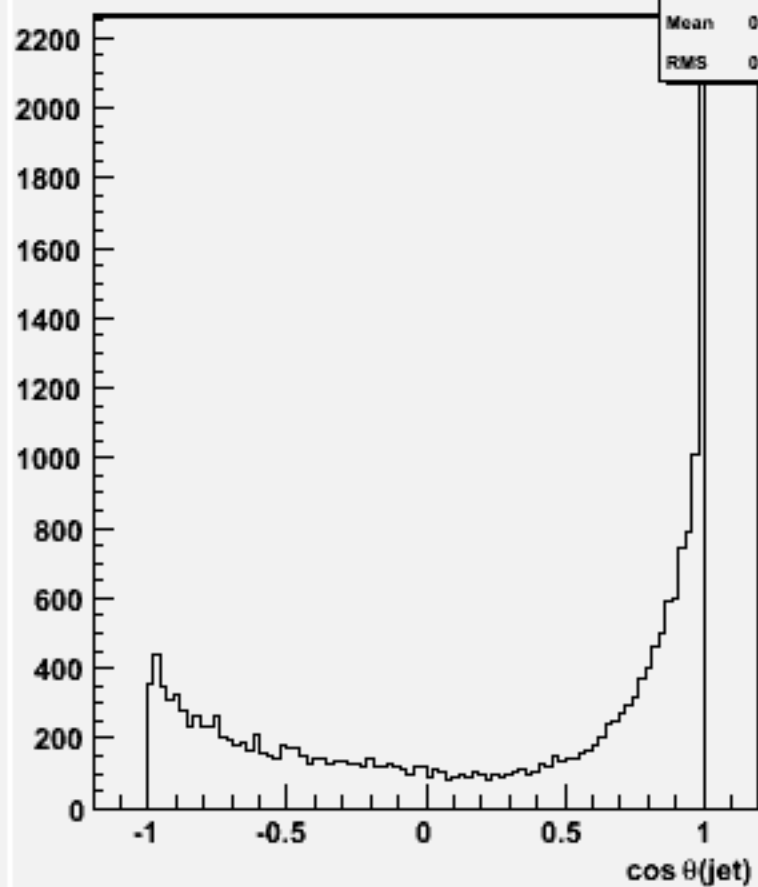
cos \theta for 2-jets :w103518 ae1_n1uduu_o
