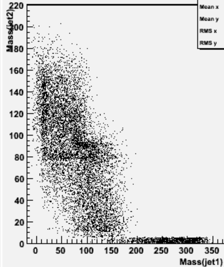
Jet mass for forced 2-jets : w103518 ae1_n1uduu_o
