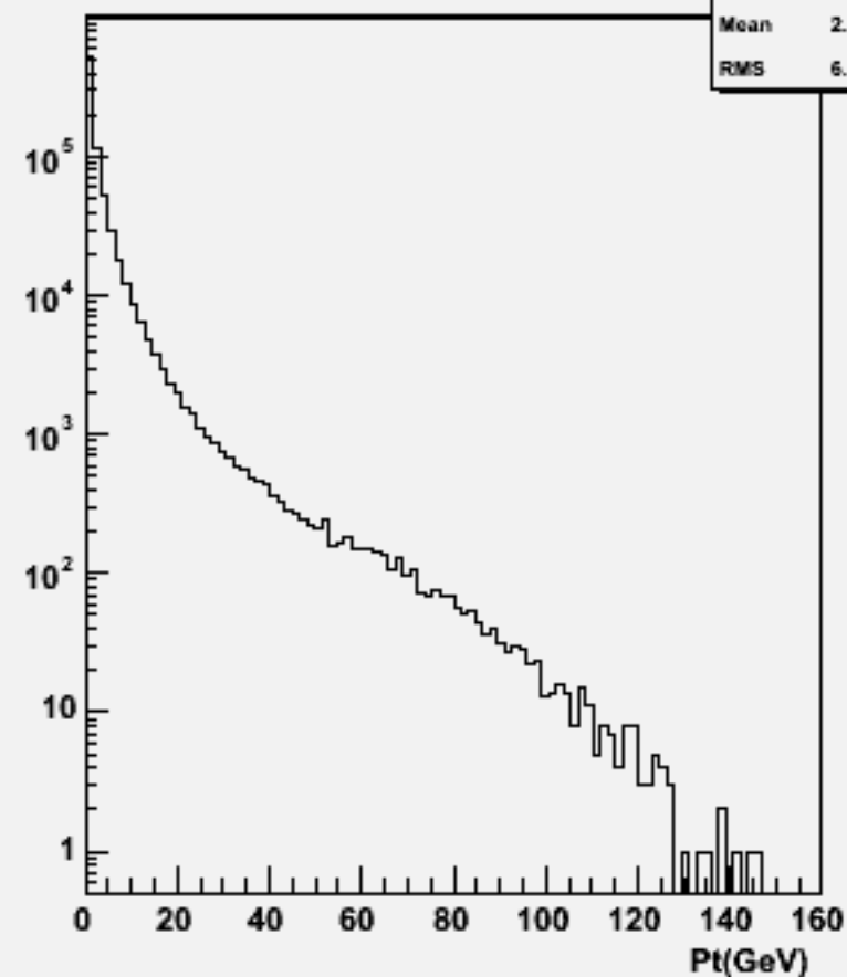
Start point Z : w103518 ae1_n1uduu_o
