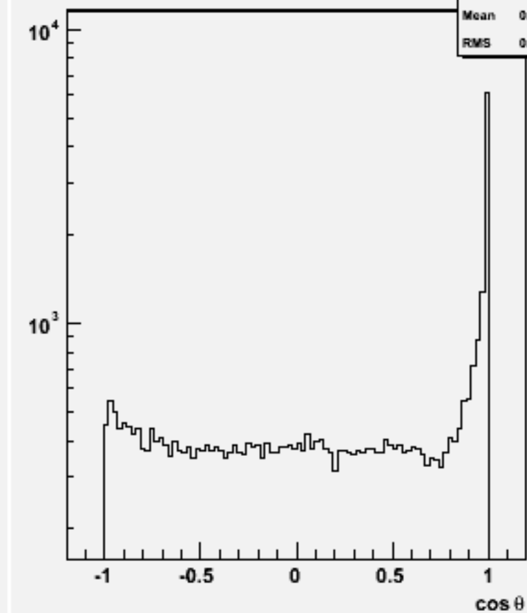
Jet cos \theta (All jets)w103518 ae1_n1uduu_o
