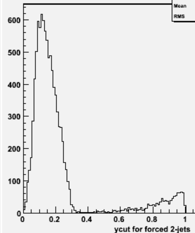
Ycut for 2-jets :w103518 ae1_n1uduu_o
