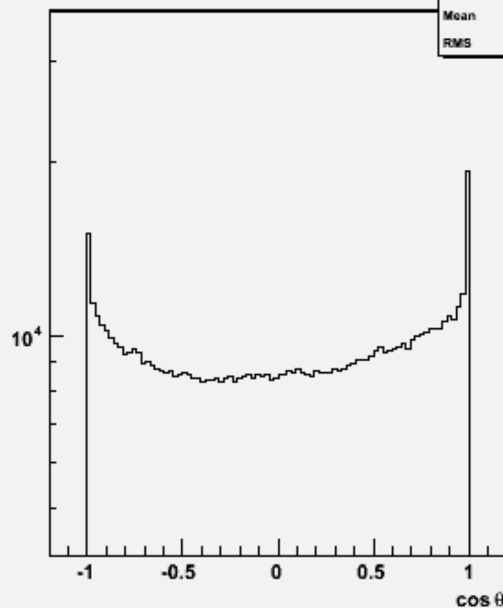
Particle cos \theta : w103518 ae1_n1uduu_o
