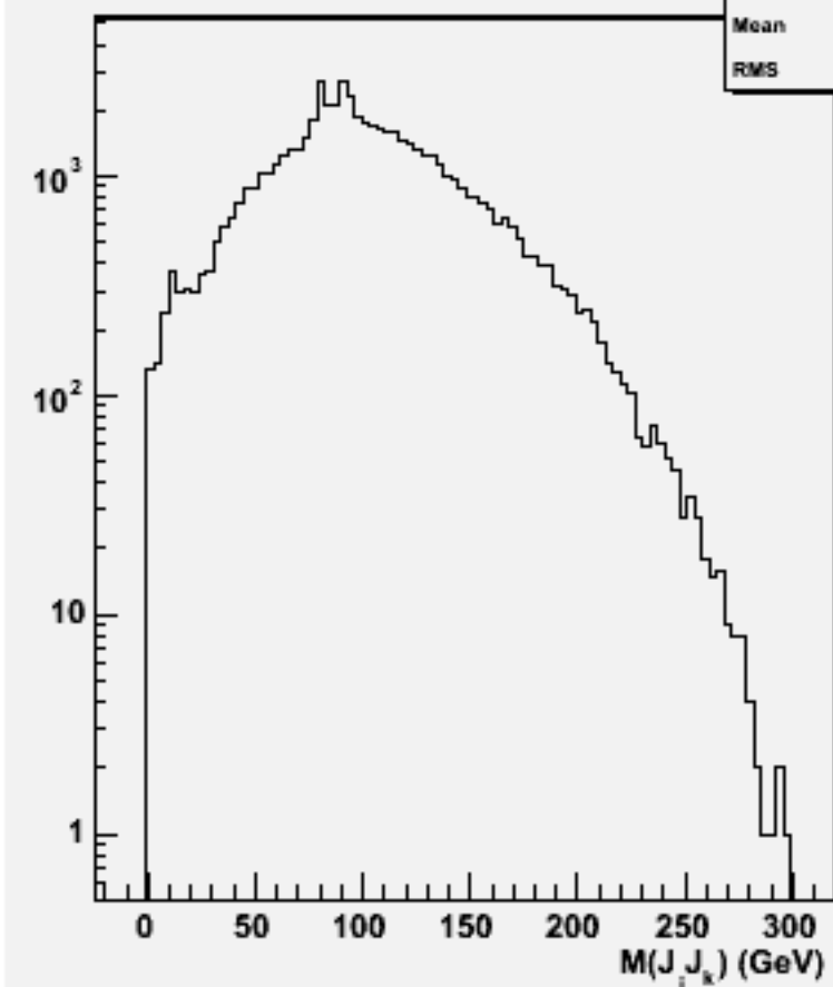
2jets mass(All comb)w103518 ae1_n1uduu_o
