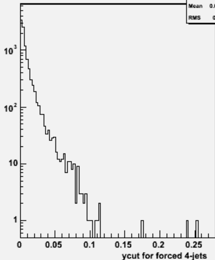
Ycut for 4-jets :w103514 ae1_n1n3e3uu_o
