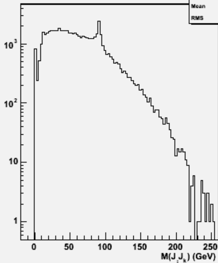
2jets mass(All comb)w103514 ae1_n1n3e3uu_o
