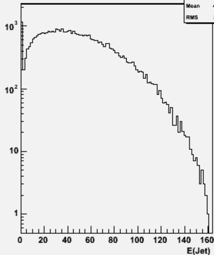
Jet energies(All jets)w103514 ae1_n1n3e3uu_o
