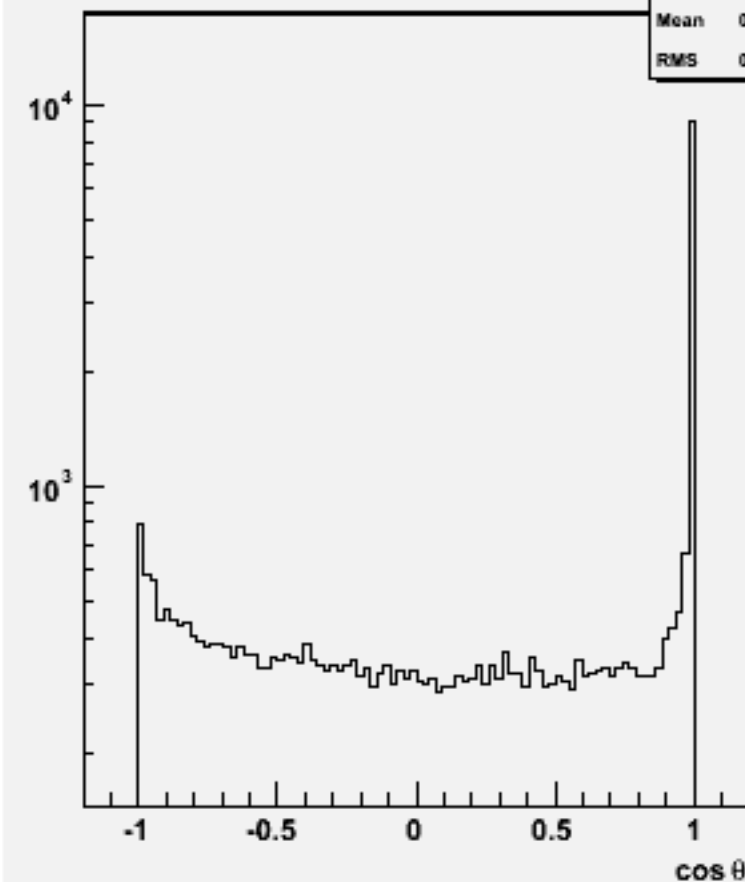
Jet cos \theta (All jets)w103514 ae1_n1n3e3uu_o
