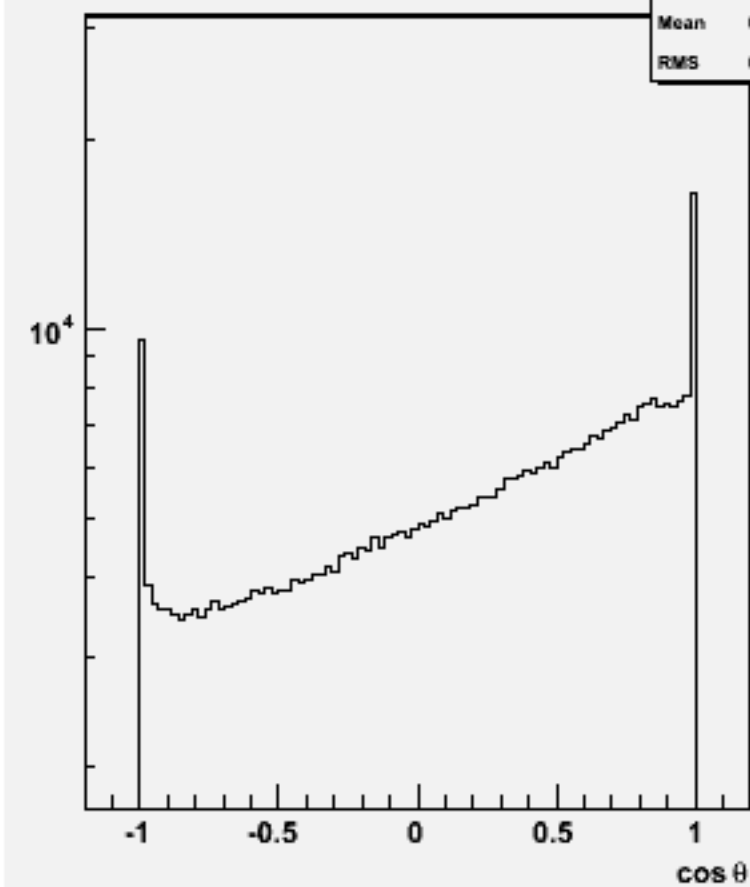
Particle cos \theta : w103498 ae1_n1udn3n3_o
