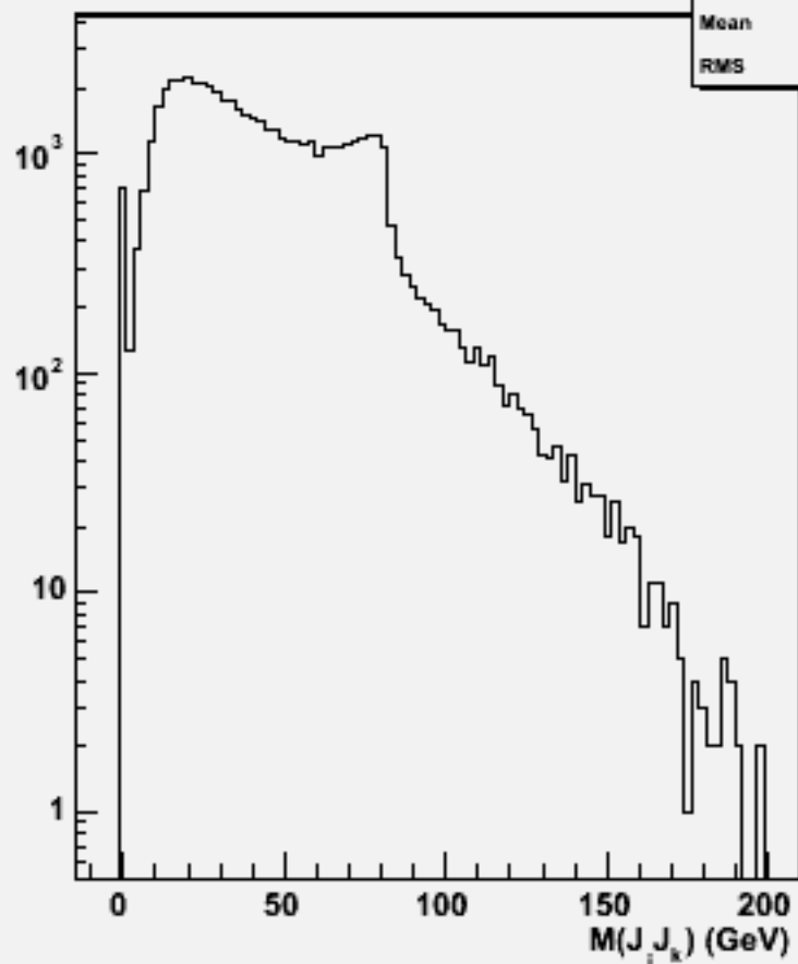
2jets mass(All comb)w103498 ae1_n1udn3n3_o
