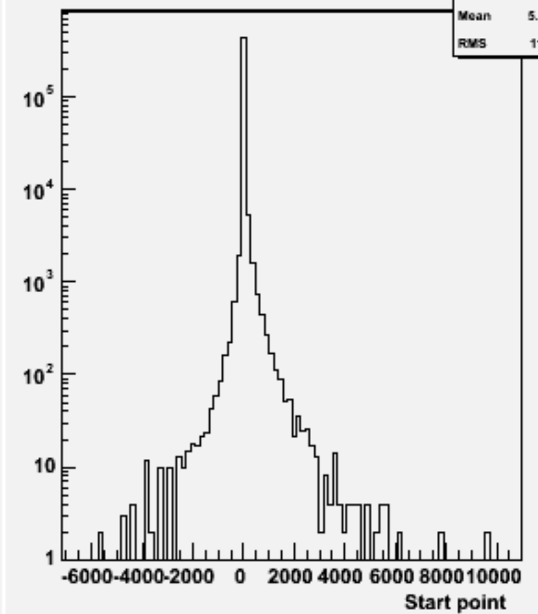
Start point Z : w103498 ae1_n1udn3n3_o
