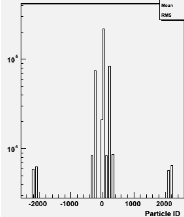
Particle ID : w103498 ae1_n1udn3n3_o
