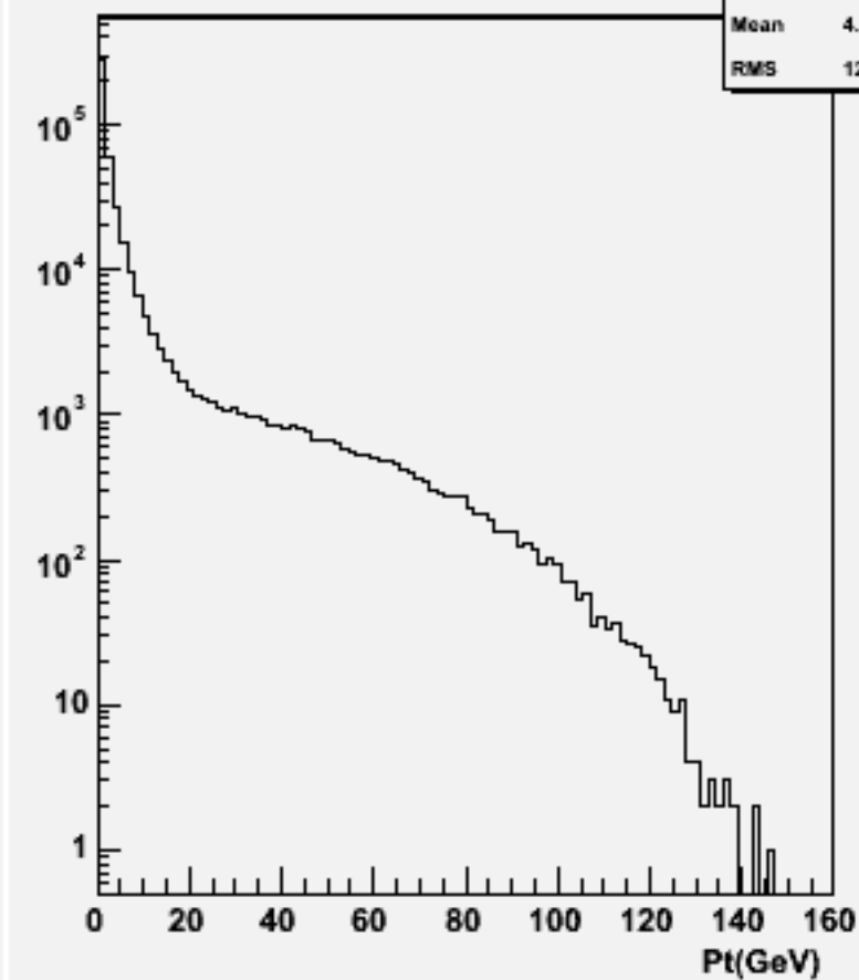
Particle Pt : w103498 ae1_n1udn3n3_o
