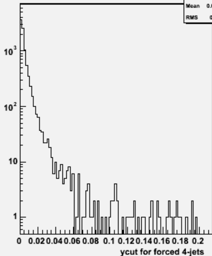
Ycut for 4-jets :w103498 ae1_n1udn3n3_o
