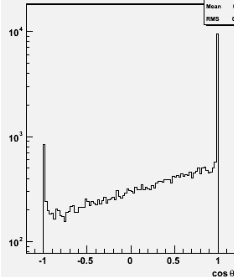
Jet cos \theta (All jets)w103498 ae1_n1udn3n3_o
