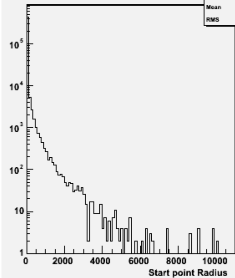
Start point R : w103498 ae1_n1udn3n3_o
