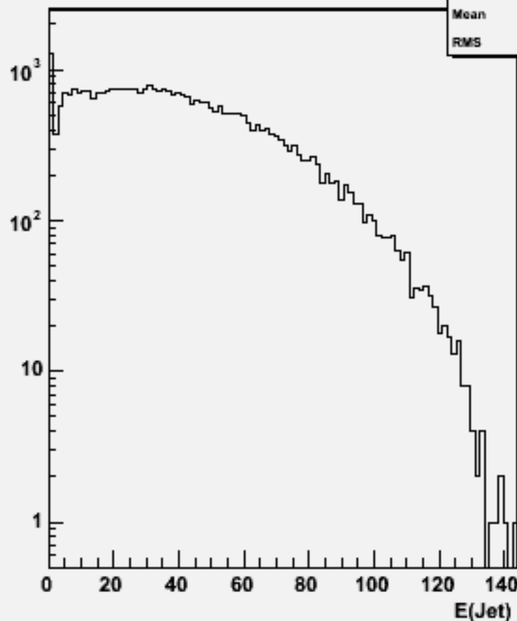
Jet energies(All jets)w103498 ae1_n1udn3n3_o
