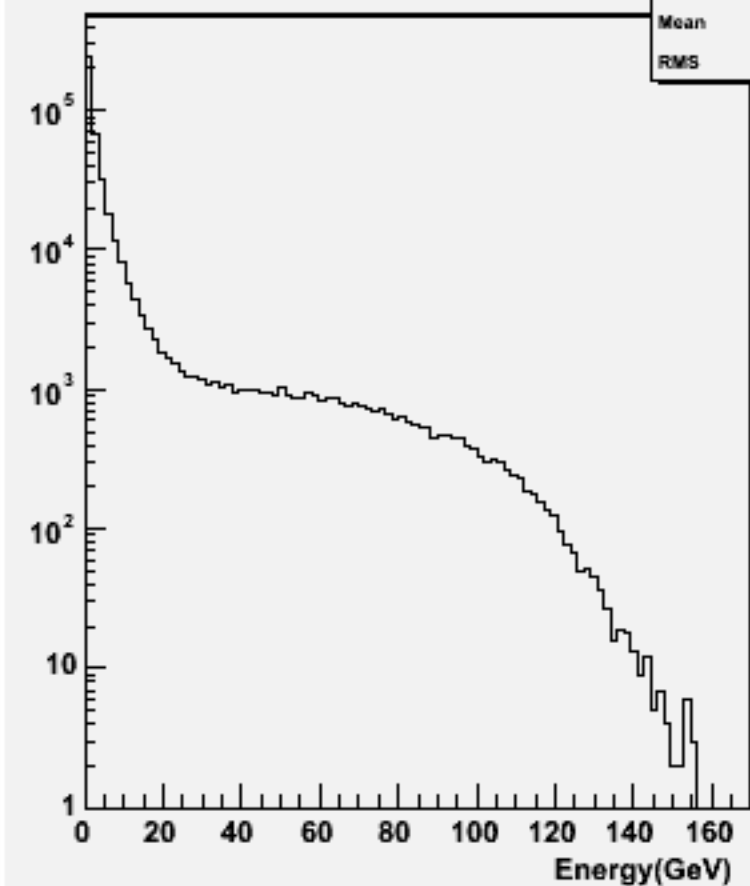
Particle Energy : w103498 ae1_n1udn3n3_o
