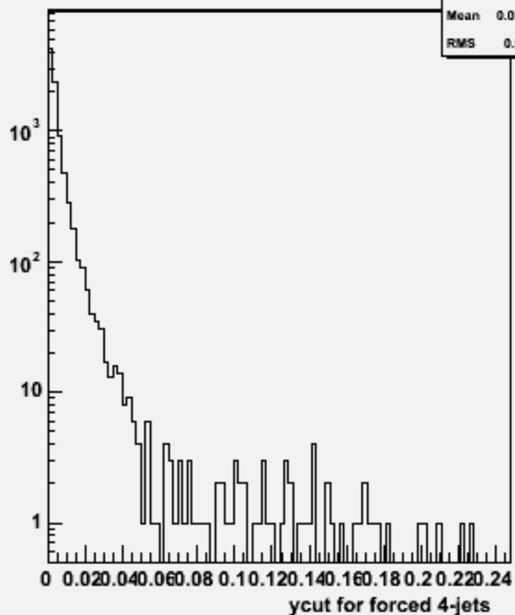
Ycut for 4-jets :w103482 ae1_n1csn2n2_o
