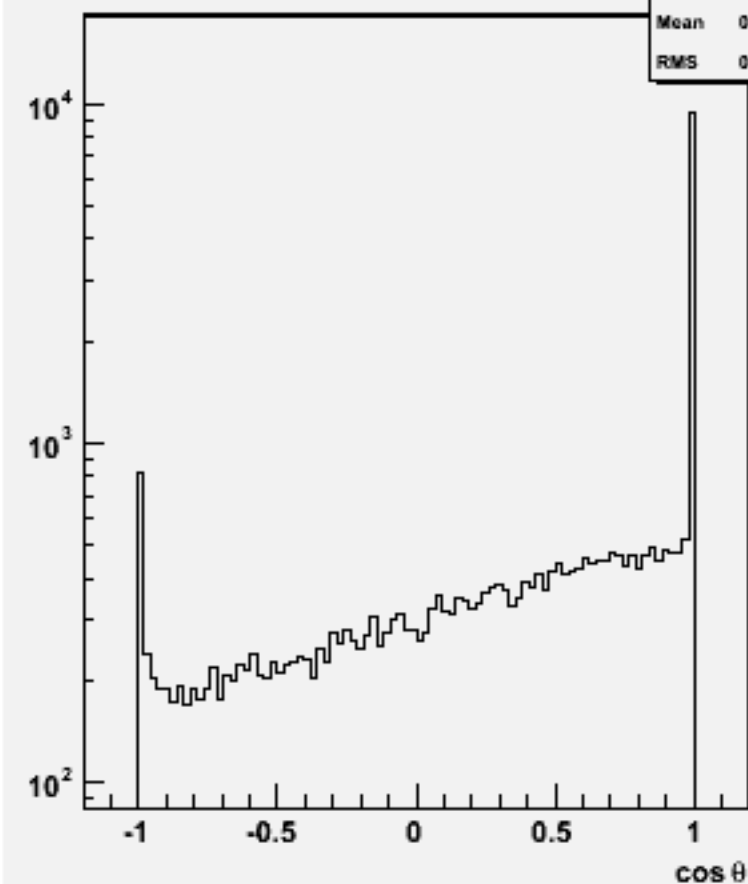
Jet cos \theta (All jets)w103482 ae1_n1csn2n2_o
