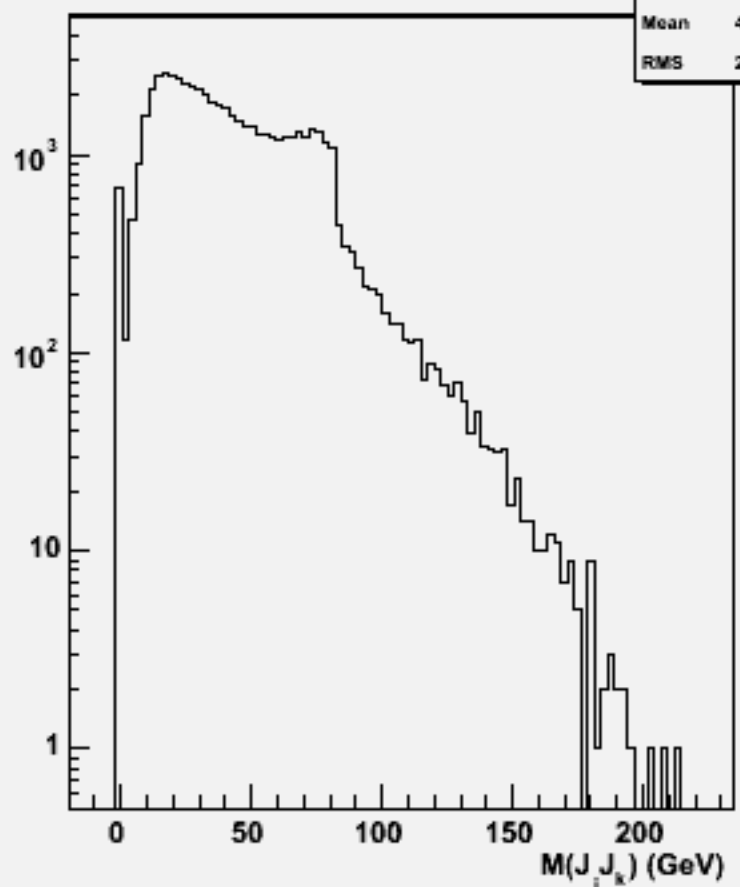
2jets mass(All comb)w103482 ae1_n1csn2n2_o
