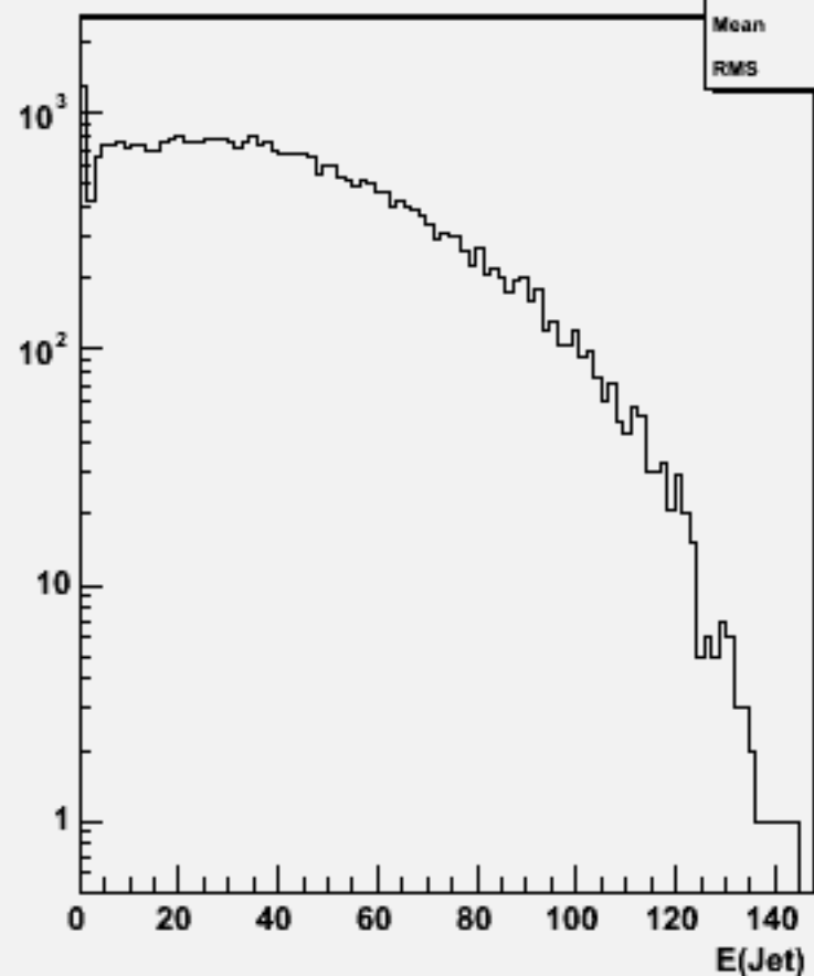
Jet energies(All jets)w103482 ae1_n1csn2n2_o
