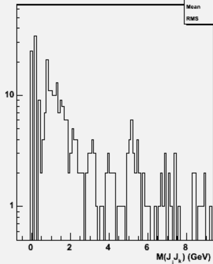
2jets mass(All comb)w103474 ae1_n1n3e3n2n2_o
