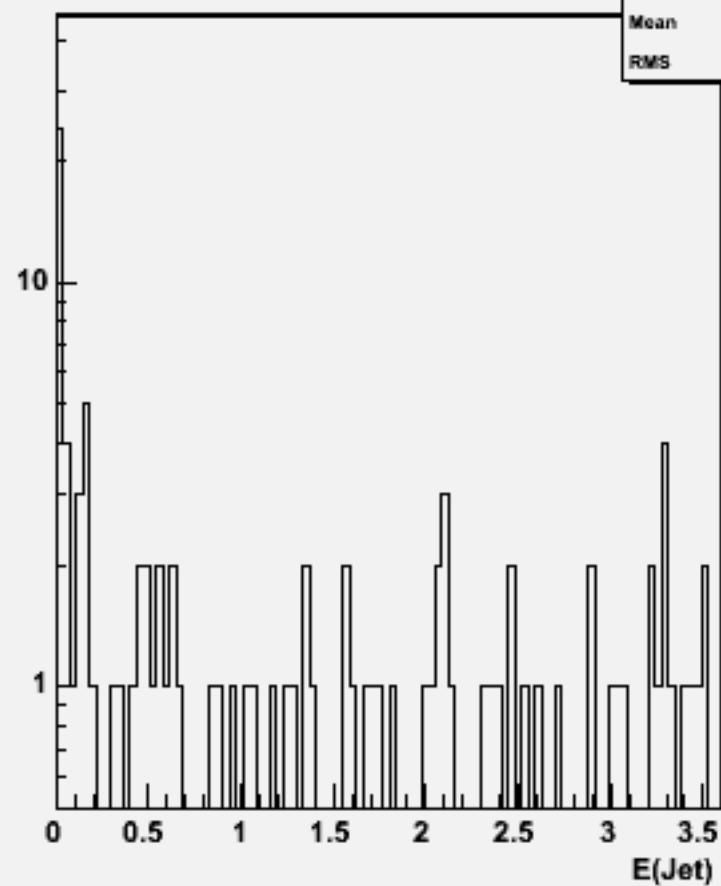
Jet energies(All jets)w103474 ae1_n1n3e3n2n2_o
