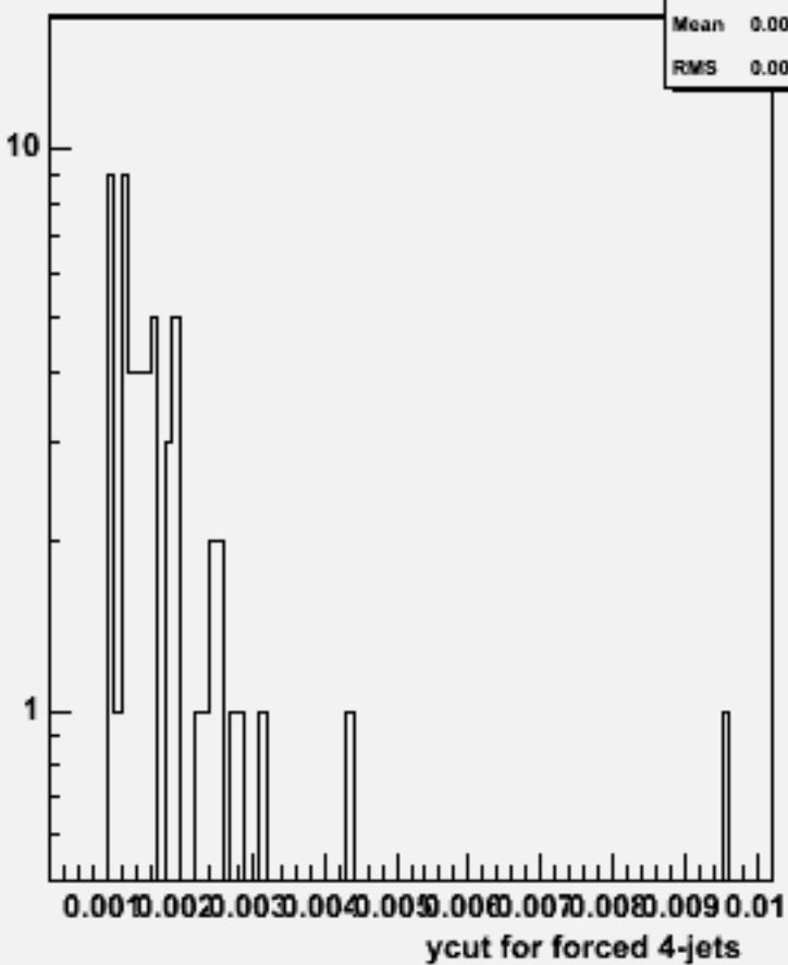
Ycut for 4-jets :w103474 ae1_n1n3e3n2n2_o
