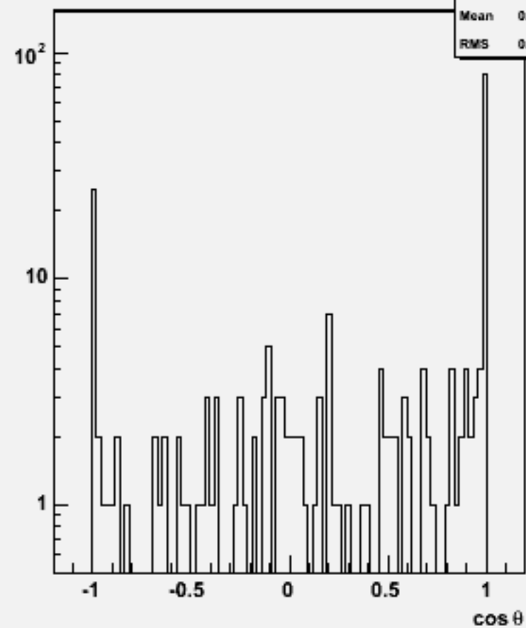
Jet cos \theta (All jets)w103474 ae1_n1n3e3n2n2_o
