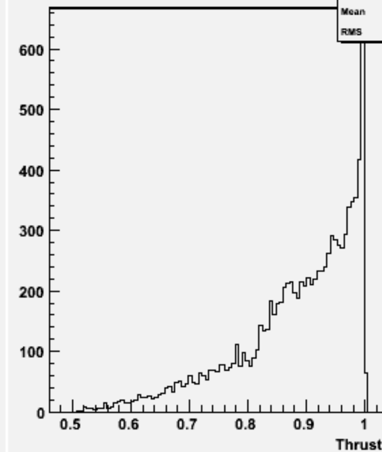
Thrust w103466 ae1_n1n1e1n2n2_o
