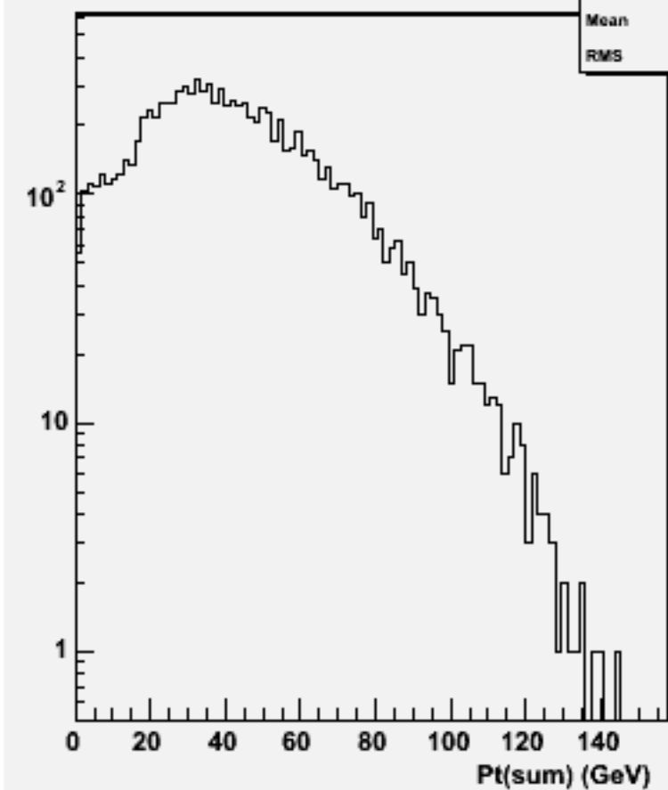
Pt Sum: w103466 ae1_n1n1e1n2n2_o
