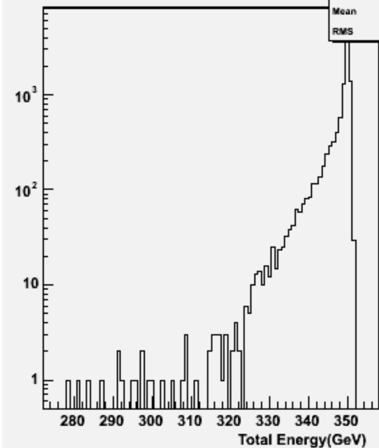
Total Energy (inc. \nu ): w103466 ae1_n1n1e1n2n2_o
