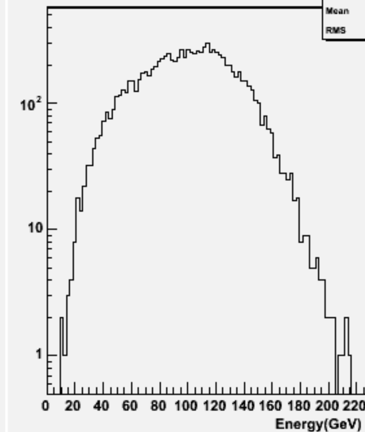
Total Energy (w/o \nu ): w103466 ae1_n1n1e1n2n2_o
