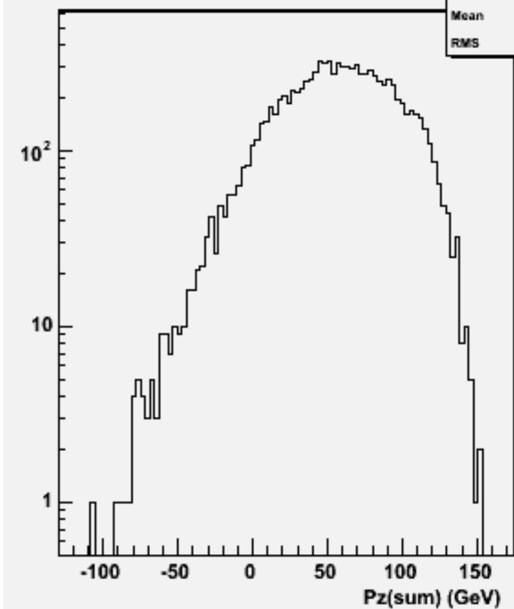
Pz Sum: w103466 ae1_n1n1e1n2n2_o
