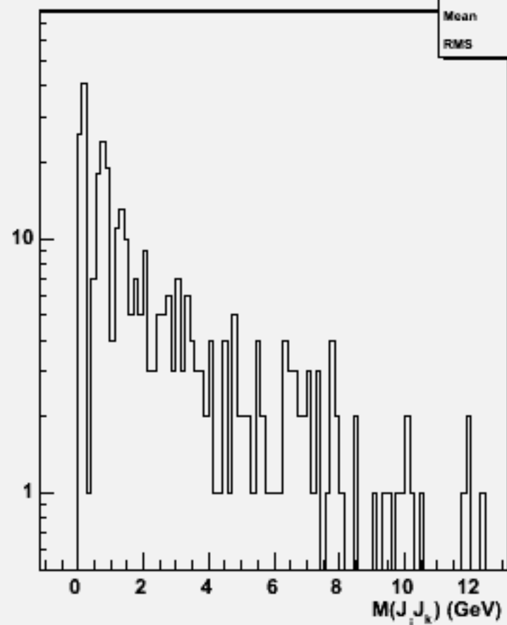
2jets mass(All comb)w103454 ae1_n1n3e3n1n1_o
