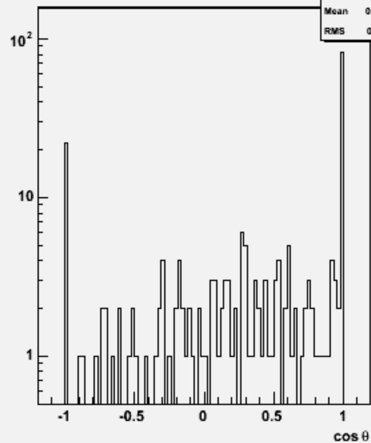
Jet cos \theta (All jets)w103454 ae1_n1n3e3n1n1_o
