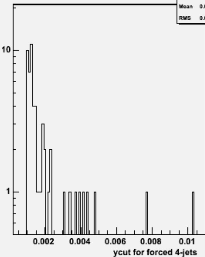
Ycut for 4-jets :w103454 ae1_n1n3e3n1n1_o
