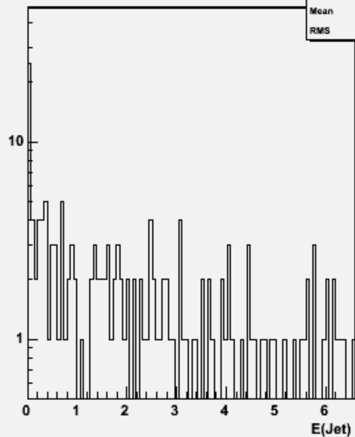
Jet energies(All jets)w103454 ae1_n1n3e3n1n1_o
