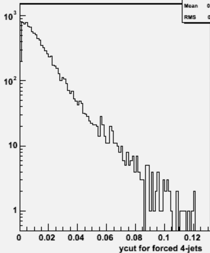
Ycut for 4-jets :w103432 e1a_e1bbbb_o
