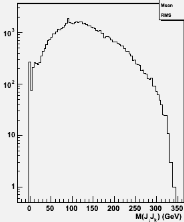
2jets mass(All comb)w103428 e1a_e1ssbb_o
