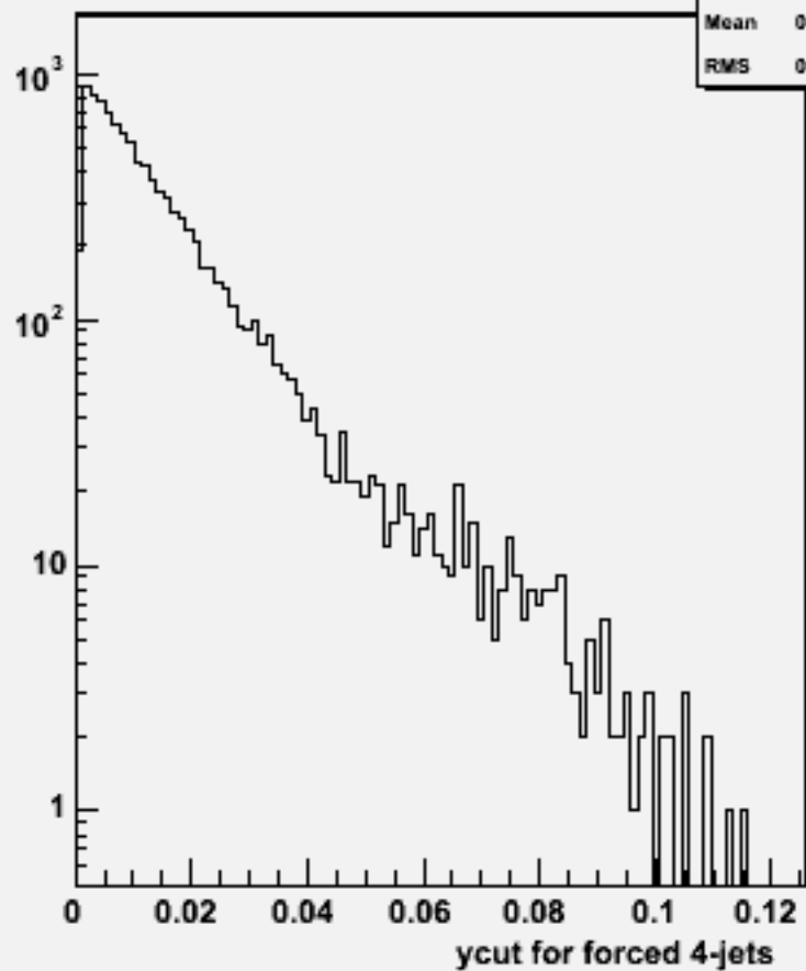
Ycut for 4-jets :w103428 e1a_e1ssbb_o
