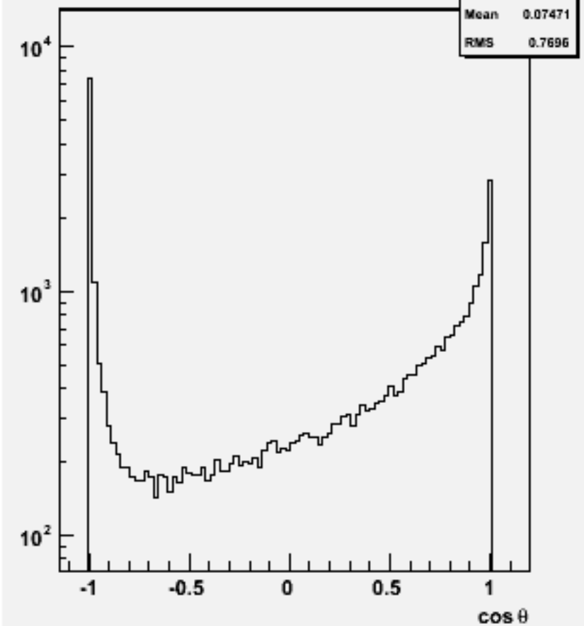
Jet cos \theta (All jets)w103428 e1a_e1ssbb_o
