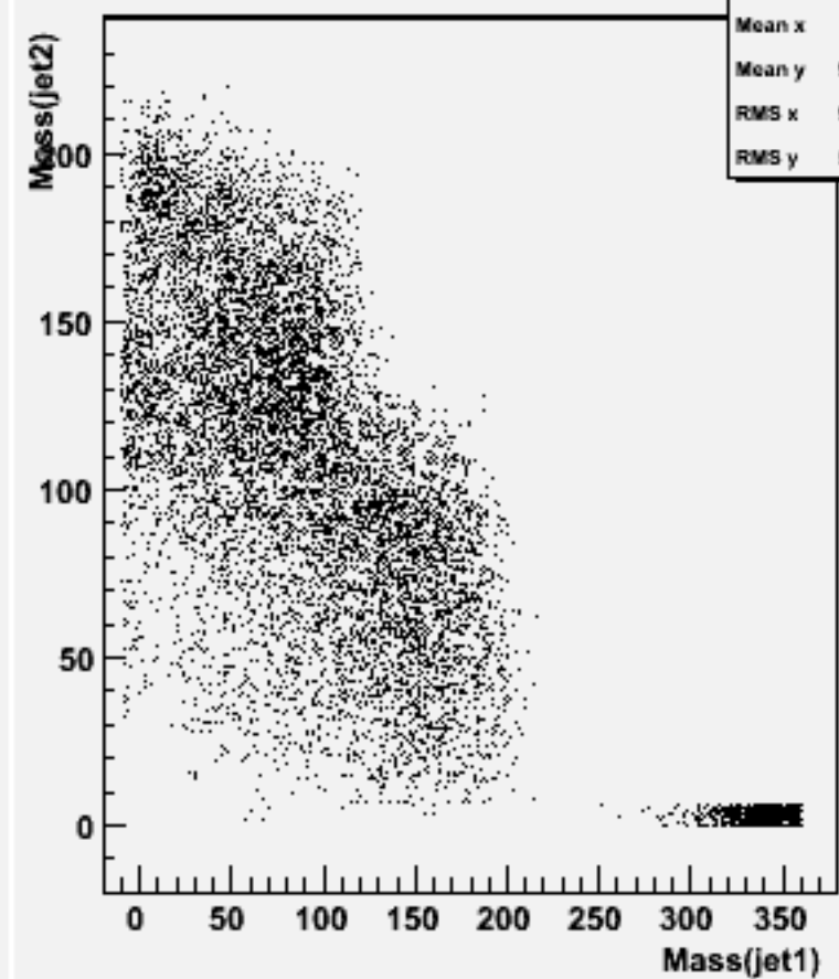
Jet mass for forced 2-jets : w103426 e1a_e1ssbb_o
