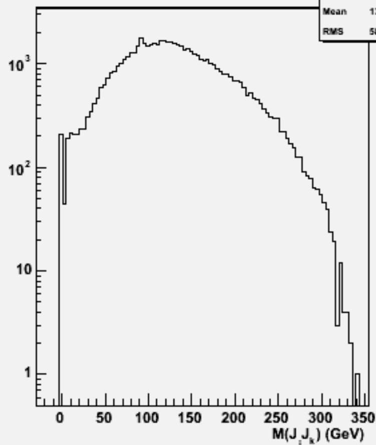
2jets mass(All comb)w103426 e1a_e1ssbb_o
