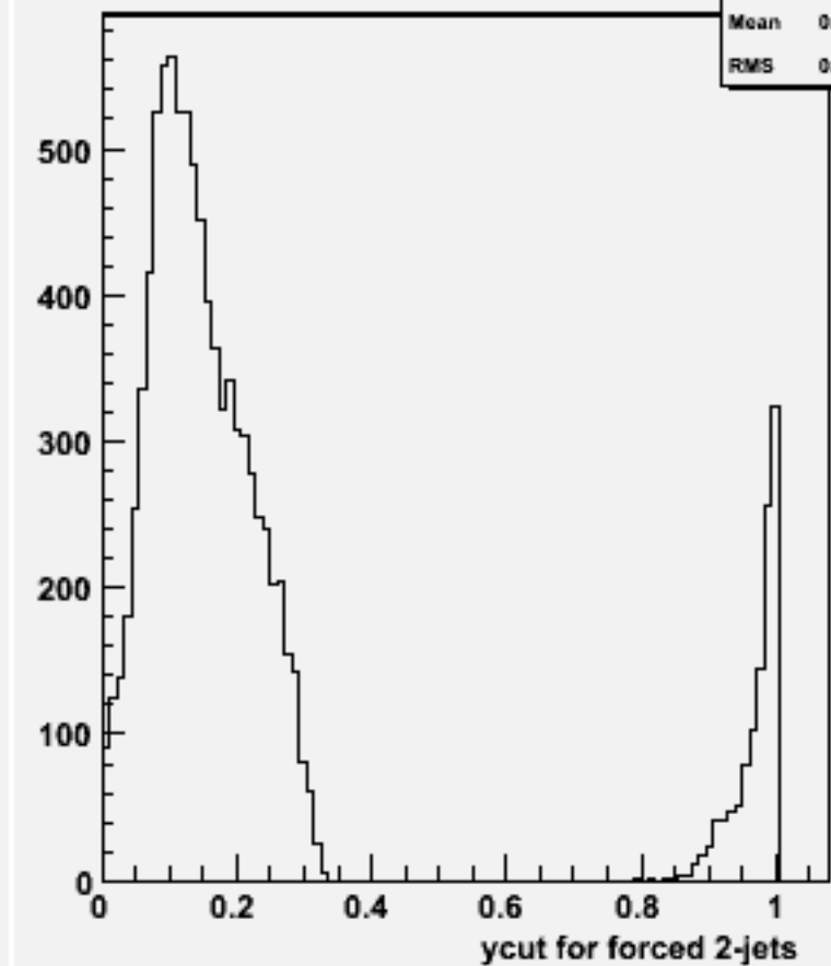
Ycut for 2-jets :w103426 e1a_e1ssbb_o
