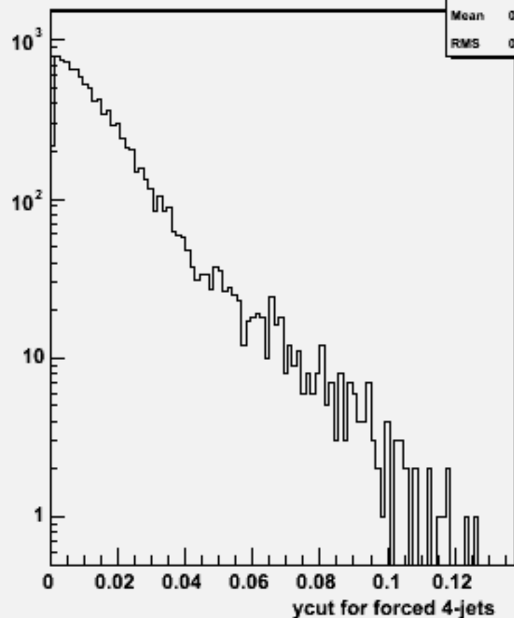
Ycut for 4-jets :w103426 e1a_e1ssbb_o
