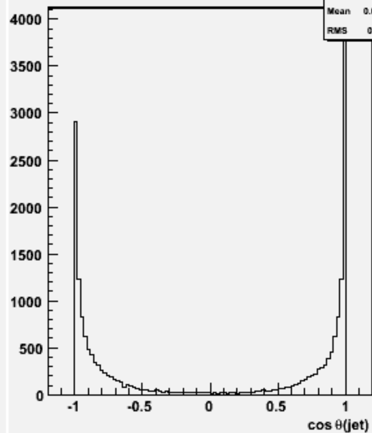
cos \theta for 2-jets :w103426 e1a_e1ssbb_o
