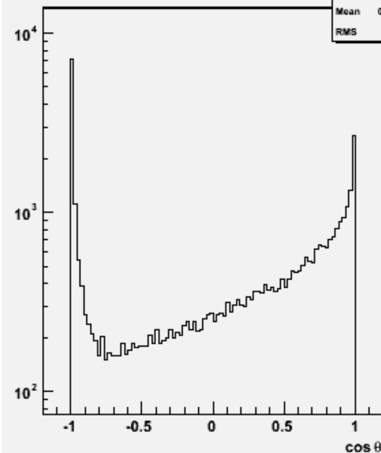
Jet cos \theta (All jets)w103426 e1a_e1ssbb_o
