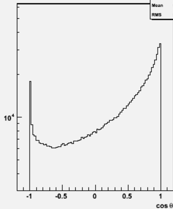
Particle cosθ : w103426 e1a_e1ssbb_o
