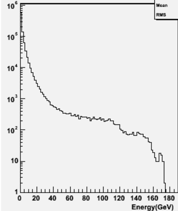
Particle Energy : w103426 e1a_e1ssbb_o
