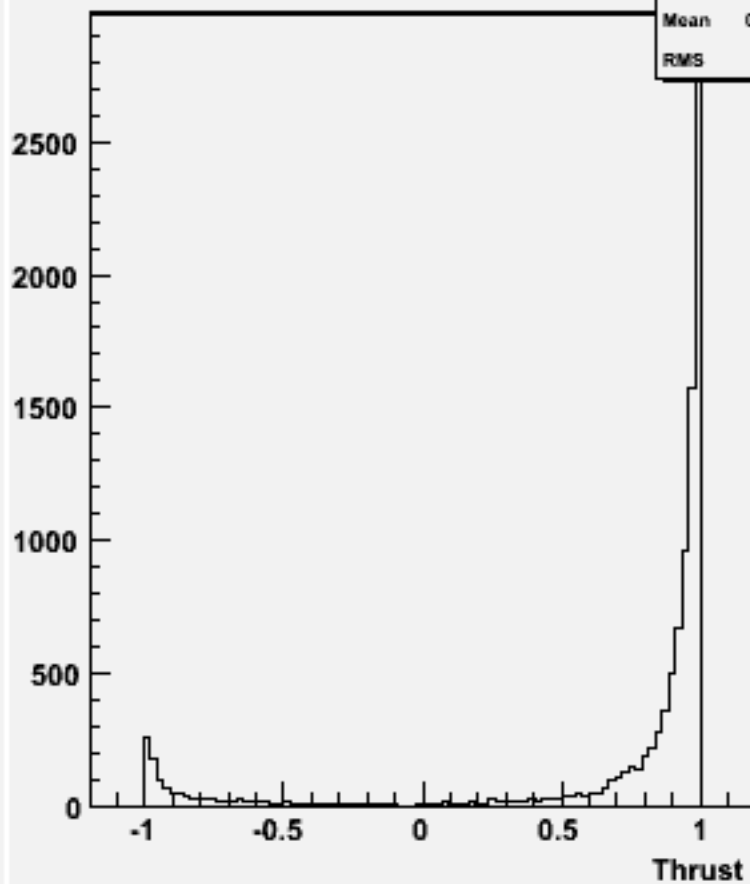
cos \Theta (thrust) w103426 e1a_e1ssbb_o
