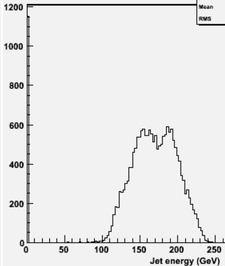
energy for 2-jets :w103426 e1a_e1ssbb_o
