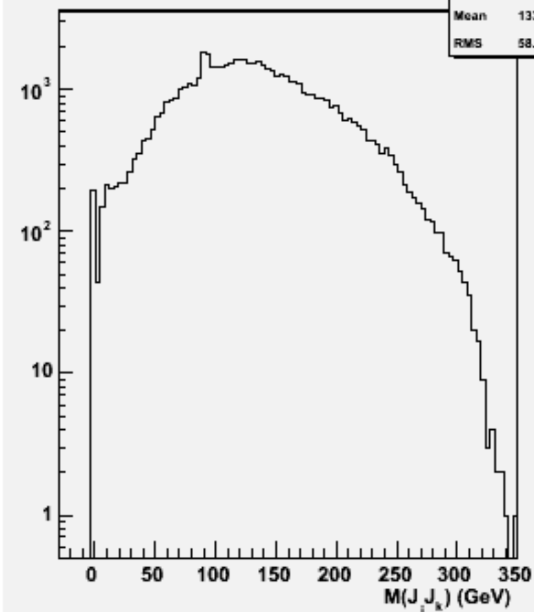
2jets mass(All comb)w103422 e1a_e1ssss_o
