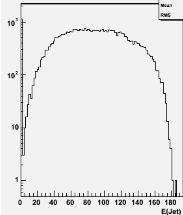
Jet energies(All jets)w103422 e1a_e1ssss_o
