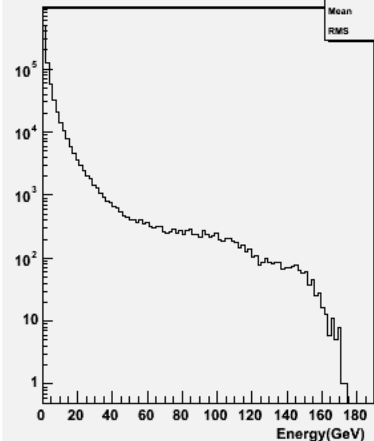
Particle Energy : w103422 e1a_e1ssss_o
