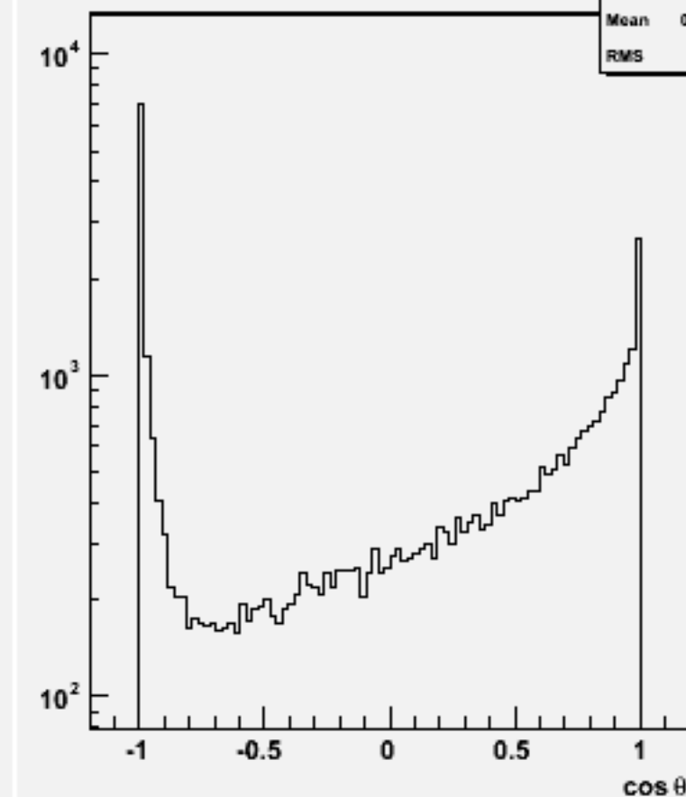
Jet cos \theta (All jets)w103422 e1a_e1ssss_o
