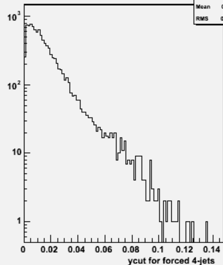
Ycut for 4-jets :w103422 e1a_e1ssss_o
