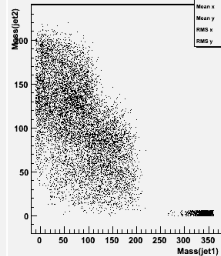
Jet mass for forced 2-jets : w103420 e1a_e1ddb_o
