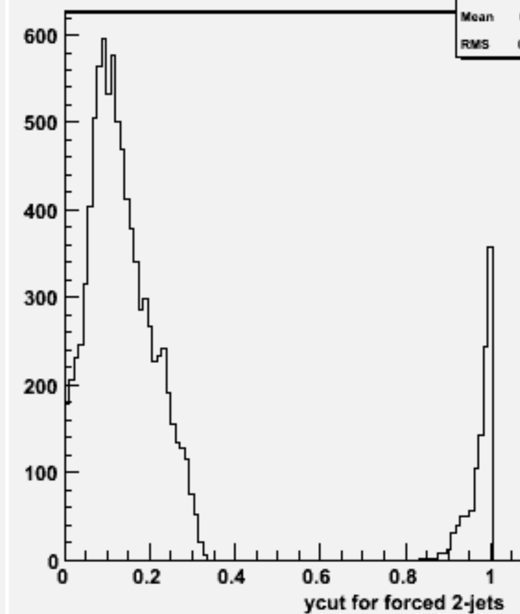
Ycut for 2-jets :w103420 e1a_e1ddb_o
