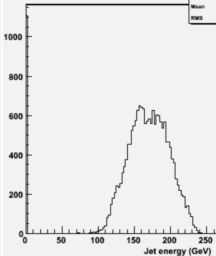
energy for 2-jets :w103420 e1a_e1ddb_o
