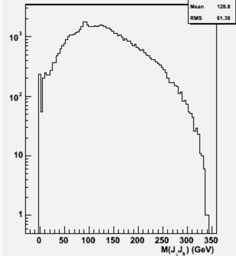
2jets mass(All comb)w103420 e1a_e1ddb_o
