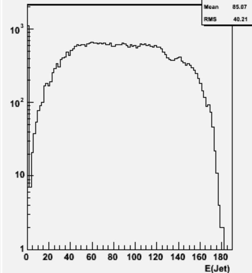
Jet energies(All jets)w103420 e1a_e1ddb_o
