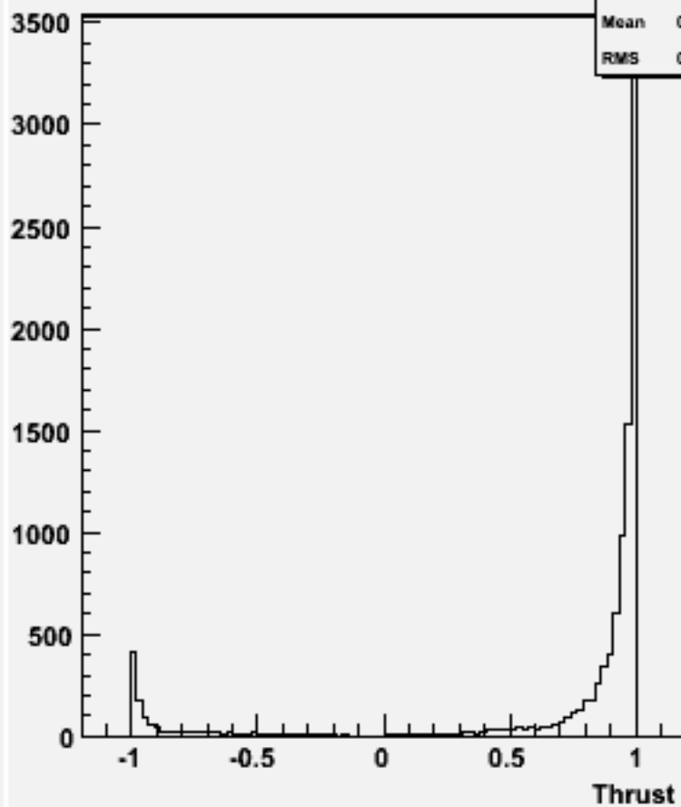
cos \Theta (thrust) w103420 e1a_e1ddb_o
