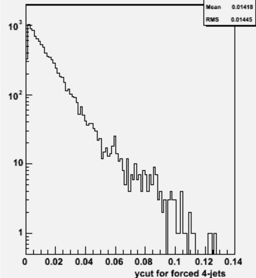
Ycut for 4-jets :w103420 e1a_e1ddb_o
