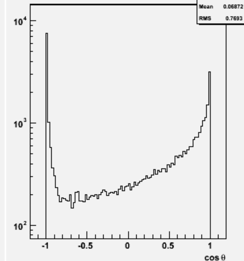
Jet cos \theta (All jets)w103420 e1a_e1ddb_o
