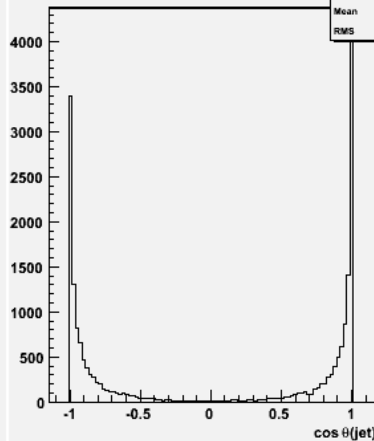
cos \theta for 2-jets :w103420 e1a_e1ddb_o
