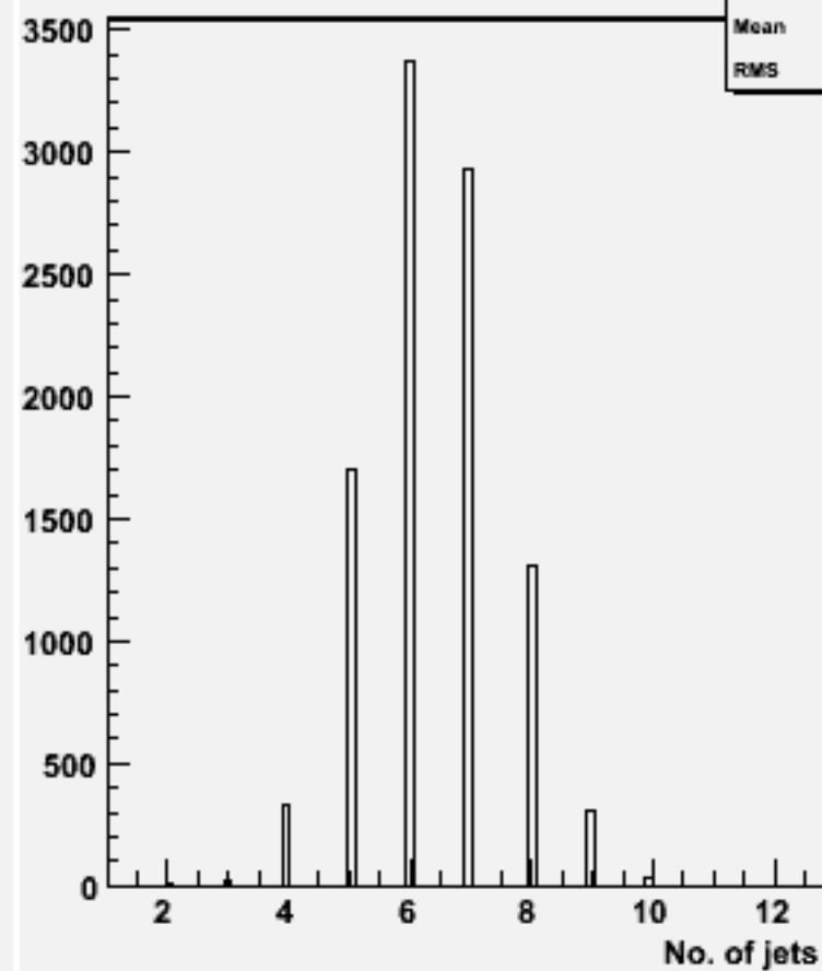
No. jets (ycut=0.001) : w103420 e1a_e1ddb_o
