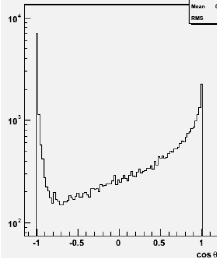
Jet cos \theta (All jets)w103418 e1a_e1ddb_o
