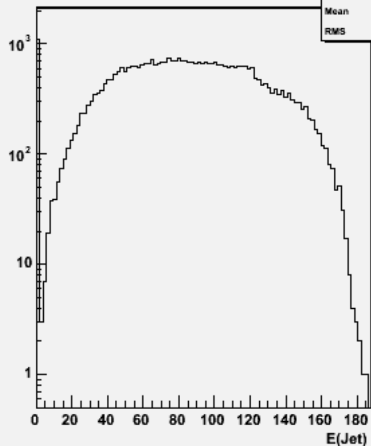
Jet energies(All jets)w103418 e1a_e1ddb_o
