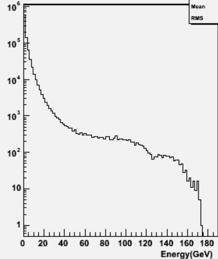
Particle Energy : w103418 e1a_e1ddbb_o
