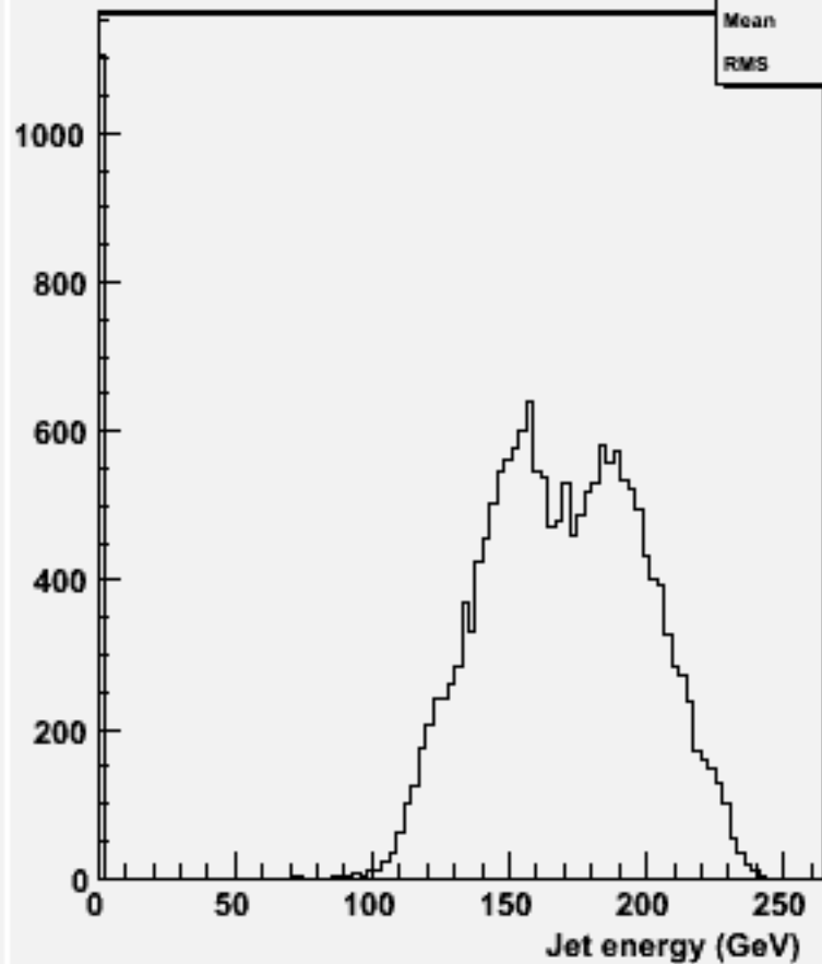
energy for 2-jets :w103418 e1a_e1ddb_o
