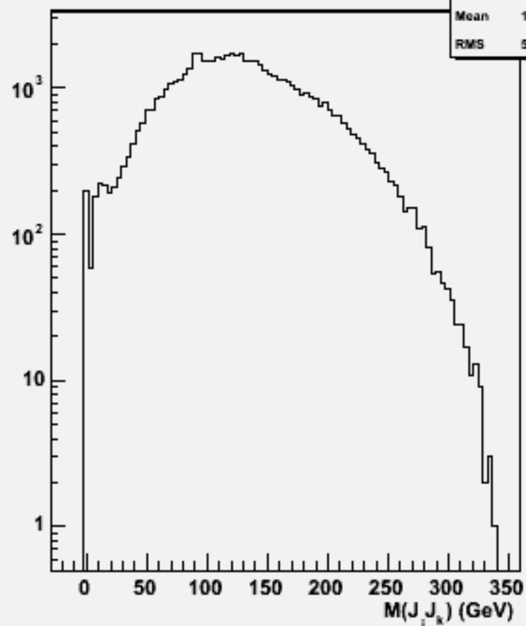
2jets mass(All comb)w103418 e1a_e1ddb_o
