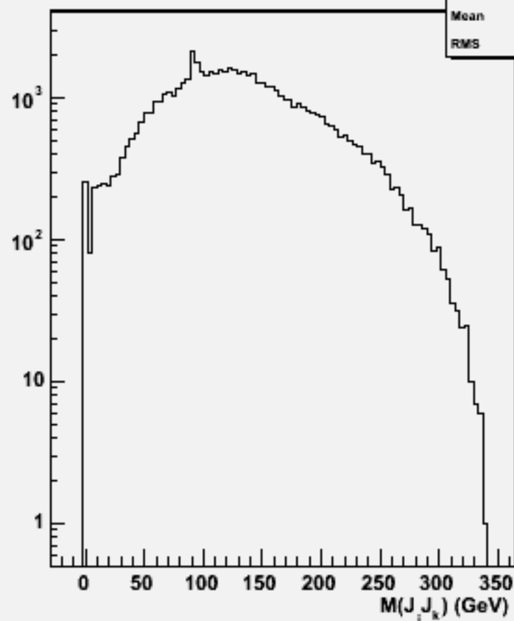
2jets mass(All comb)w103416 e1a_e1ddss_o
