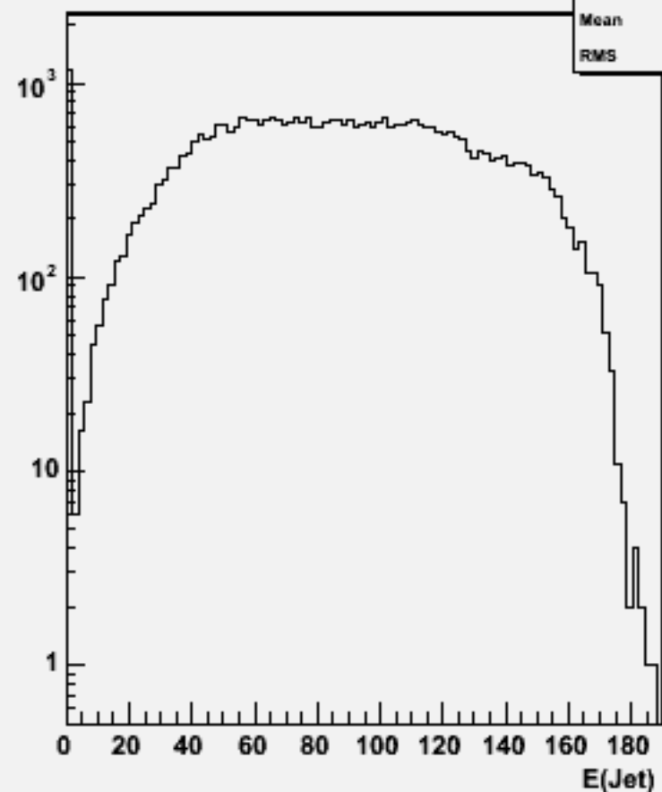
Jet energies(All jets)w103416 e1a_e1ddss_o
