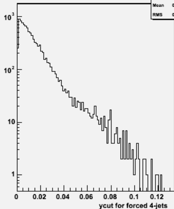
Ycut for 4-jets :w103416 e1a_e1ddss_o
