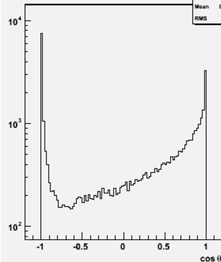
Jet cos \theta (All jets)w103416 e1a_e1ddss_o
