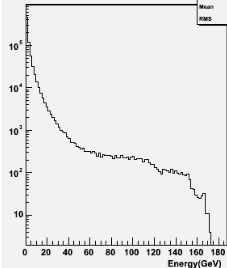
Particle Energy : w103416 e1a_e1ddss_o
