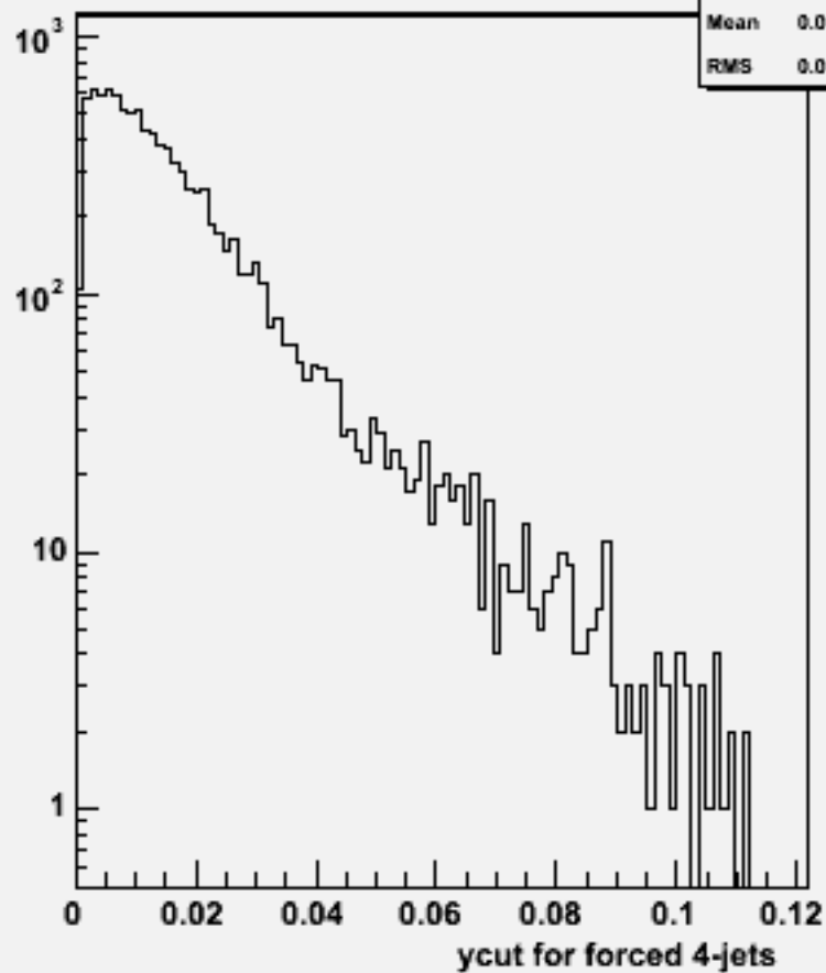
Ycut for 4-jets :w103414 e1a_e1dddss_o
