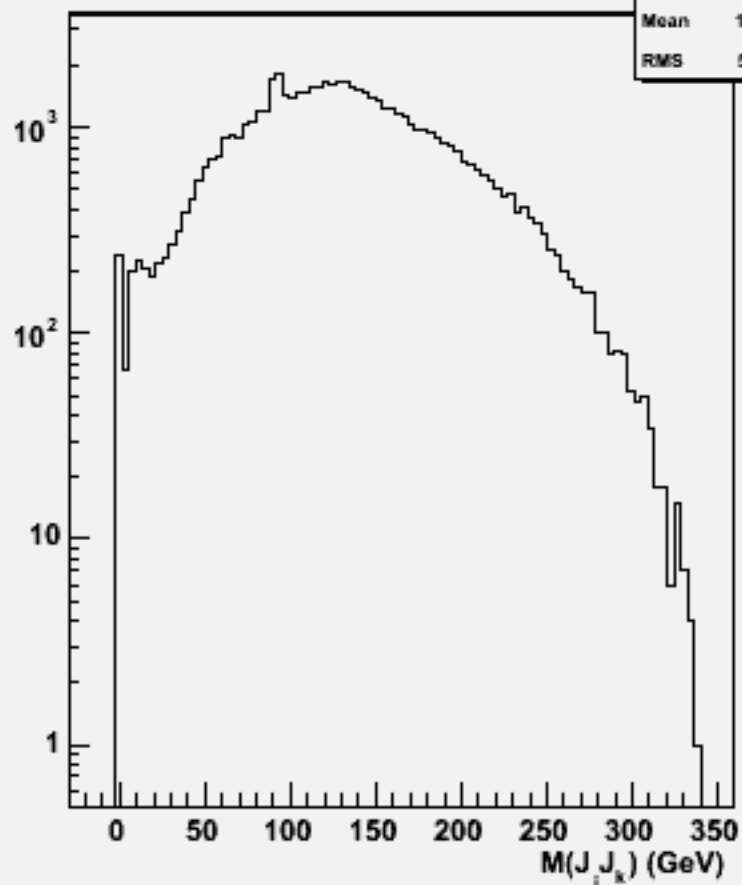
2jets mass(All comb)w103414 e1a_e1dddss_o
