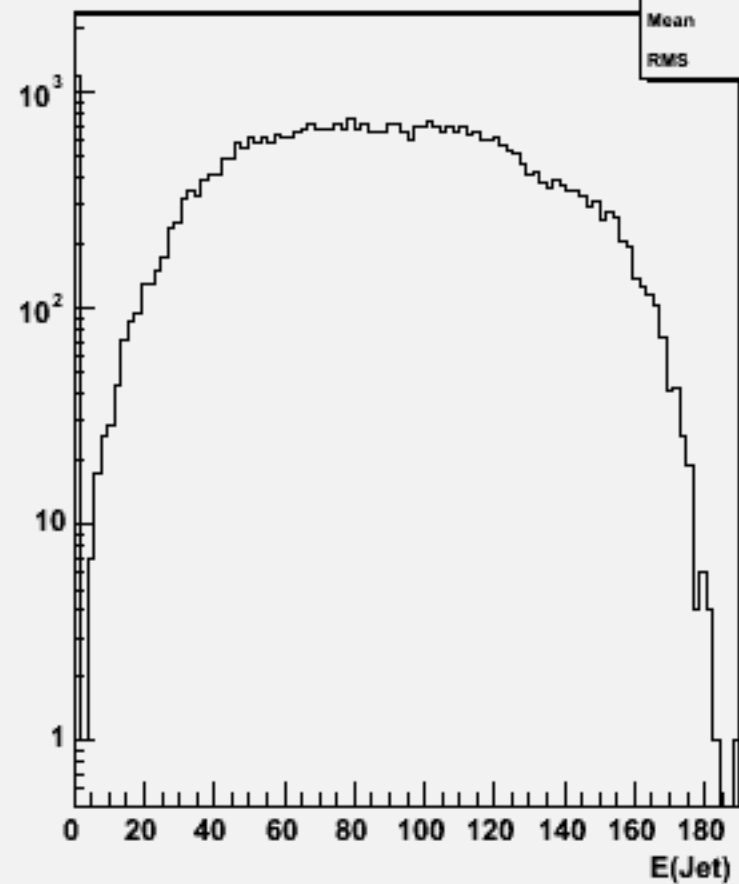
Jet energies(All jets)w103414 e1a_e1dddss_o
