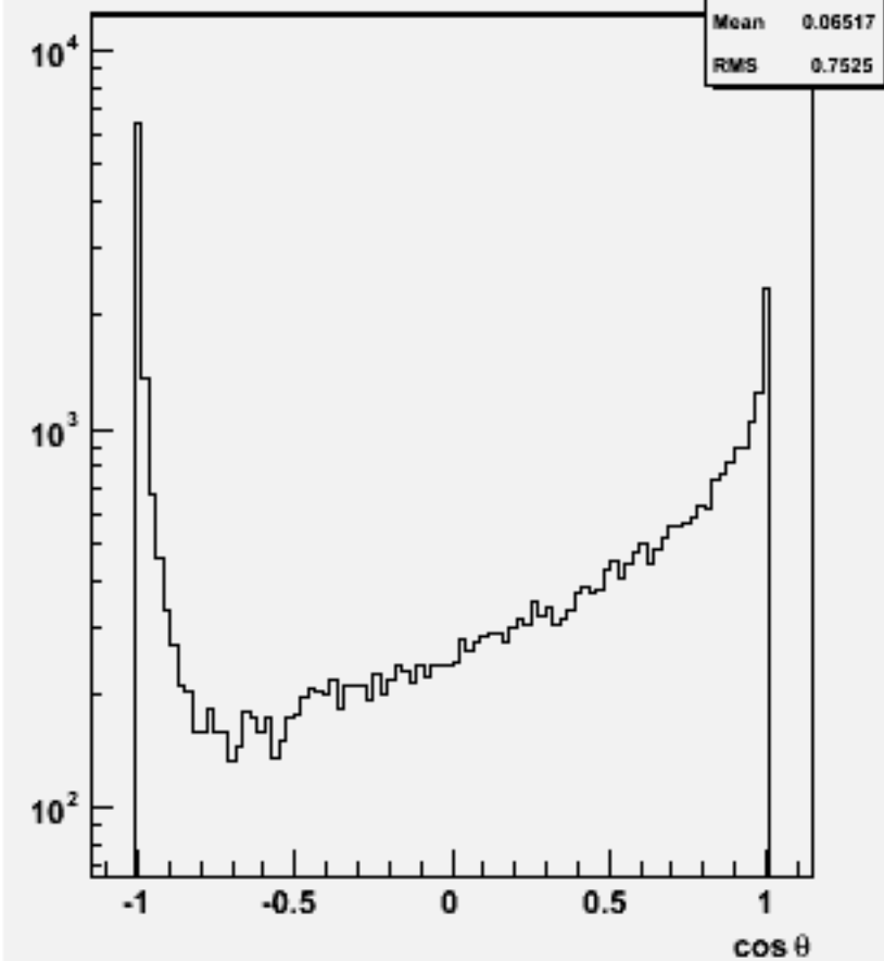
Jet cos \theta (All jets)w103414 e1a_e1dddss_o
