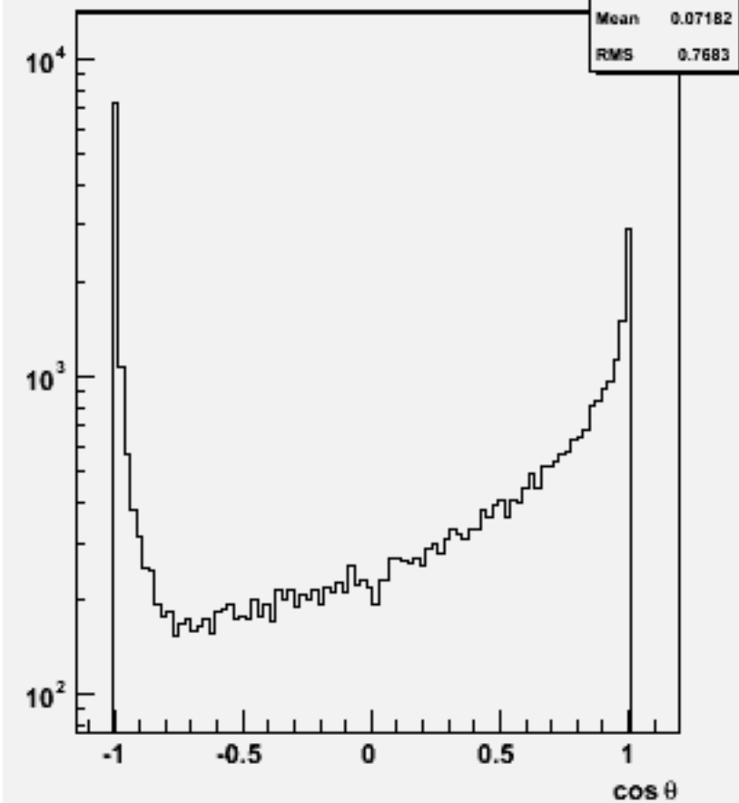
Jet cos \theta (All jets)w103412 e1a_e1dddd_o
