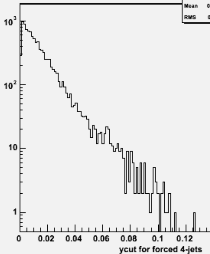
Ycut for 4-jets :w103412 e1a_e1dddd_o
