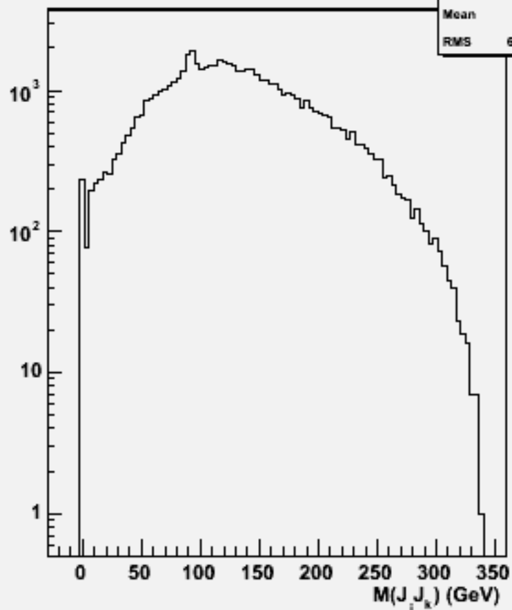
2jets mass(All comb)w103412 e1a_e1dddd_o
