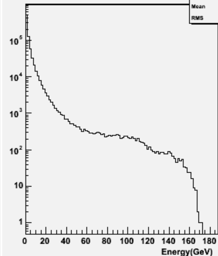
Particle Energy : w103410 e1a_e1dddd_o
