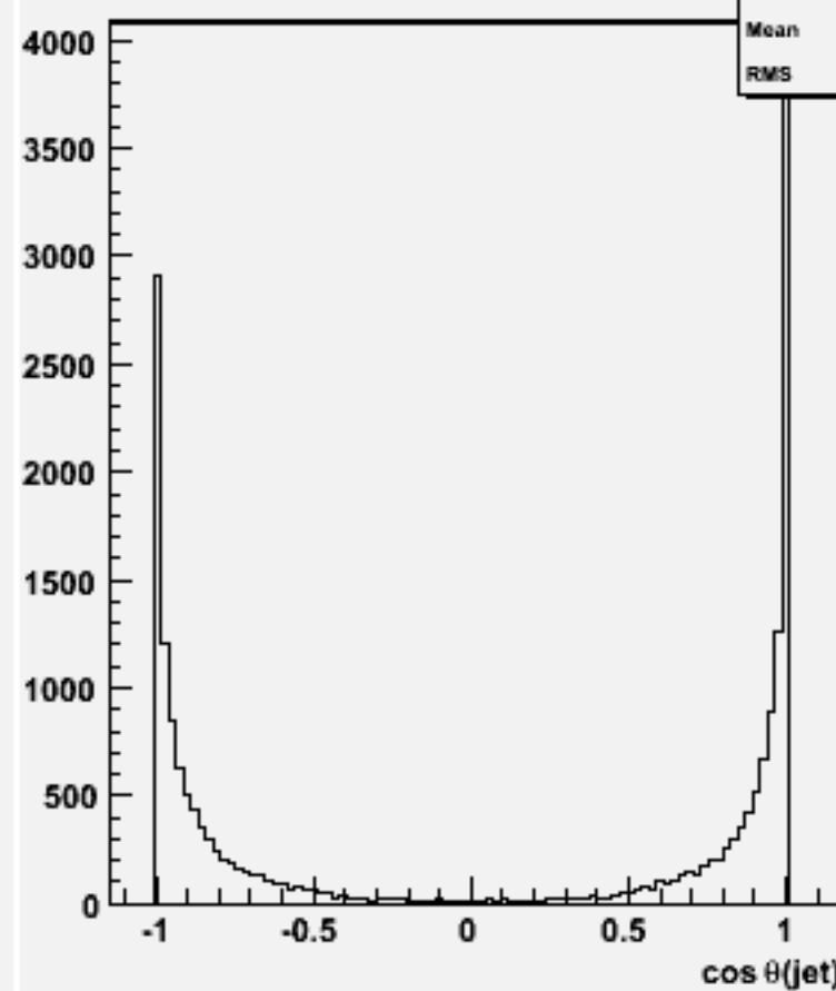
cos \theta for 2-jets :w103410 e1a_e1dddd_o
