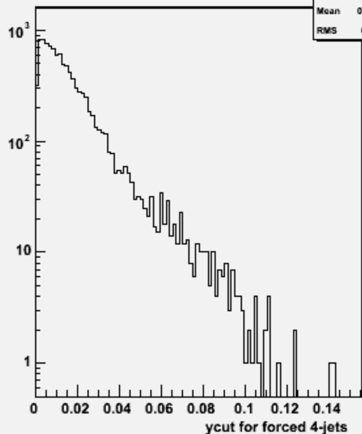
Ycut for 4-jets :w103410 e1a_e1dddd_o
