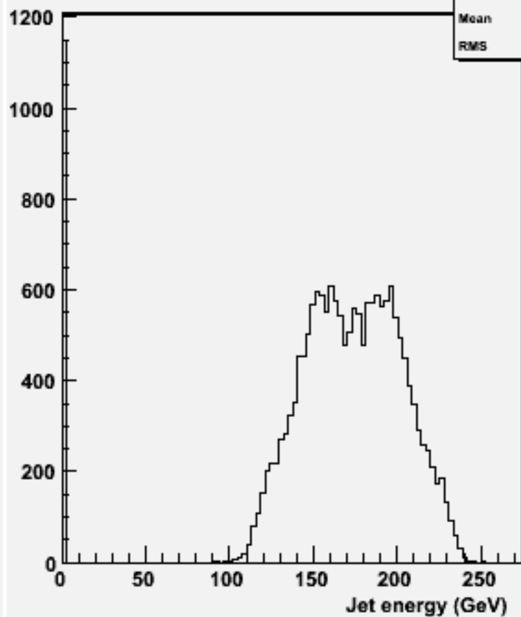
energy for 2-jets :w103410 e1a_e1dddd_o
