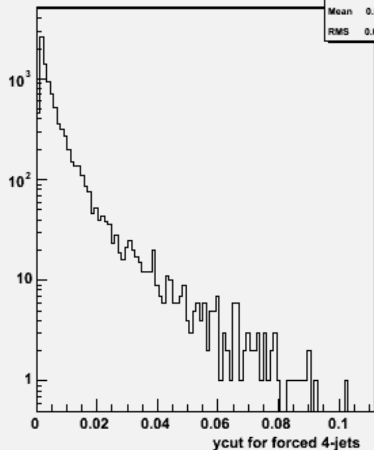
Ycut for 4-jets :w103408 e1a_e1e3e3bb_o
