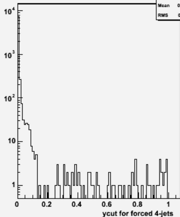
Ycut for 4-jets :w103405 e1a_e1e3e3ss_o
